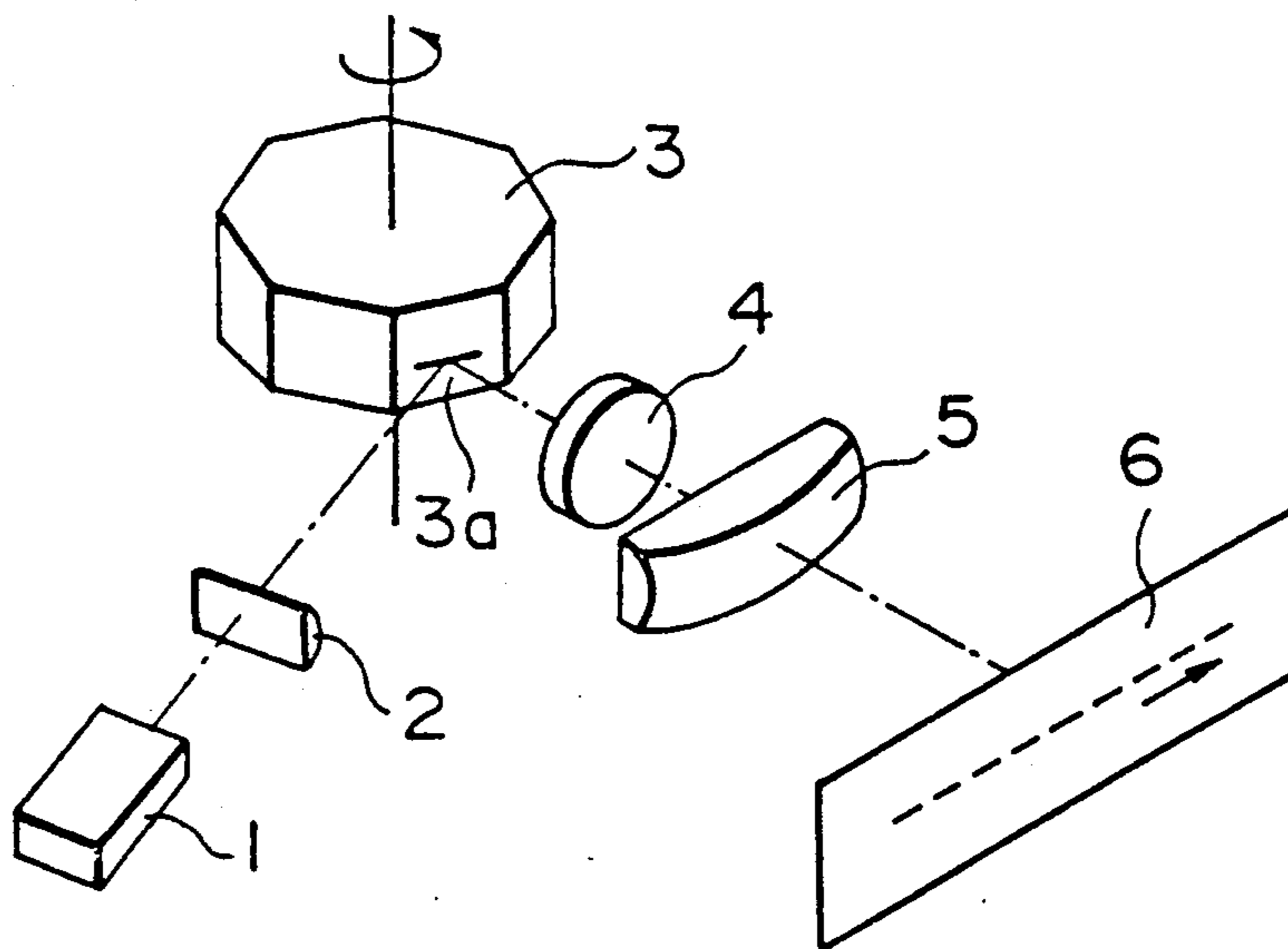
FIG. 2 PRIOR ART
