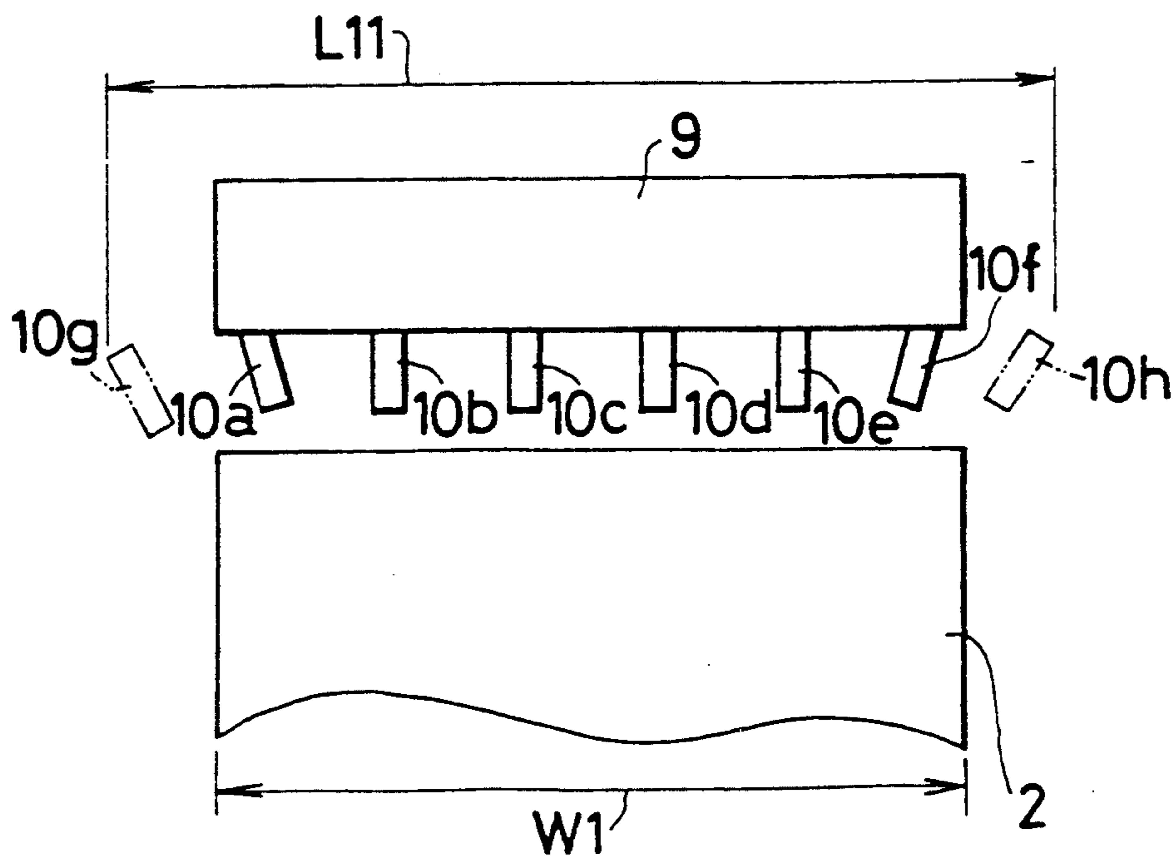
Fig. 2 Prior Art
