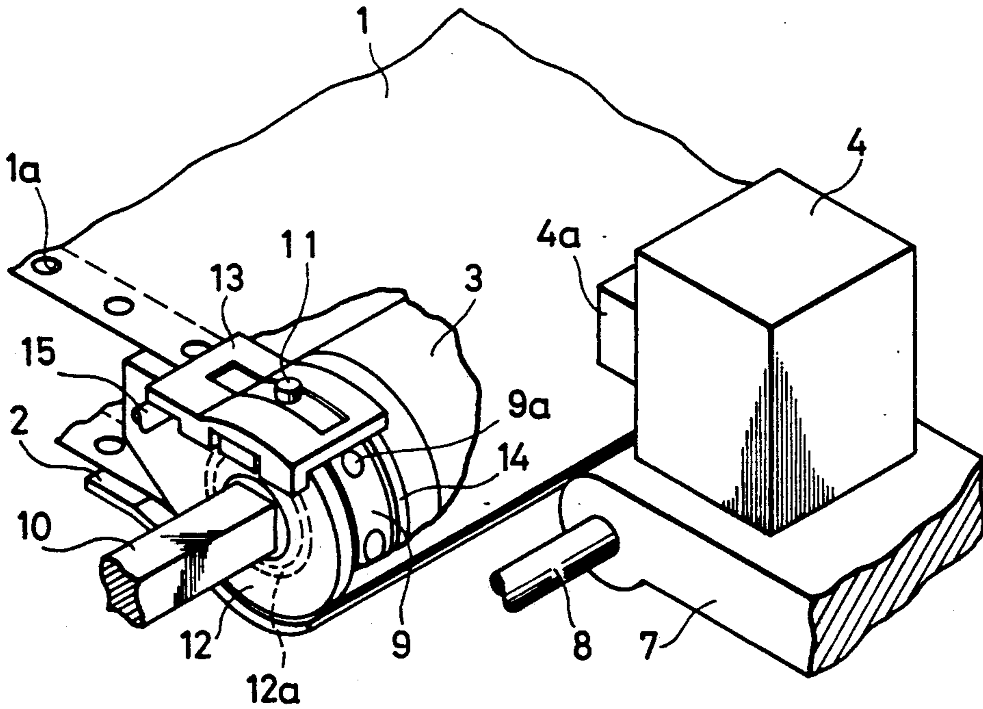
FIG. 4 (PRIOR ART)
