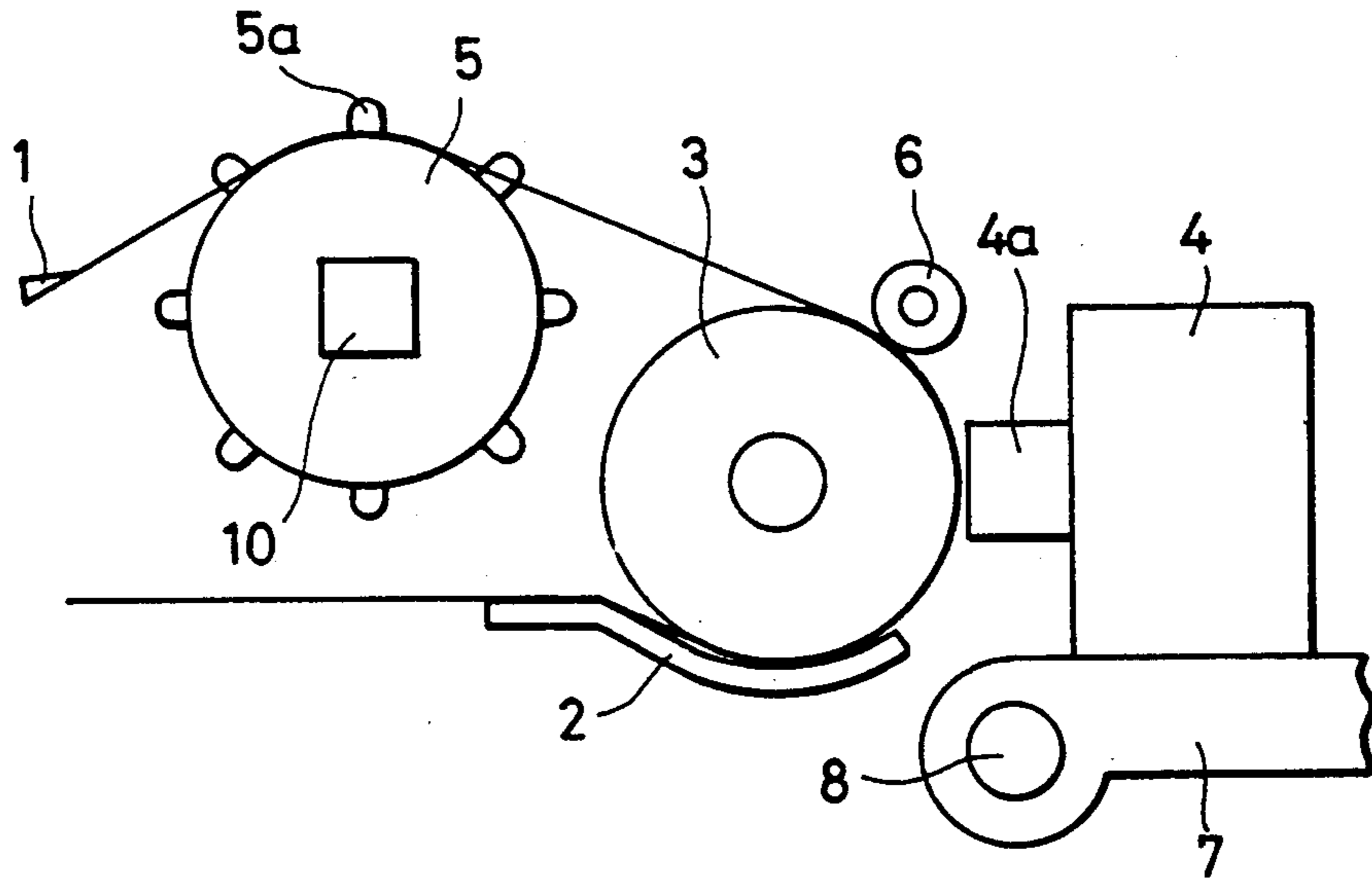
FIG. 1 (PRIOR ART)
