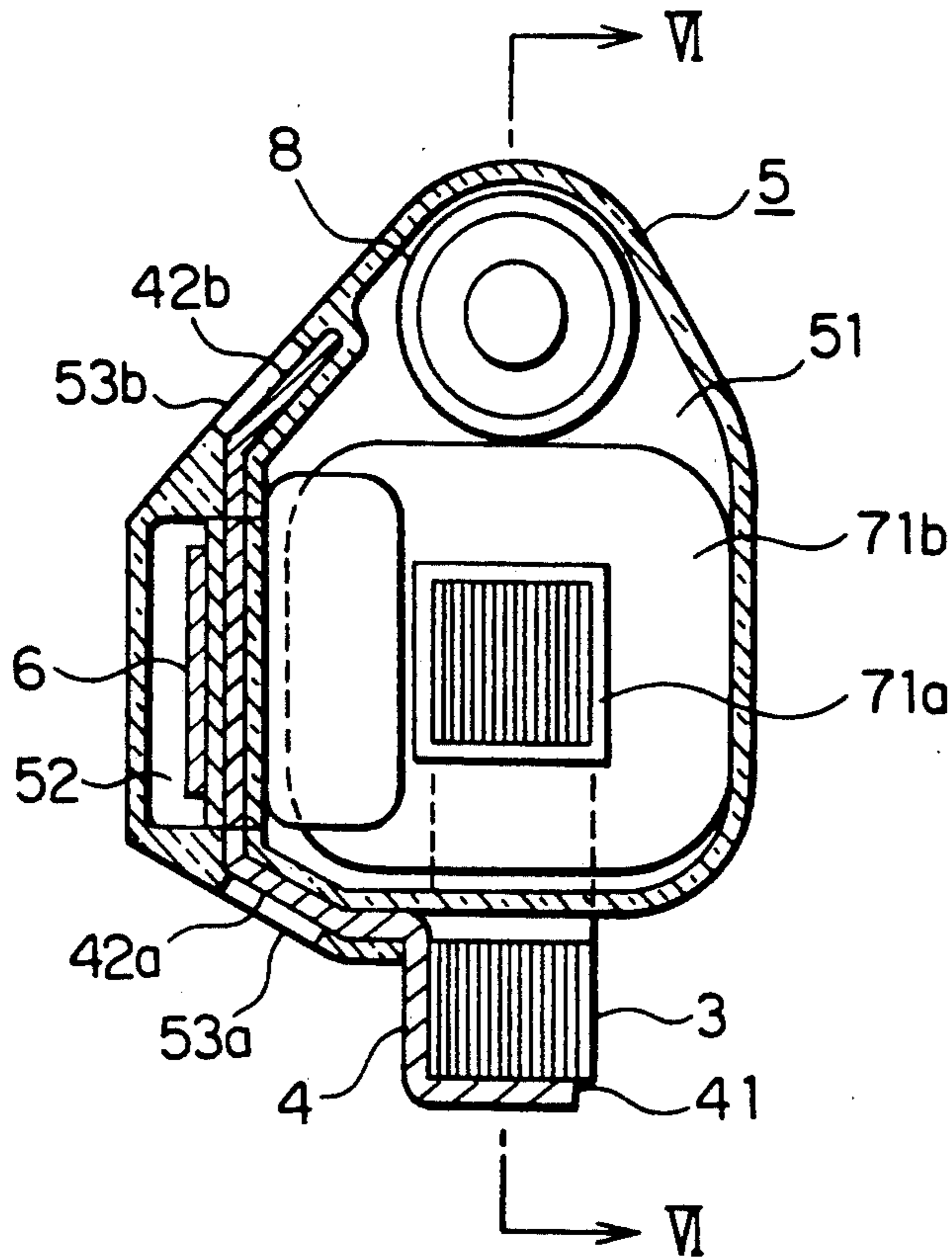
FIG. 5 PRIOR ART
