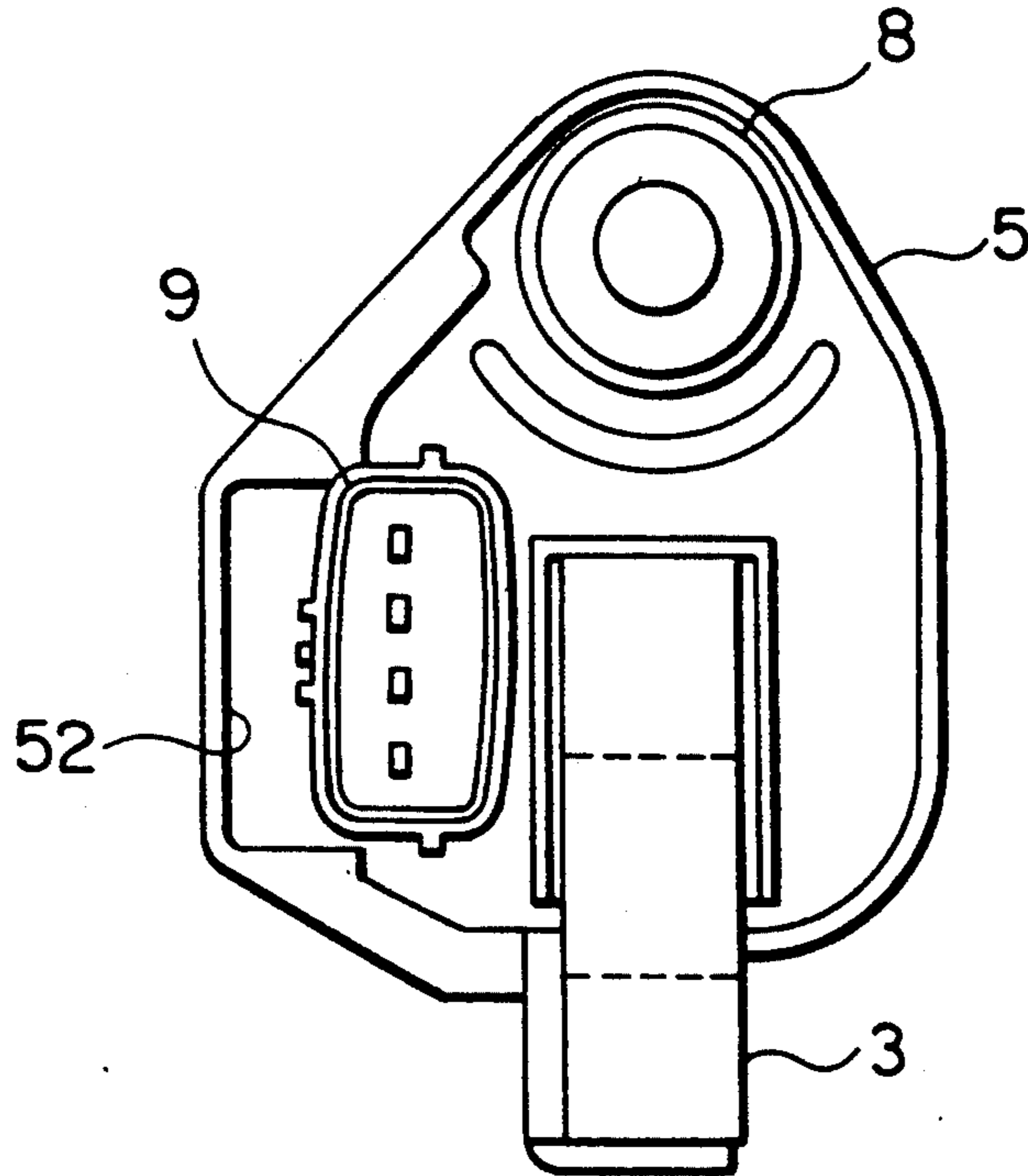
FIG. 8 PRIOR ART
