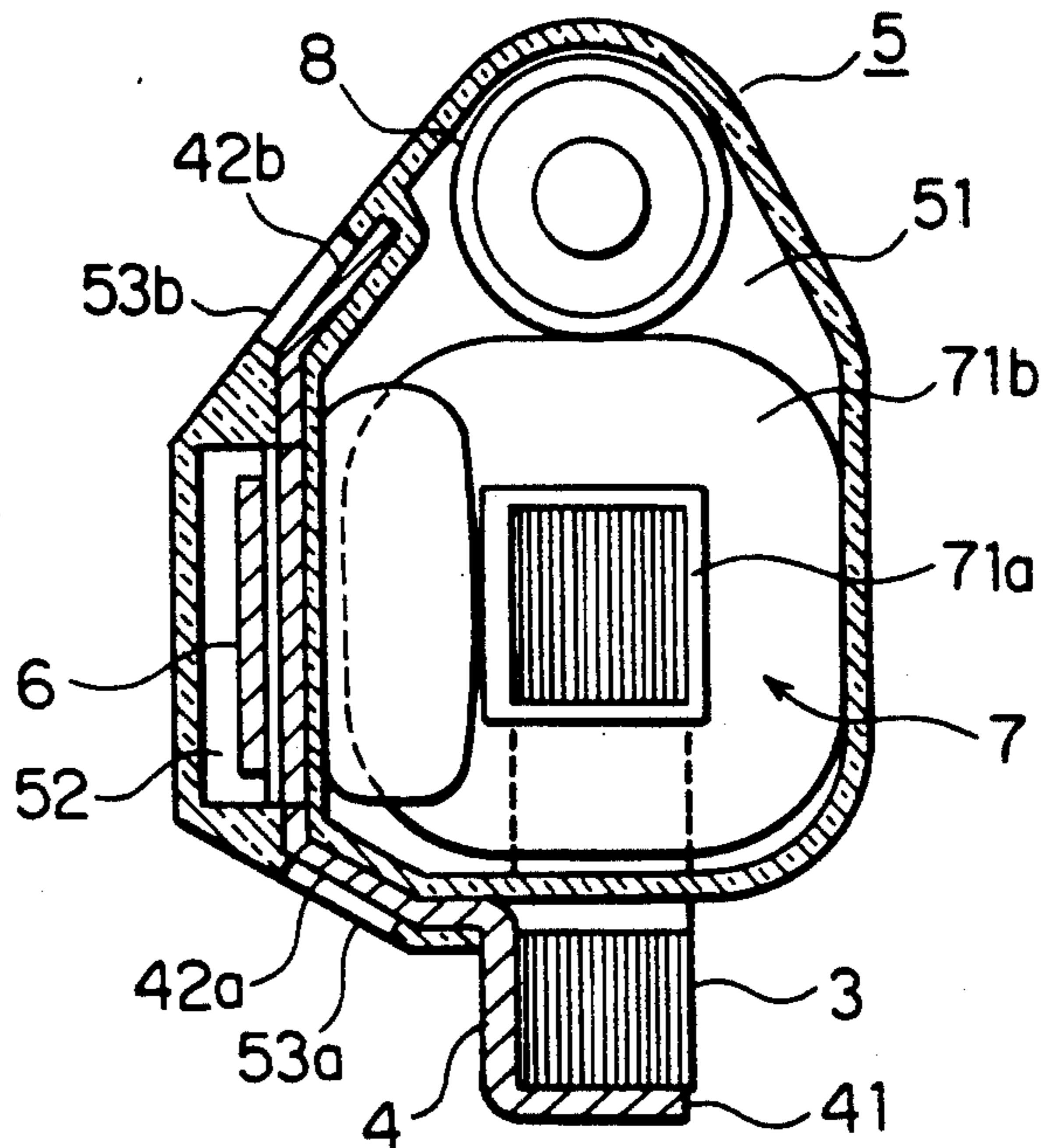
FIG. 4 PRIOR ART
