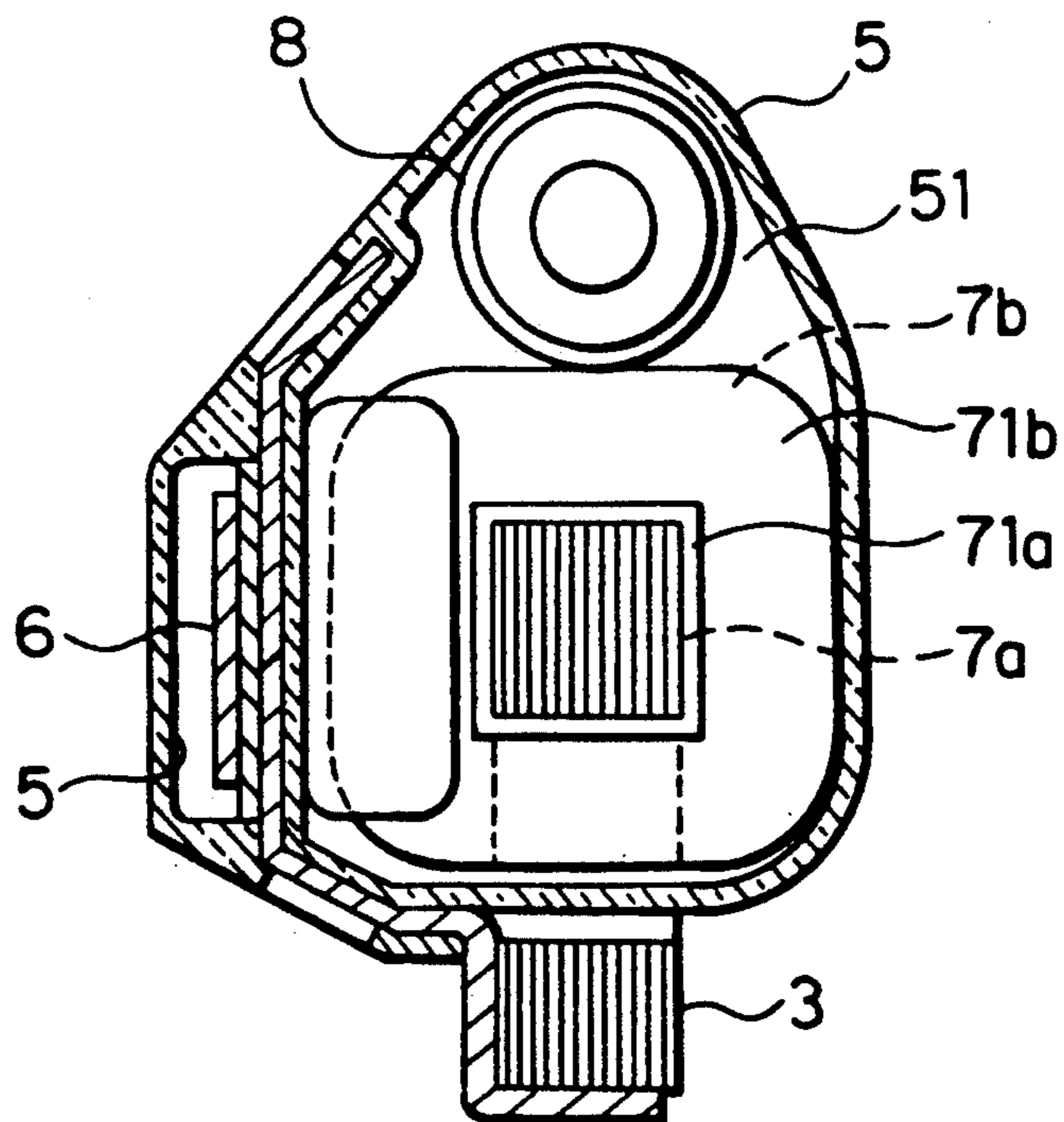
FIG. 9 PRIOR ART
