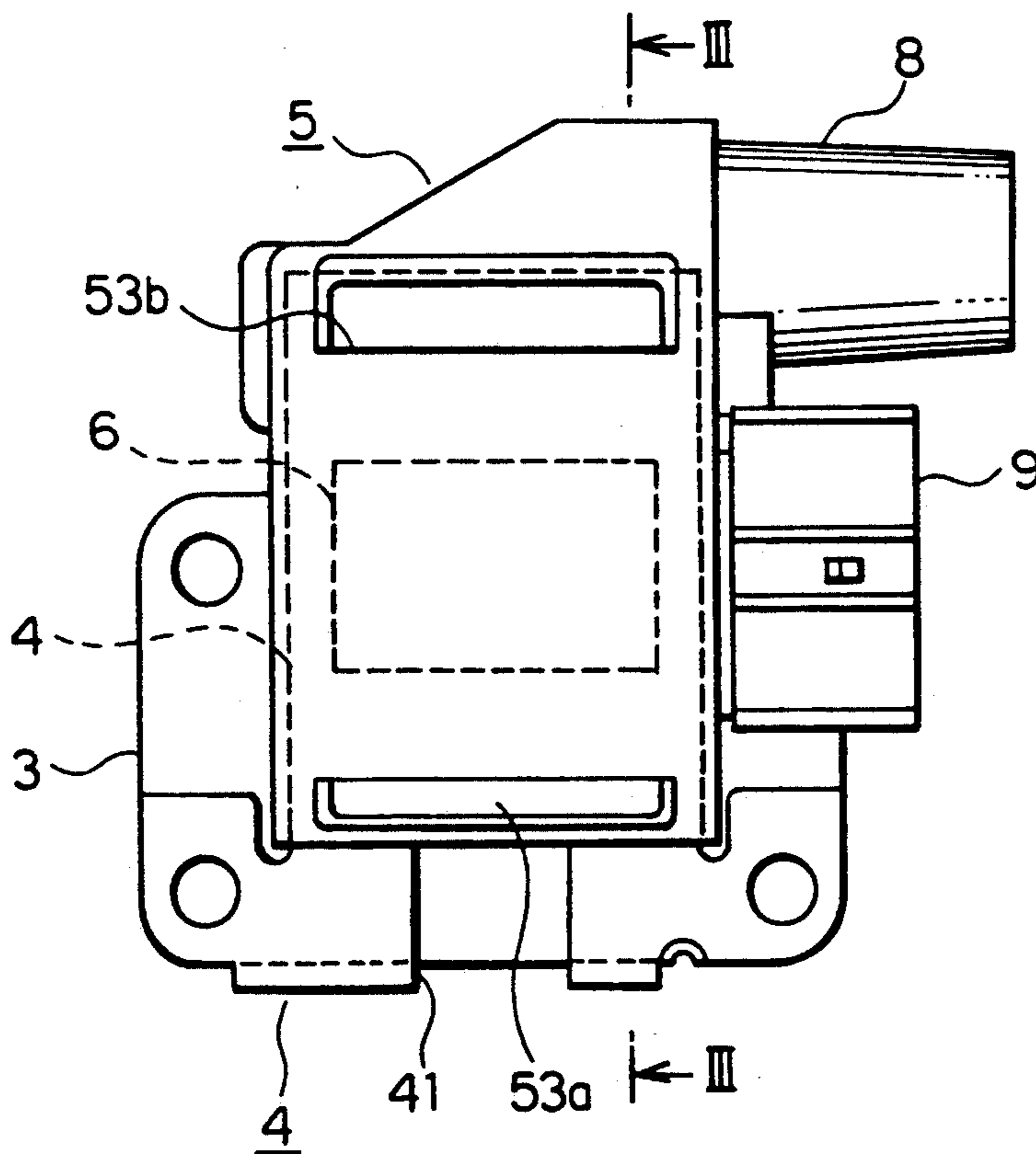
FIG. 4 PRIOR ART
