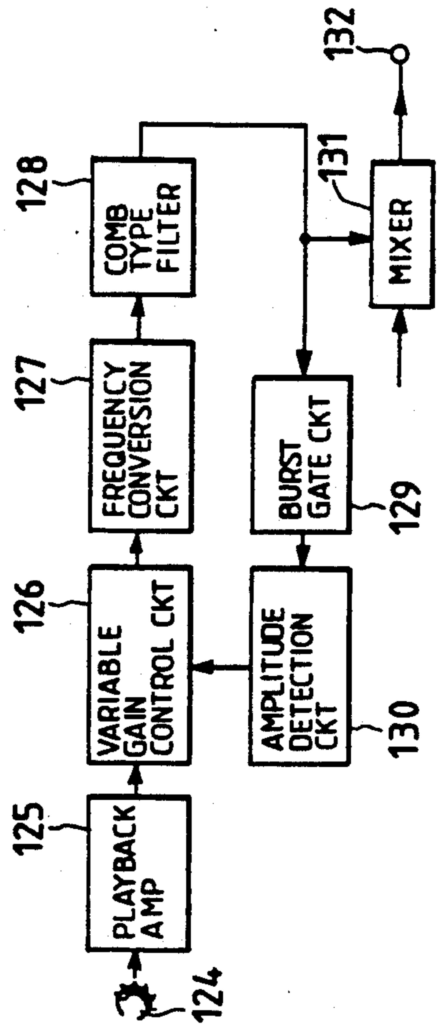
FIG. 29 PRIOR ART
