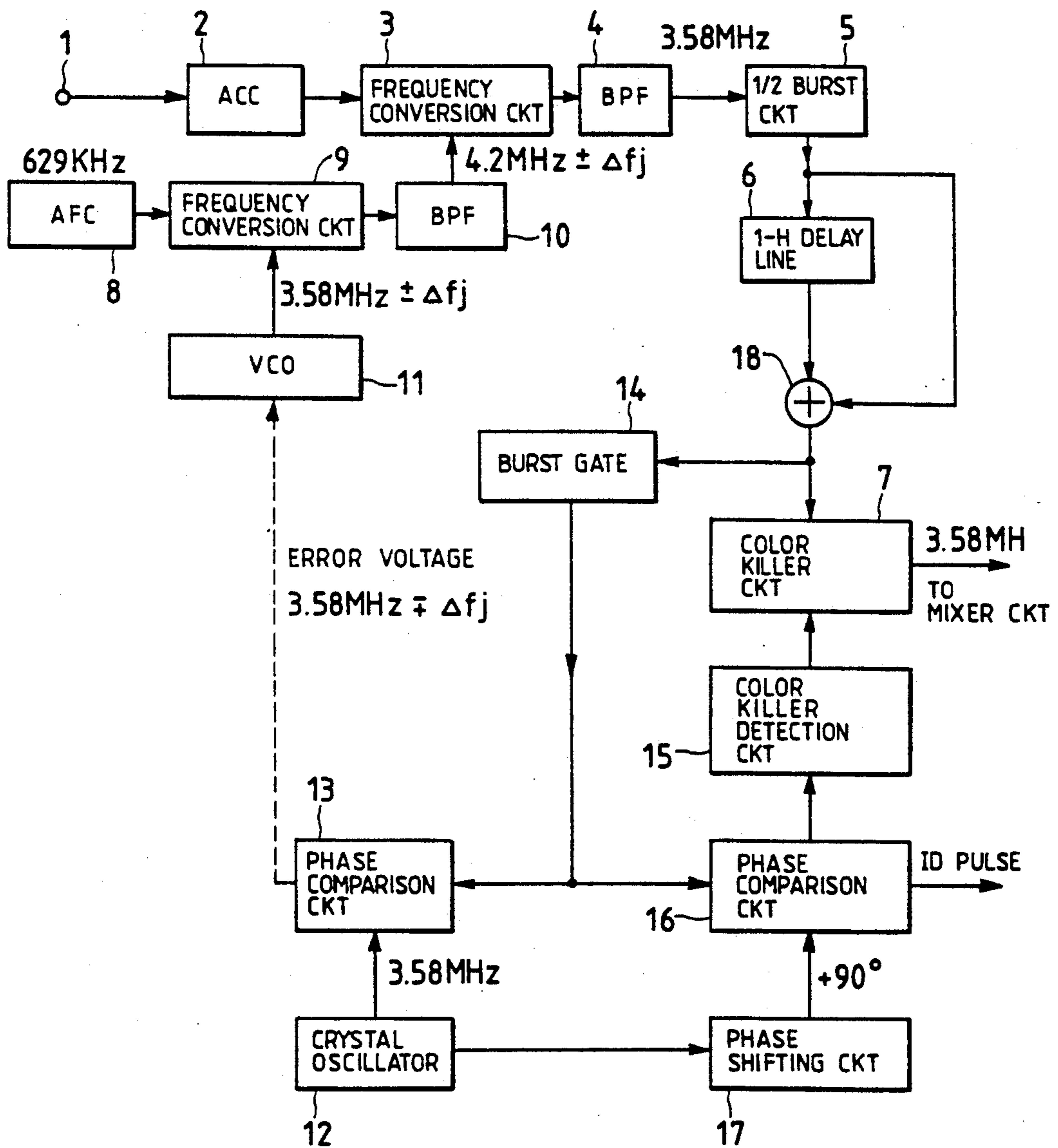
FIG. 10 PRIOR ART
