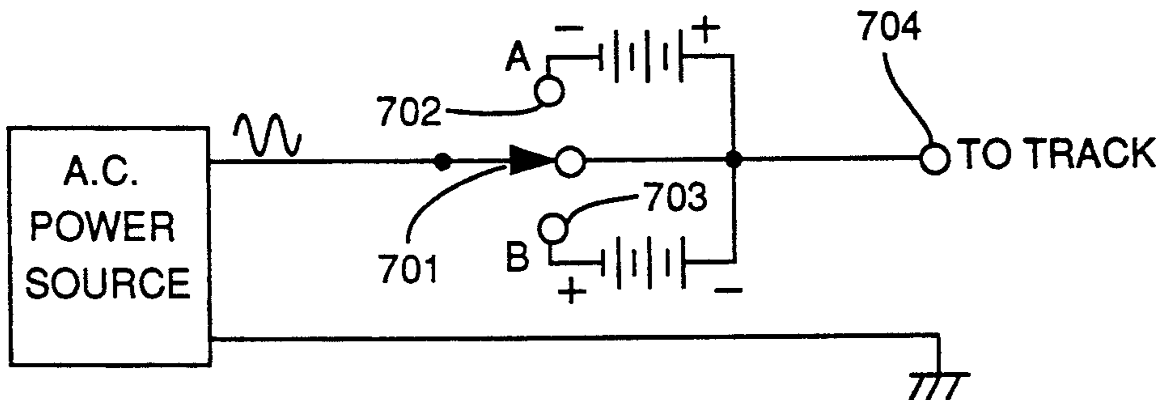
FIG. 7 ± D.C. SIGNAL GENERATORS
