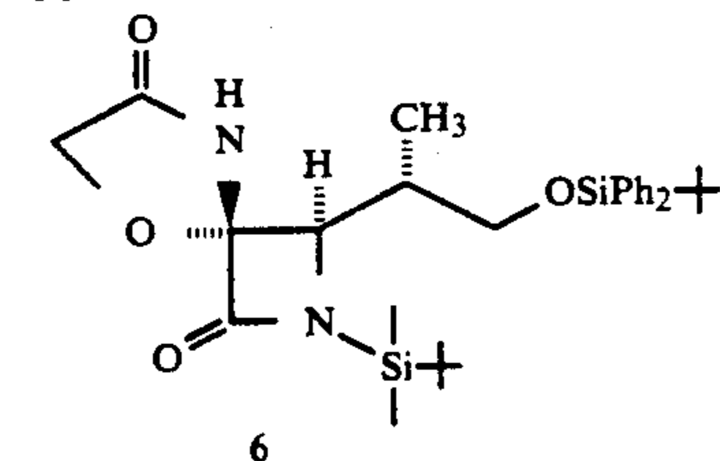
(±)-1-t-Butyldimethylsilyl-4R-(1-t-butyl-diphenylsilyloxy-2S-propyl)-3R-spiro[2-(1,3-oxazolidin-4-one)]-azetidin-2-one (6)
