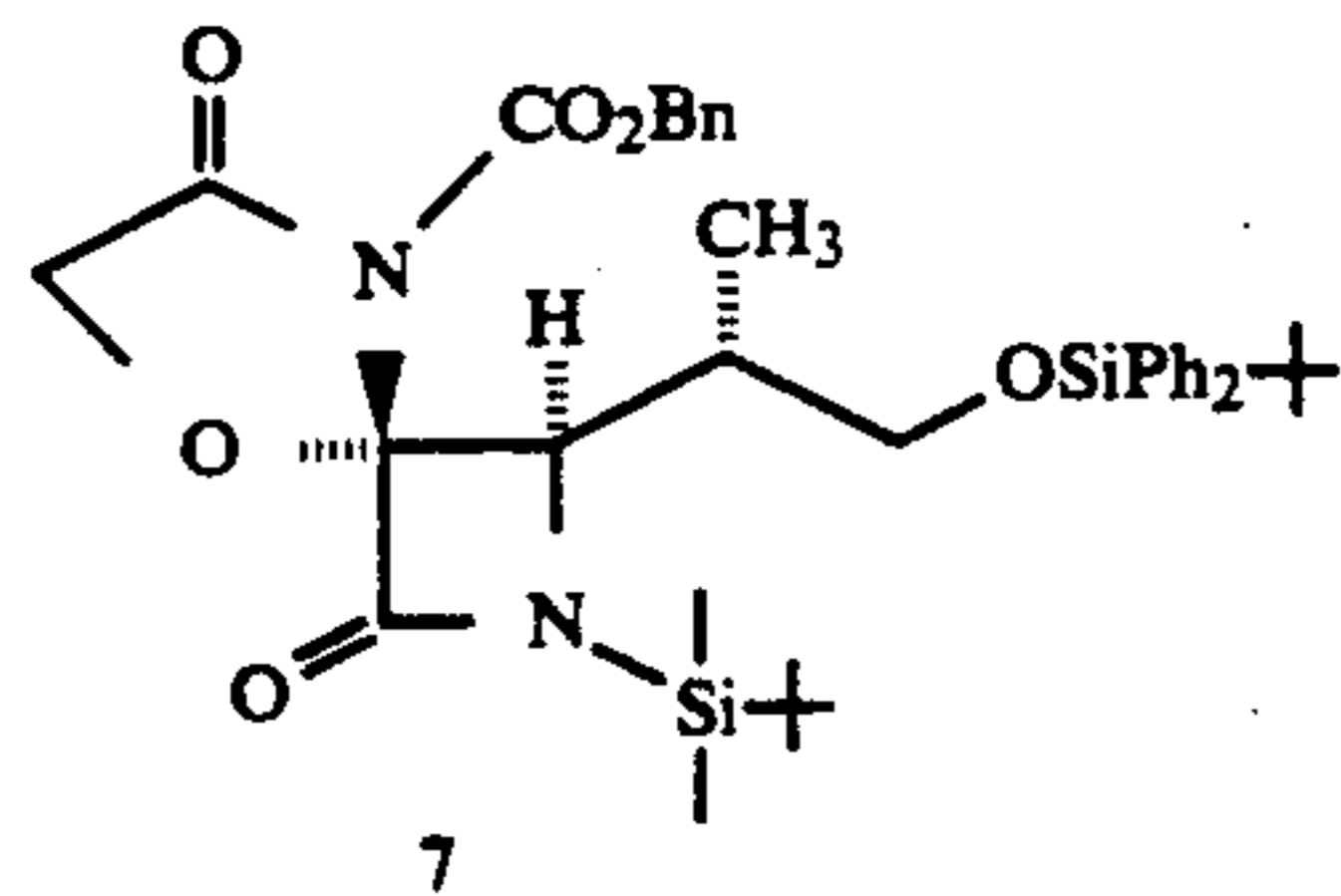
(±)-1-t-Butyldimethylsilyl-4R-(1-t-butyl-diphenylsilyloxy-2S-propyl)-3R-spiro[2-(3-benzyloxycarbonyl-1,3-oxazolidin-4-one)]-azetidin-2-one (7)
