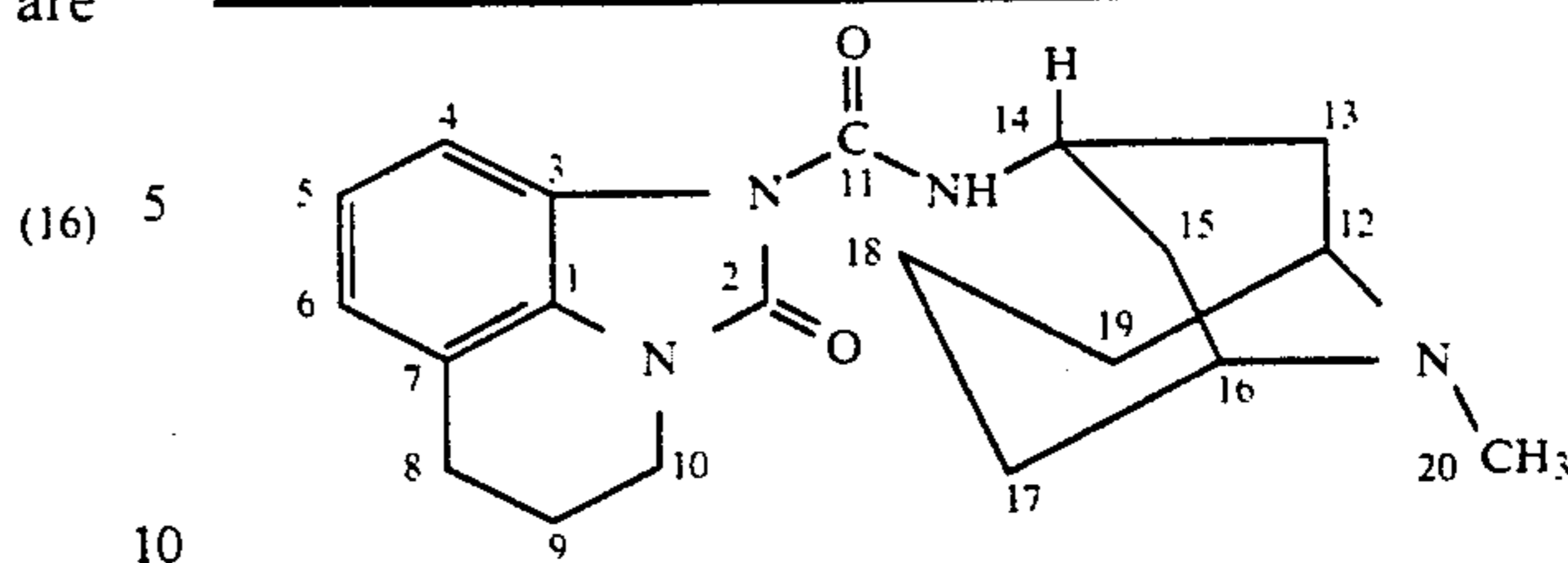
C-13-NMR (SLV: CDCl 3 , Ref. TMS)
