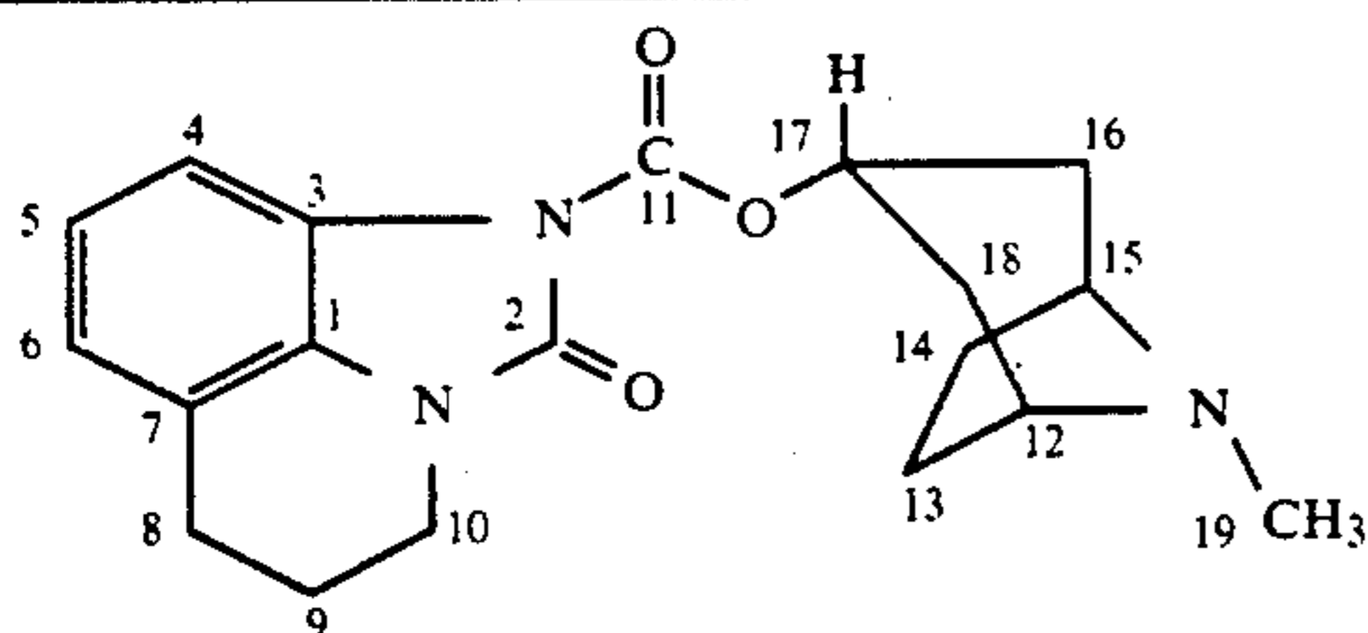
C-13-NMR SLV: CDCl 3 REF: TMS
