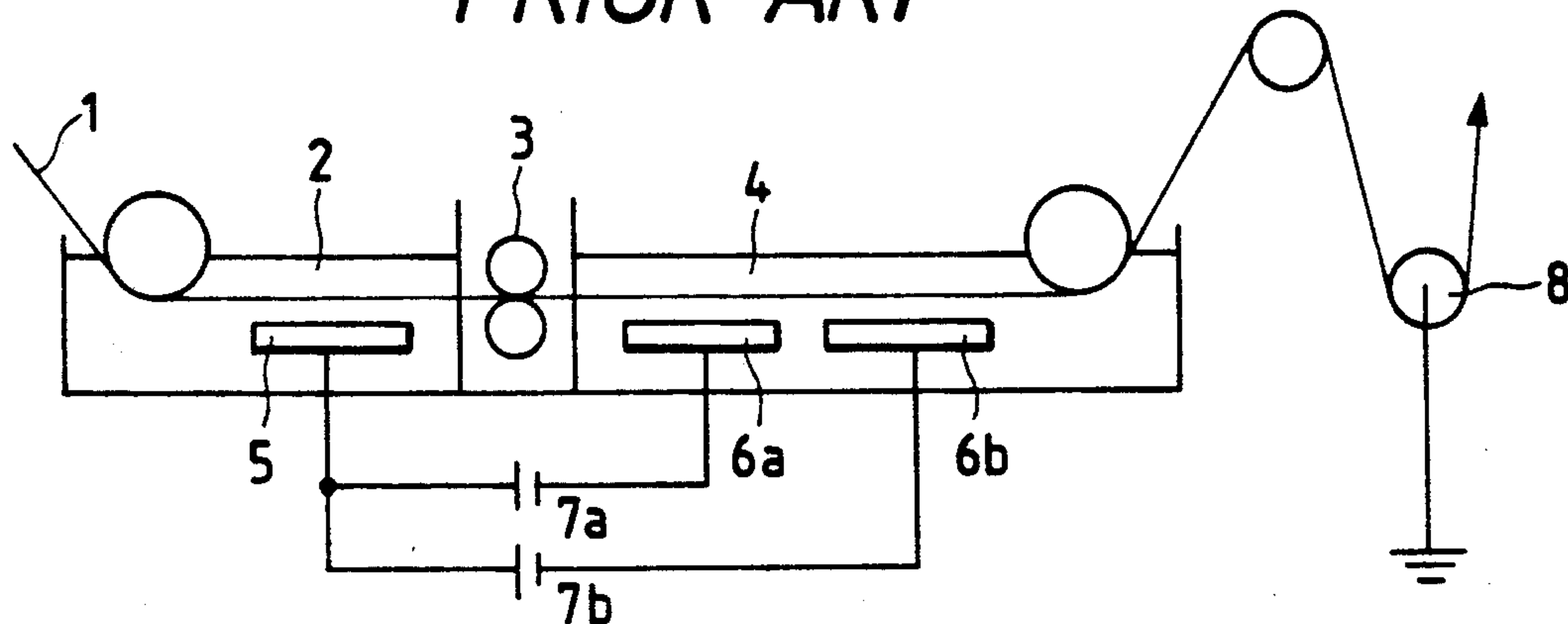
FIG. 4 PRIOR ART
