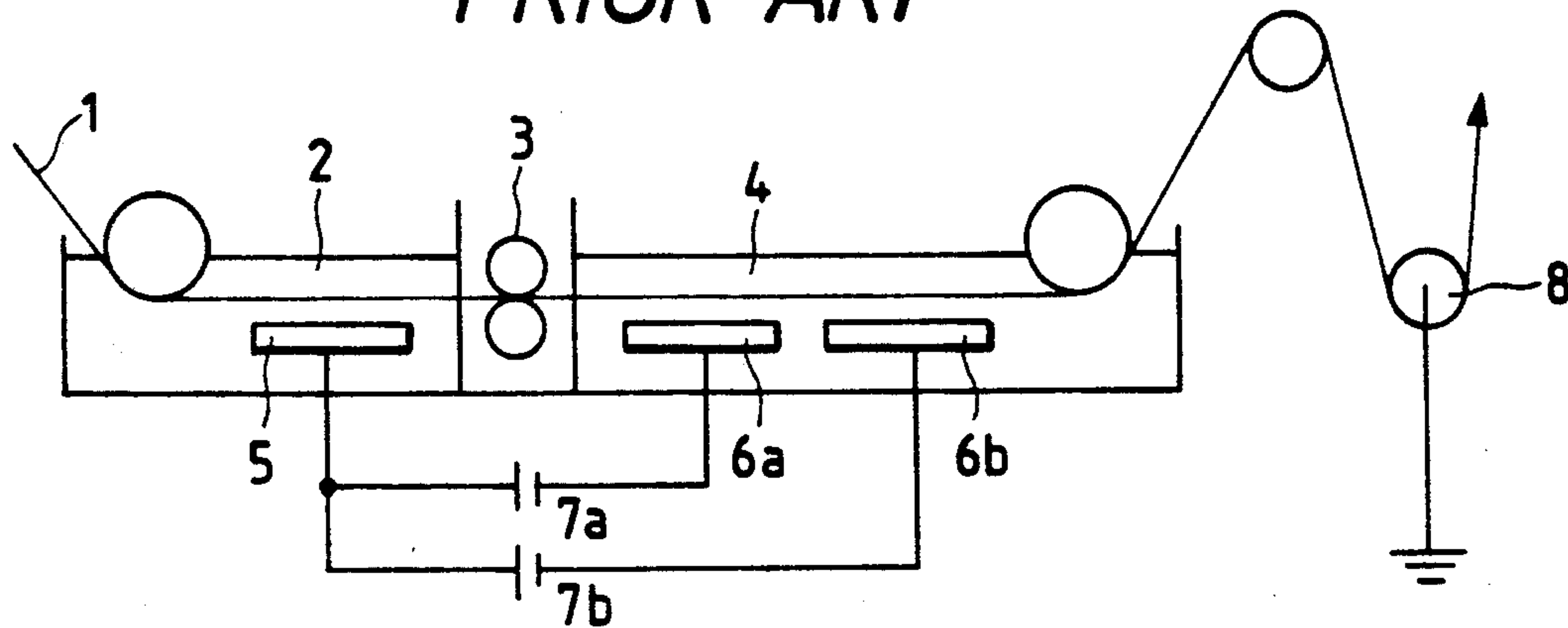
FIG. 4 PRIOR ART
