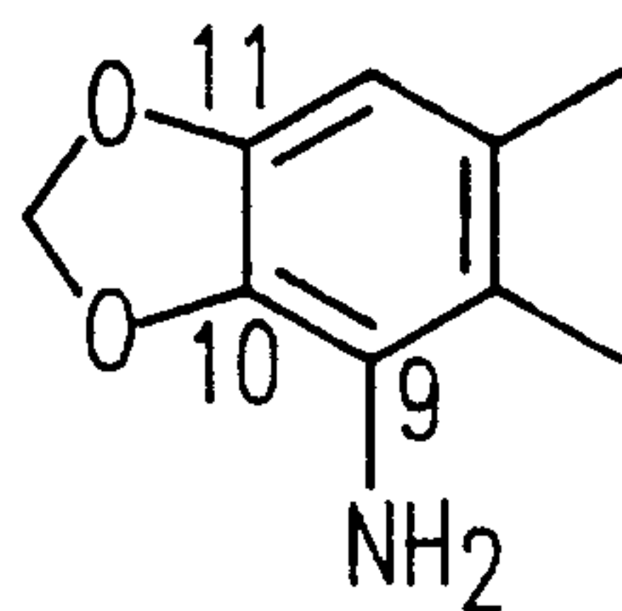
9-AMINO-10,11- MDO-20(RS)-CPT
