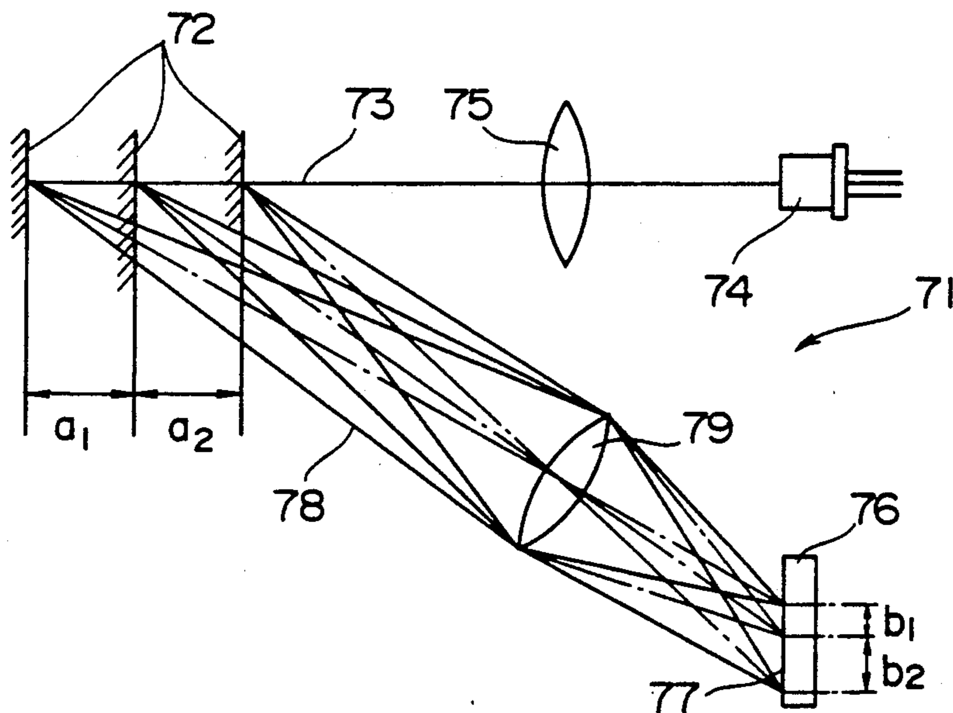
FIG. 12 PRIOR ART
