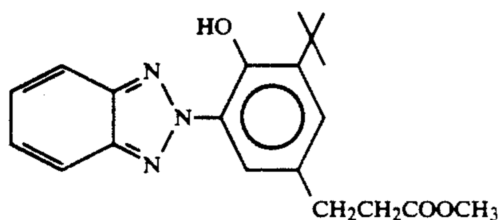
methyl-3-(3-(2H-benzotriazol-2-yl)-5-tert.butyl-4-hydroxy-phenyl)propionate
