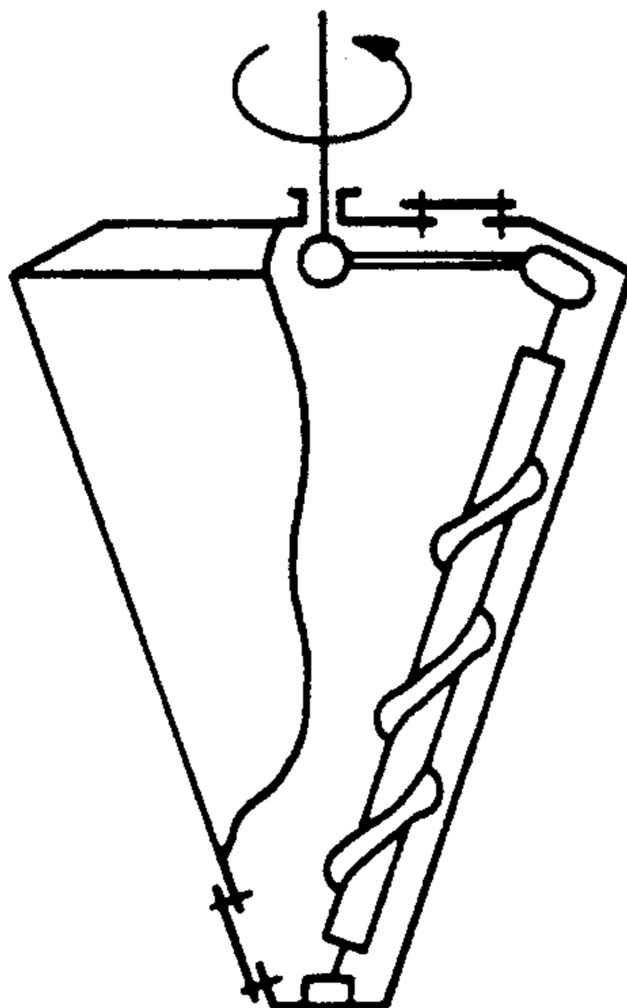
FIG. 7 PRIOR ART
