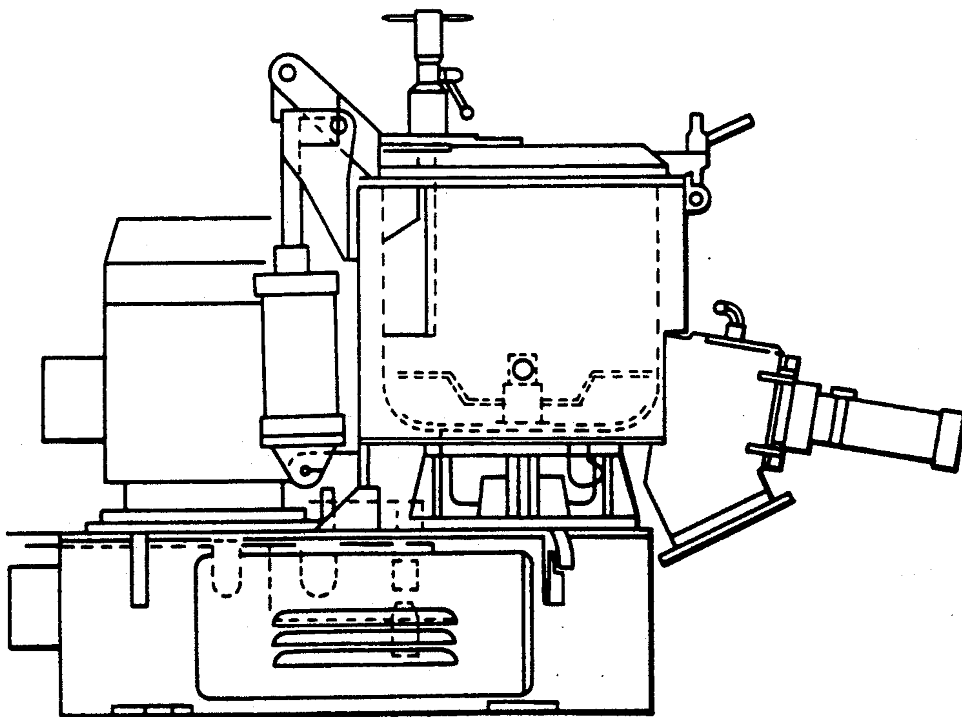
FIG. 8 PRIOR ART
