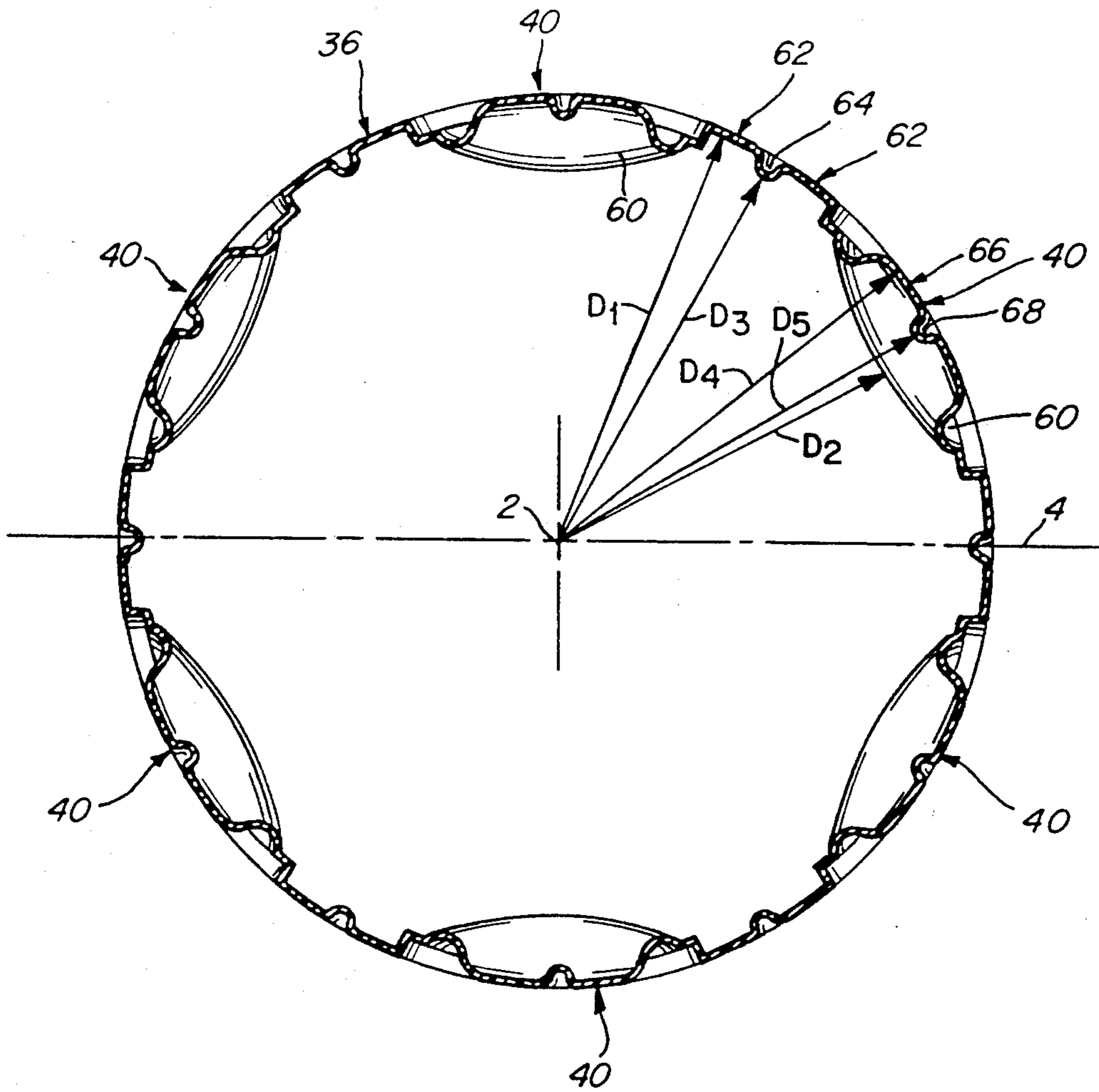
Fig. 2 (PRIOR ART)
