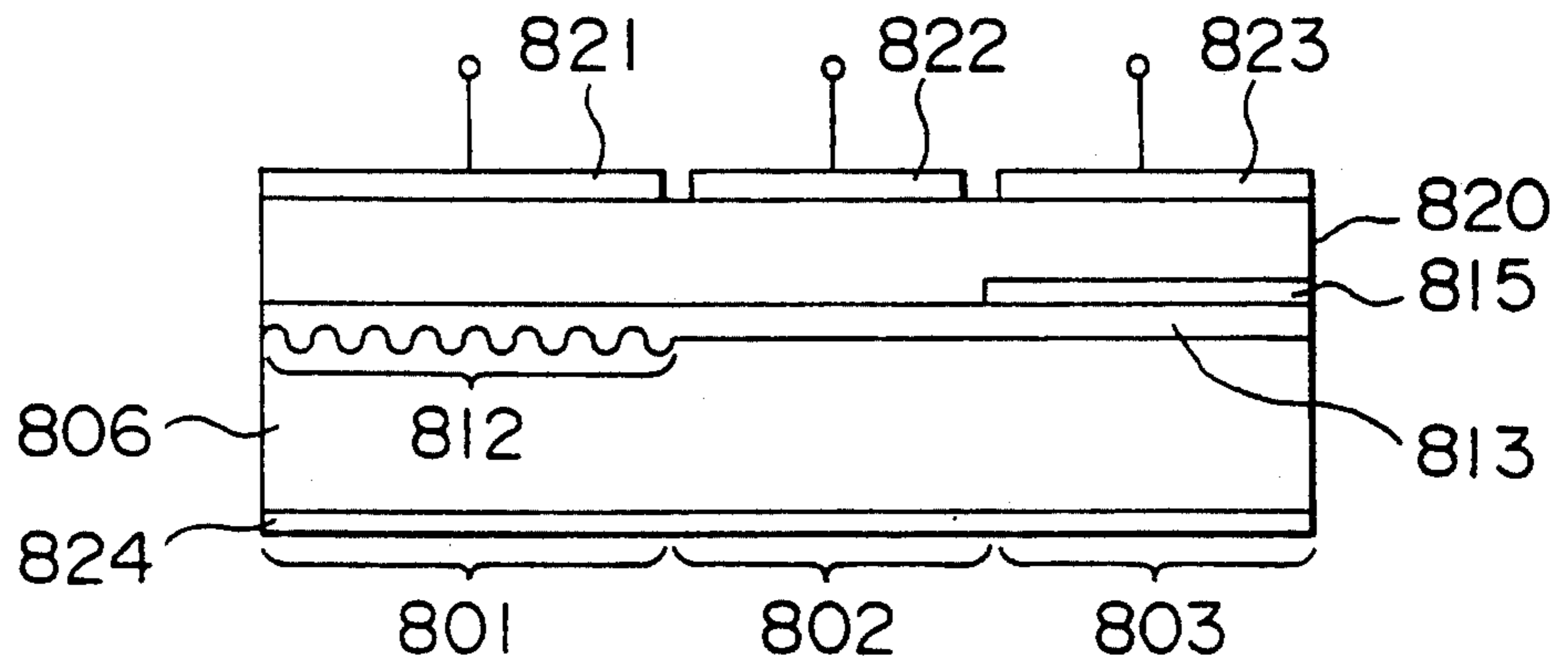
FIG. 8 PRIOR ART
