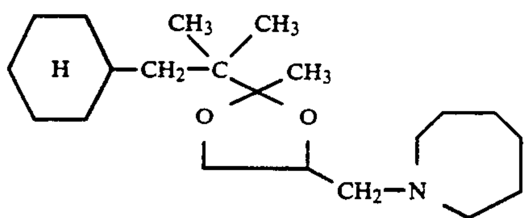
2-(2-cyclohexylmethyl-2-propyl)-2-methyl-4-(1-perhydroazepinylmethyl)-1,3-dioxolane
