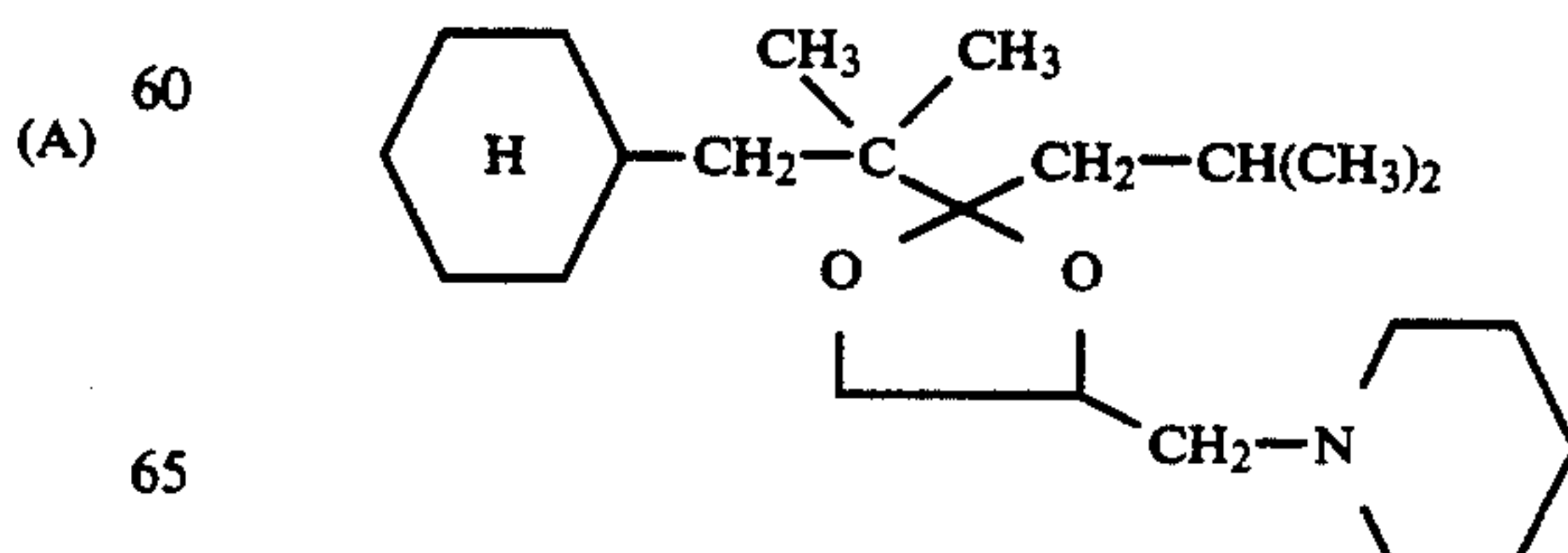
2-(2-Cyclohexylmethyl-2-propyl)-2-methyl-4-(1-piperidinyl)-1,3-dioxolane
