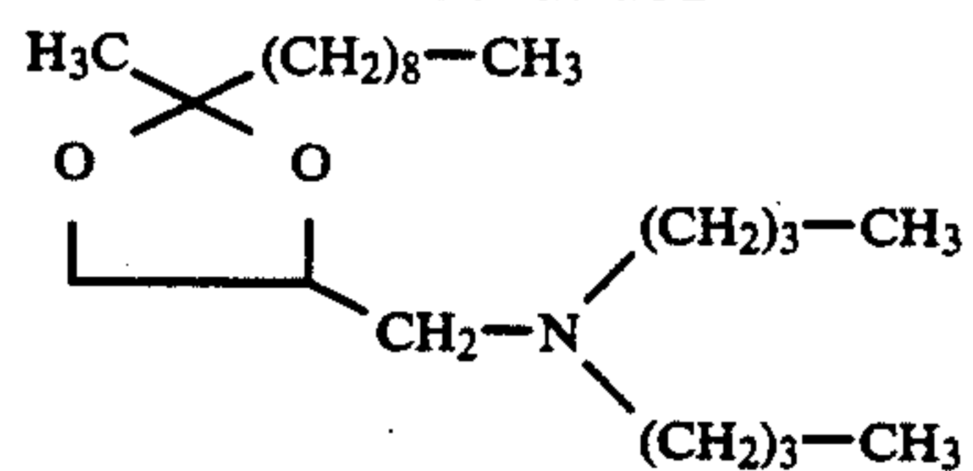
2-Methyl-2-nonyl-4-di-n-butylaminomethyl-1,3-dioxolane
