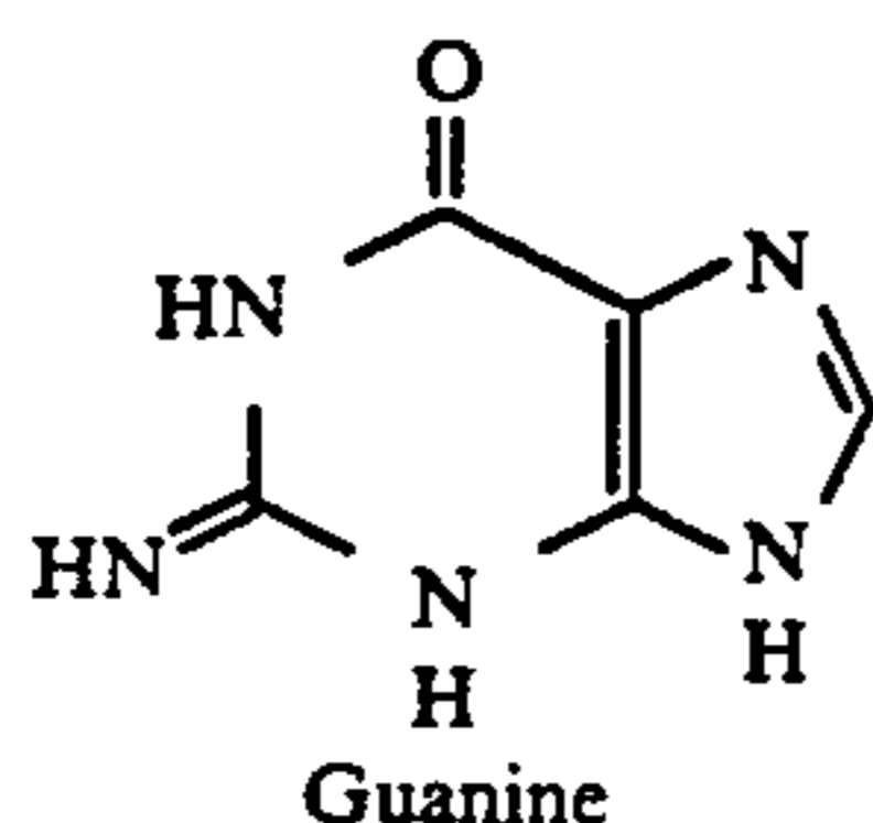
Guanine
