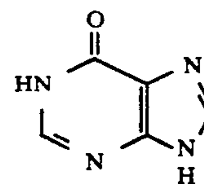
Hypoxanthine
