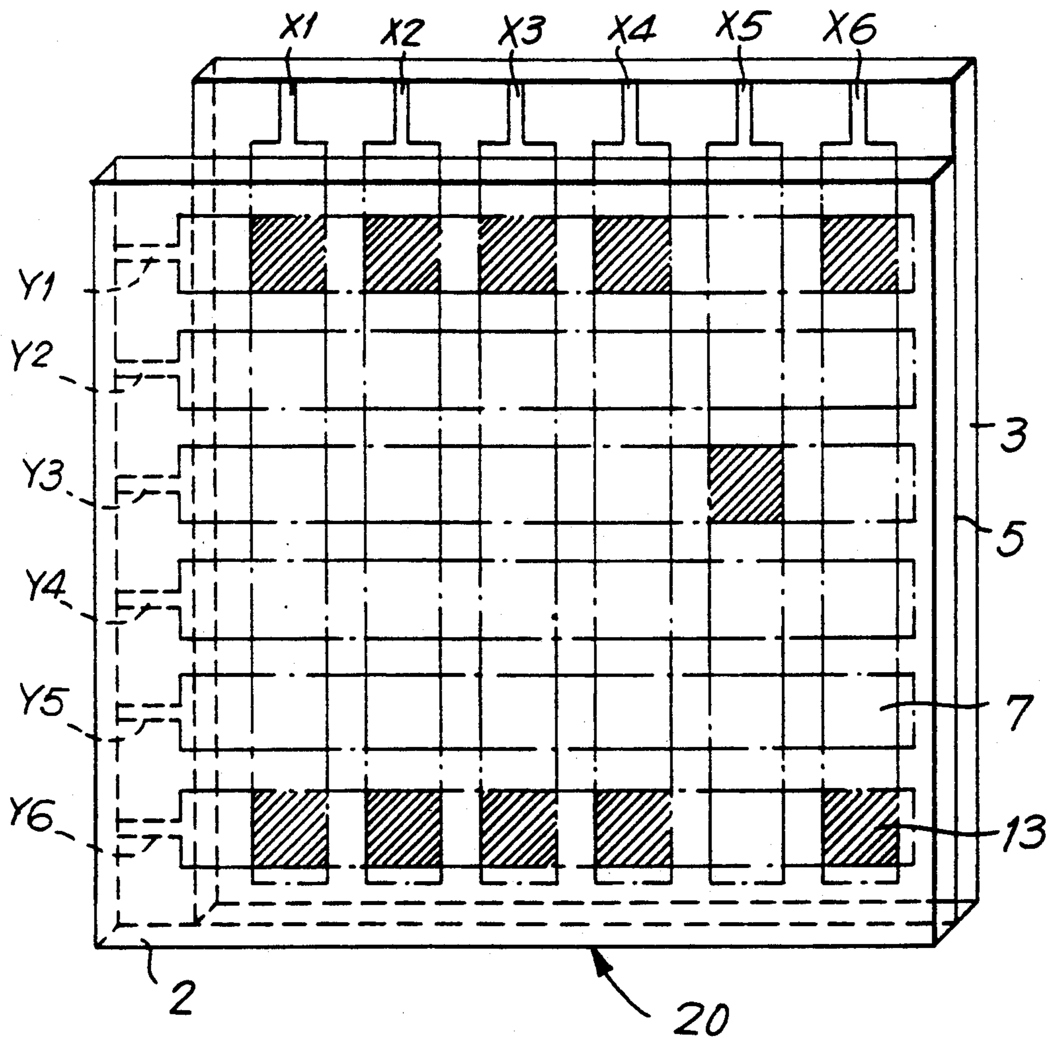
FIG. 23 PRIOR ART
