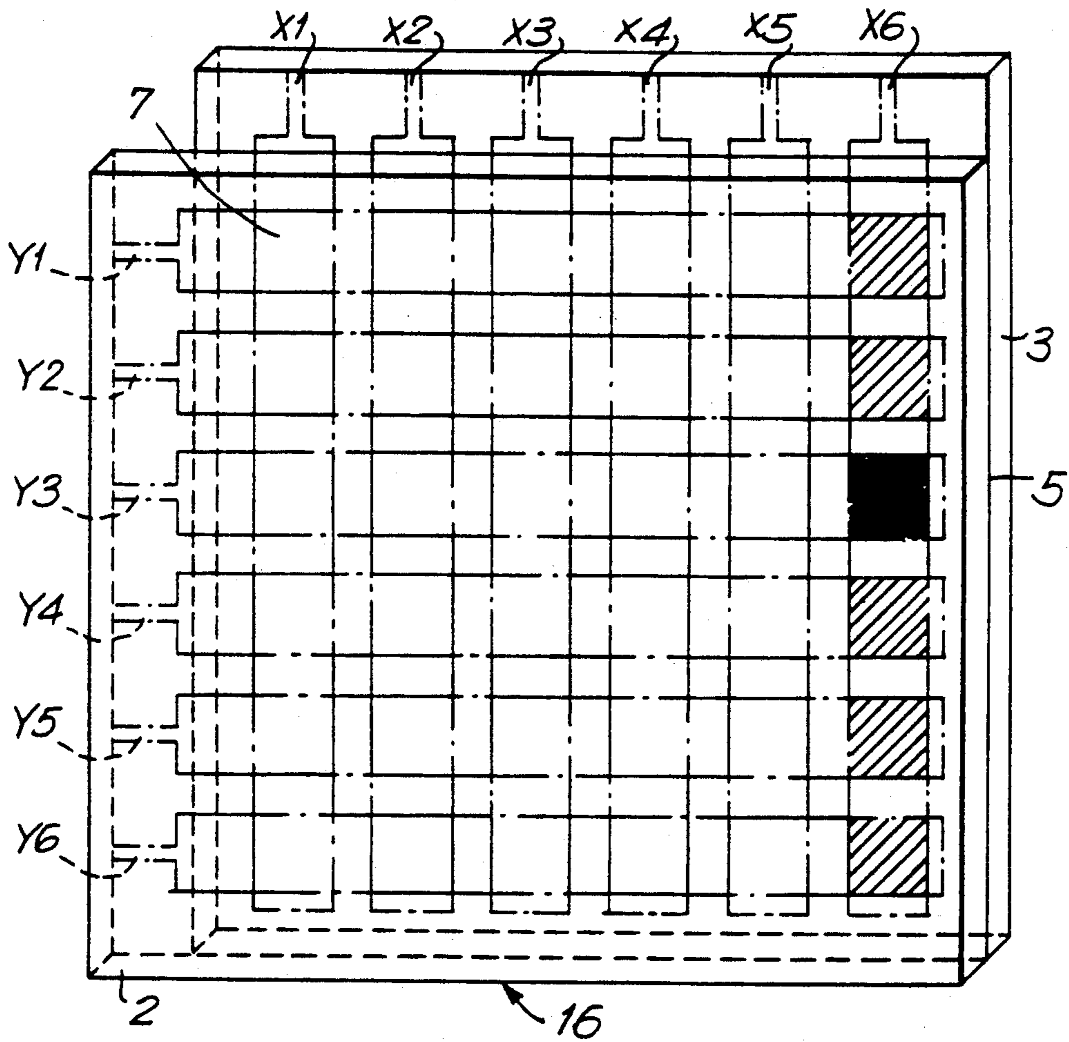
FIG. 15 PRIOR ART
