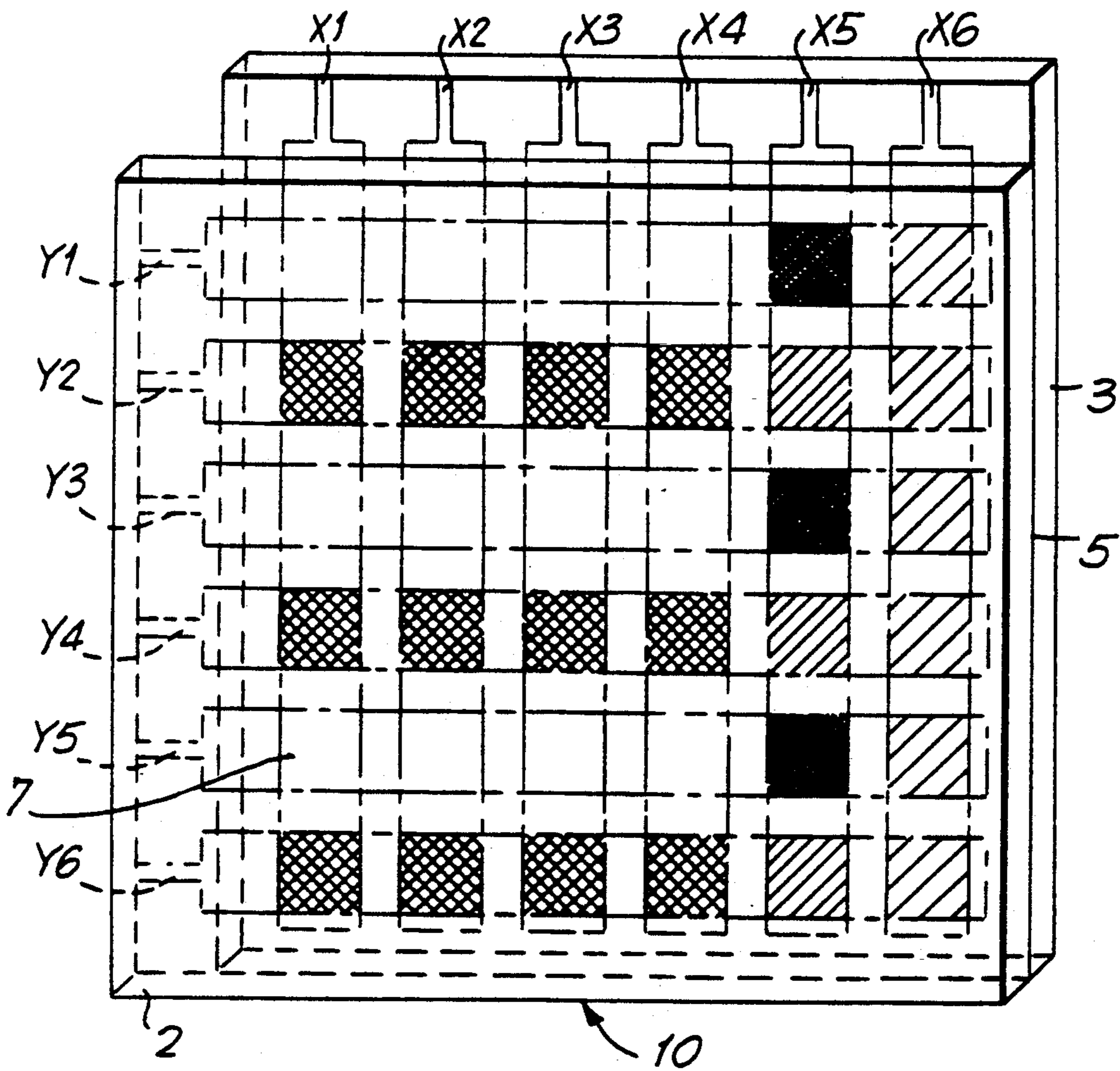
FIG. 4 PRIOR ART
