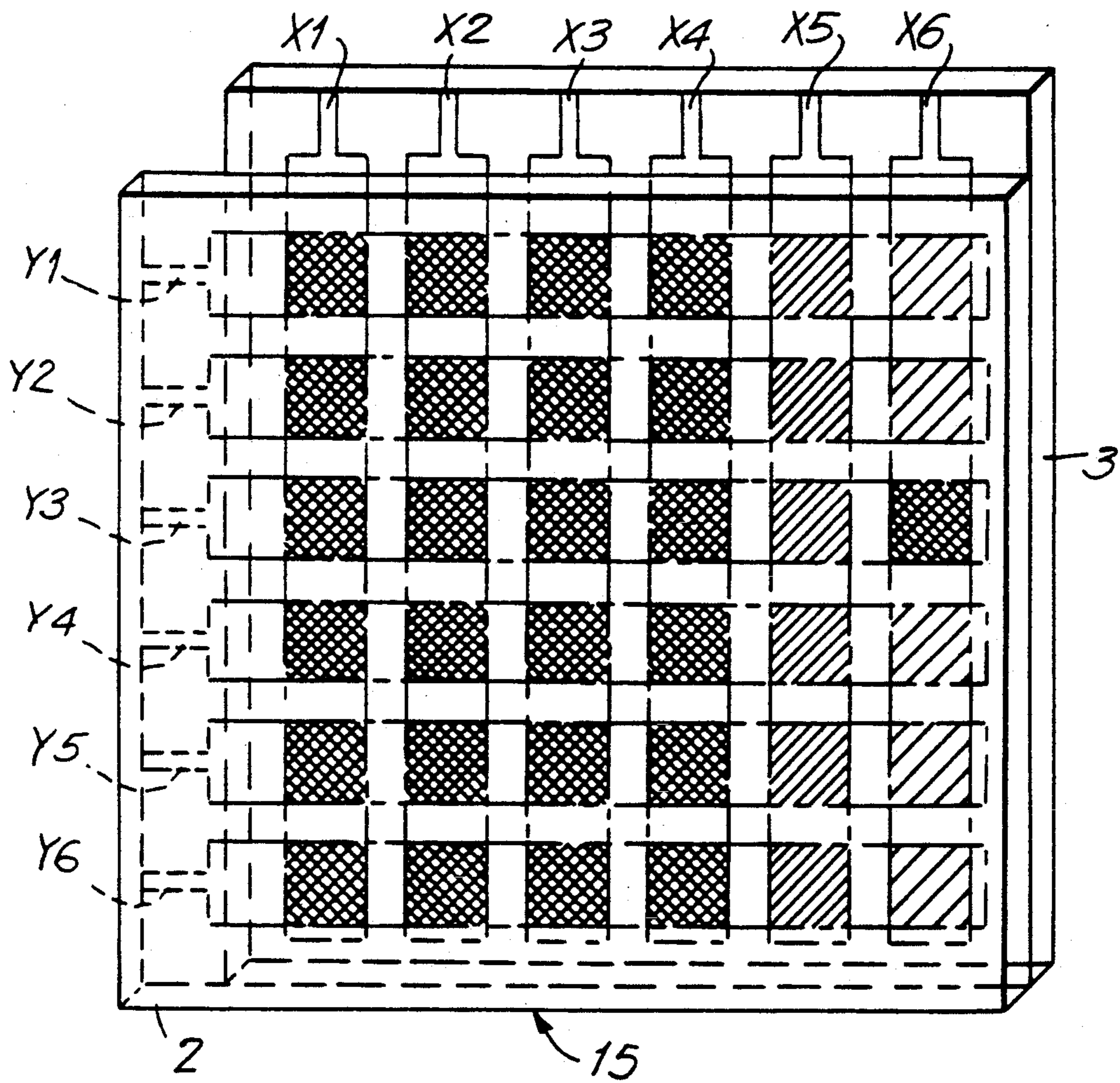
FIG. 12 PRIOR ART
