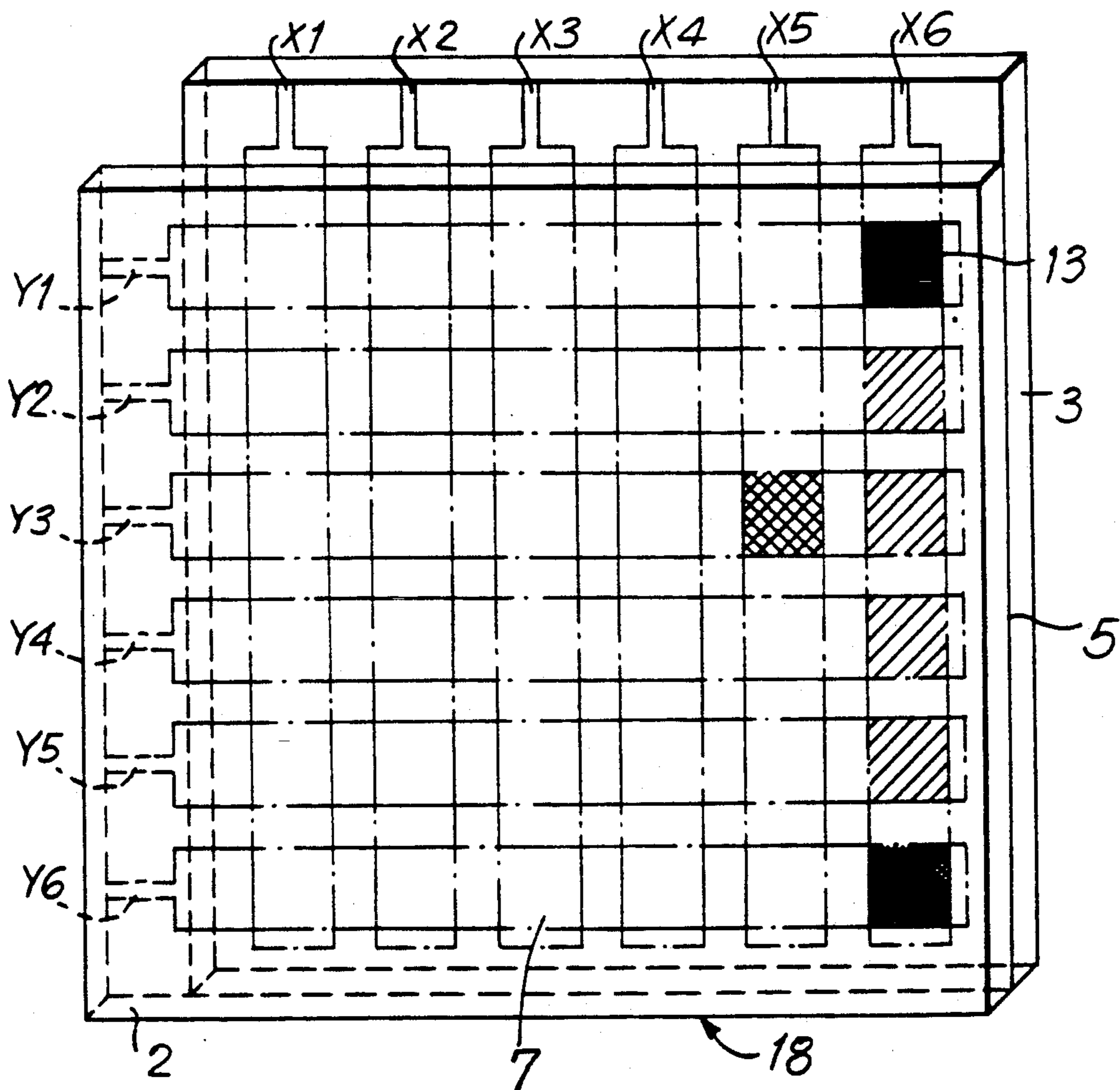
FIG. 20 PRIOR ART
