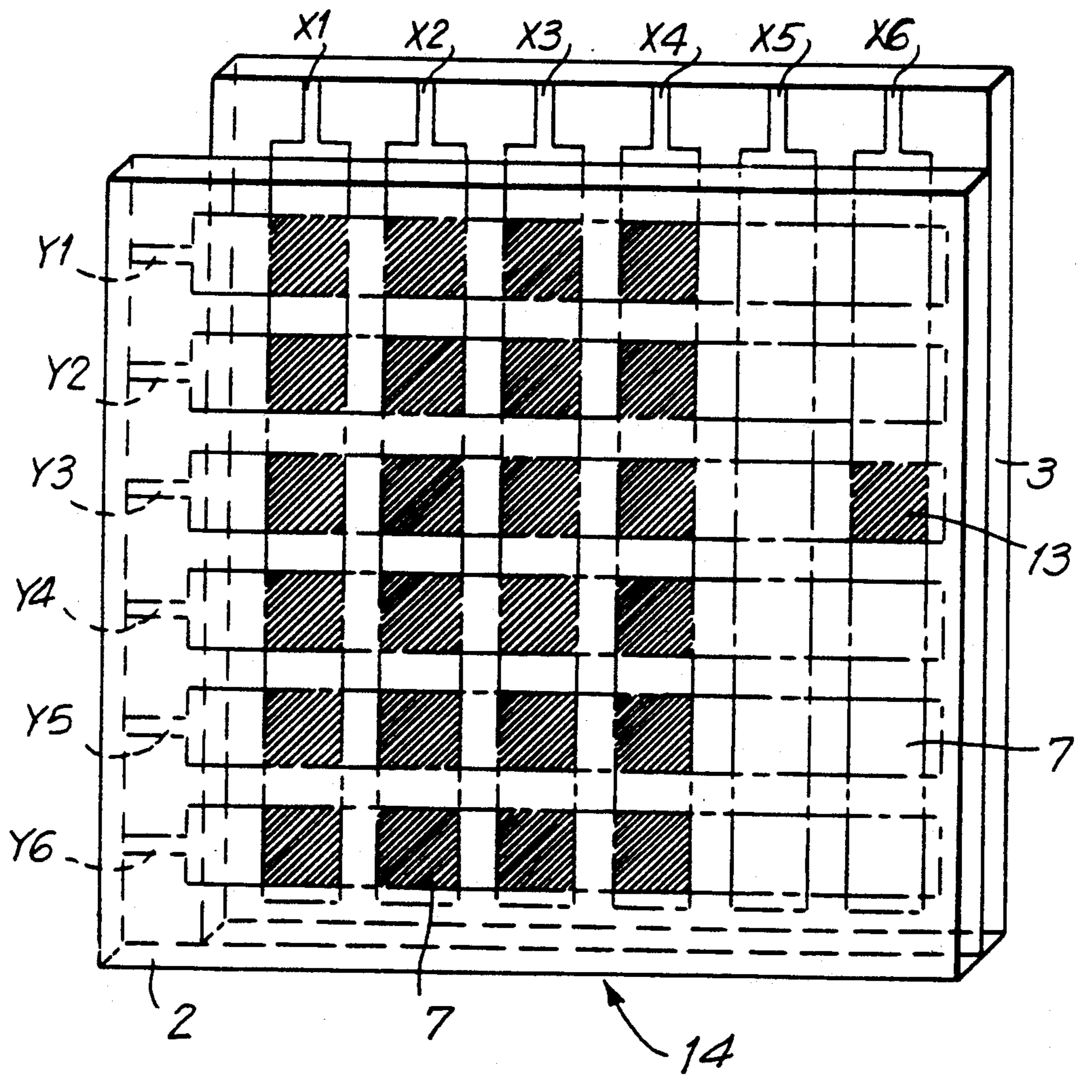
FIG. 11 PRIOR ART
