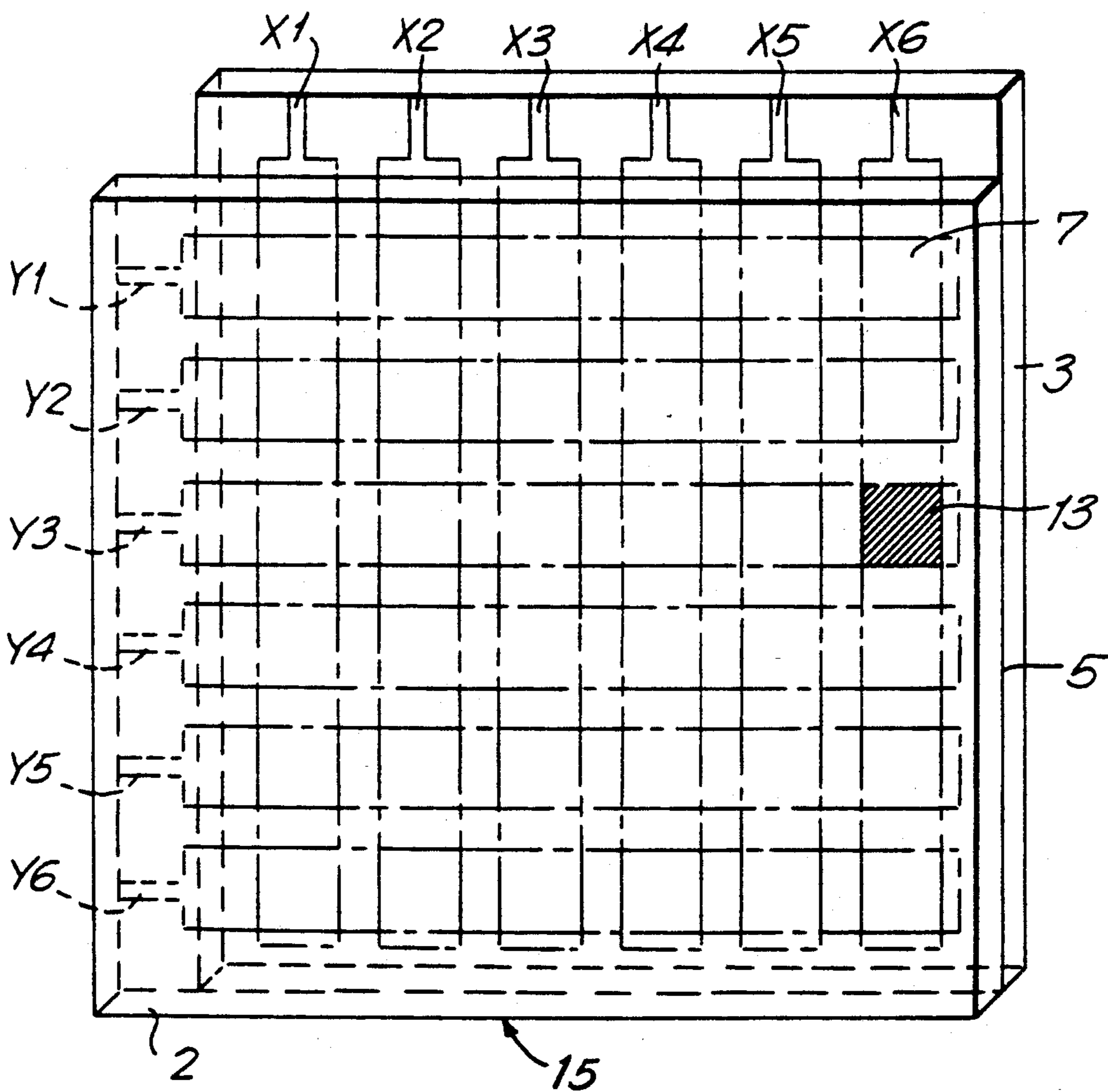
FIG. 16 PRIOR ART
