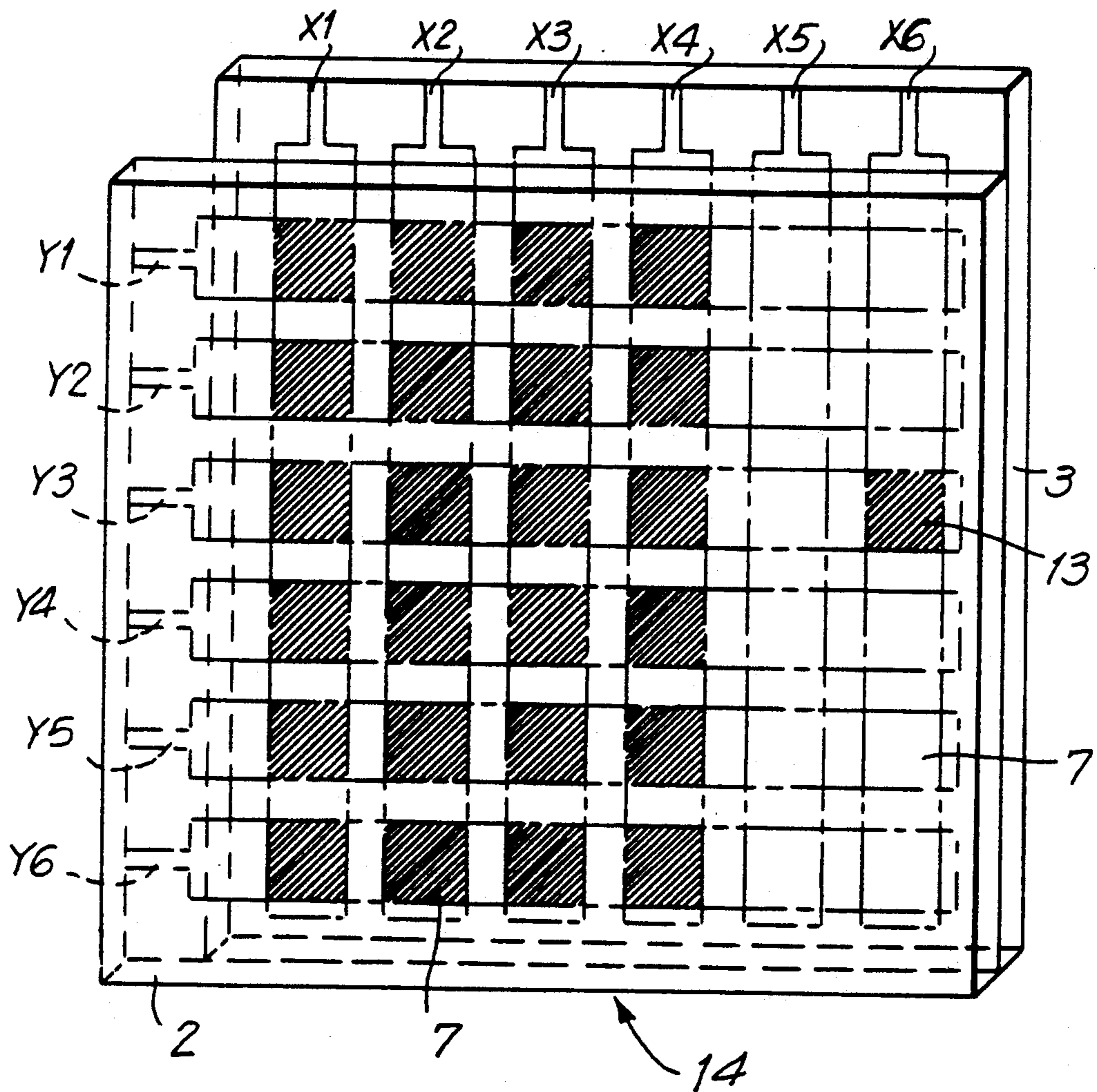
FIG. 11 PRIOR ART
