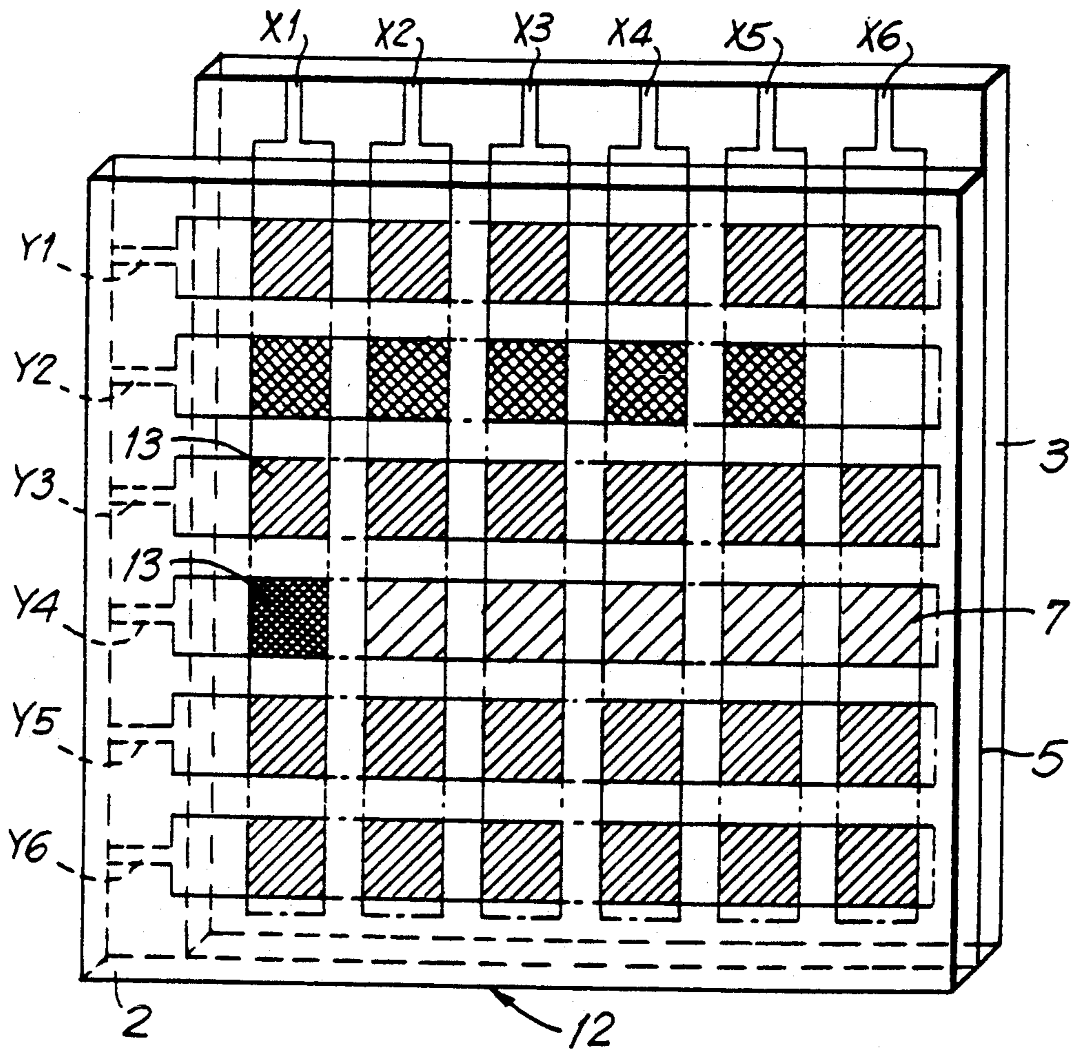
FIG. 8 PRIOR ART
