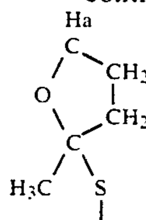
2-methyl tetrahydrofuranlyl
