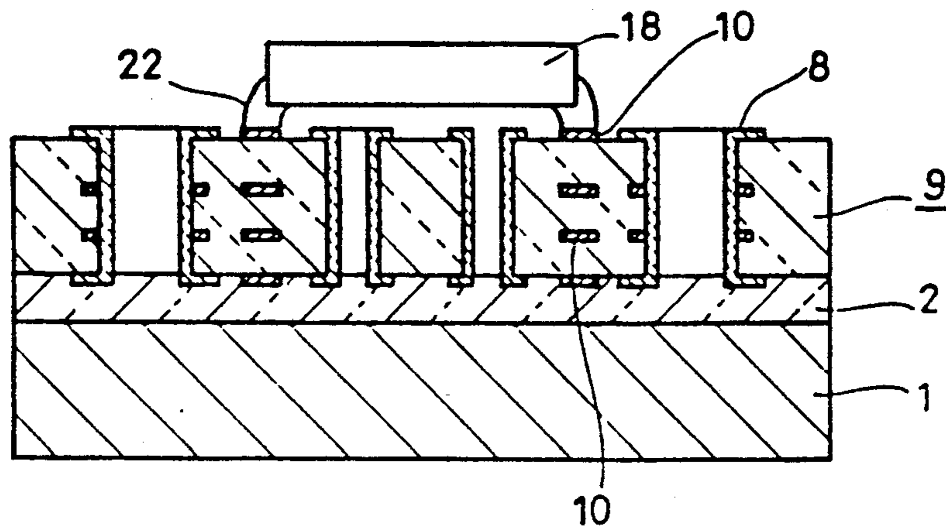
FIG.3 PRIOR ART
