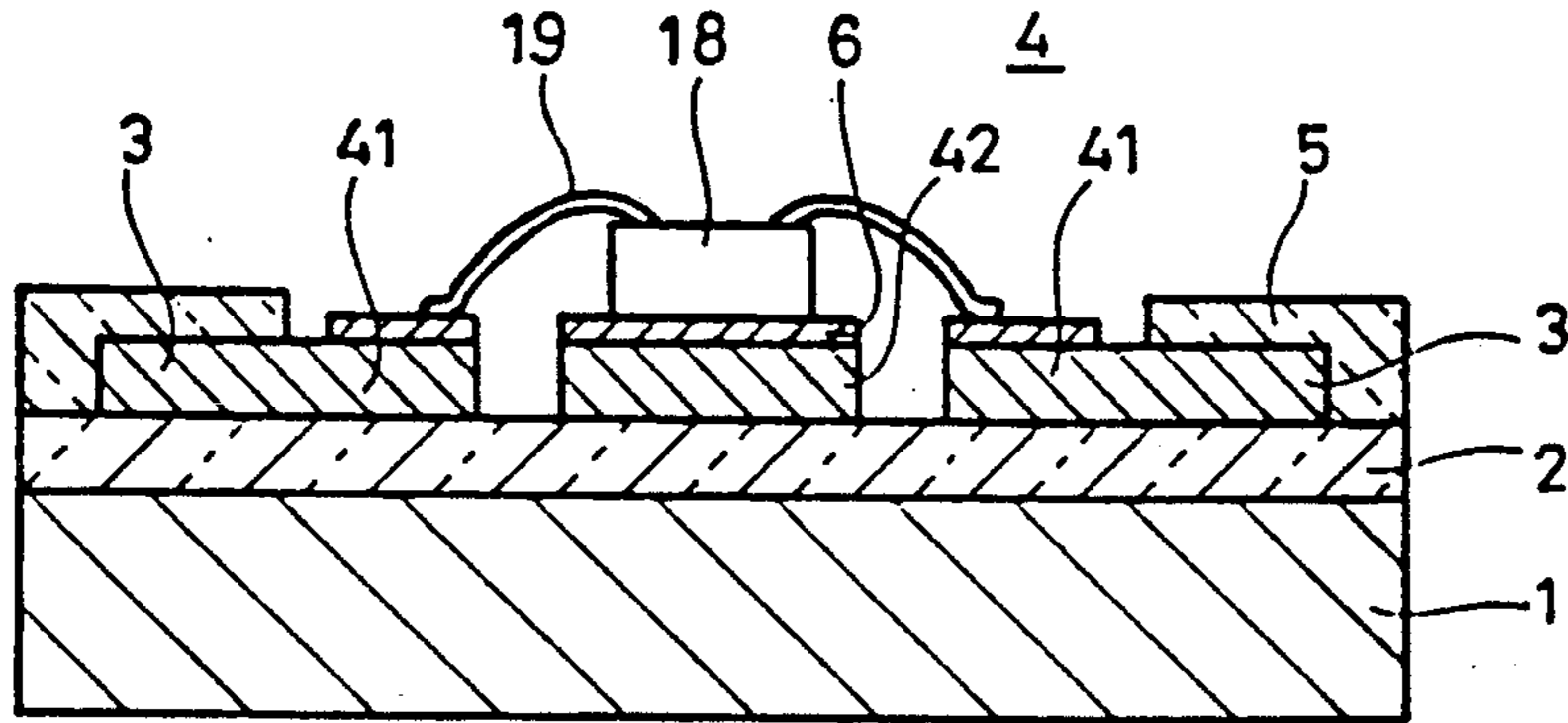
FIG.2 PRIOR ART
