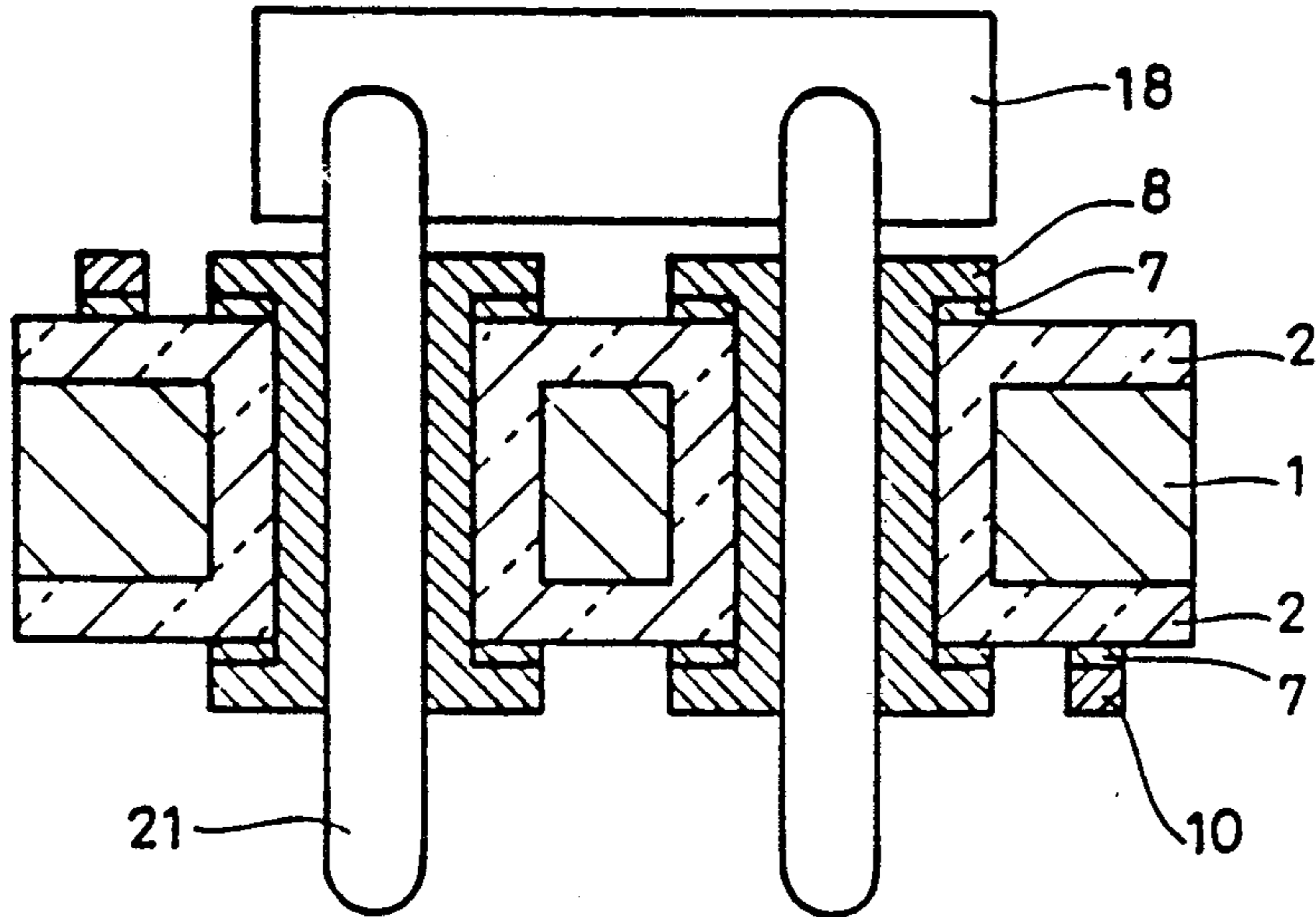
FIG.2 PRIOR ART
