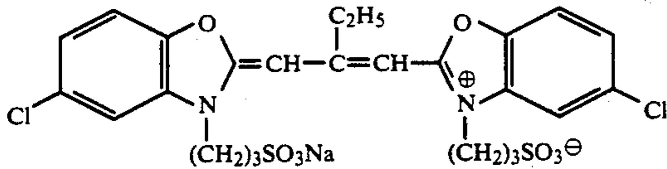
Sensitizing dye (2)
