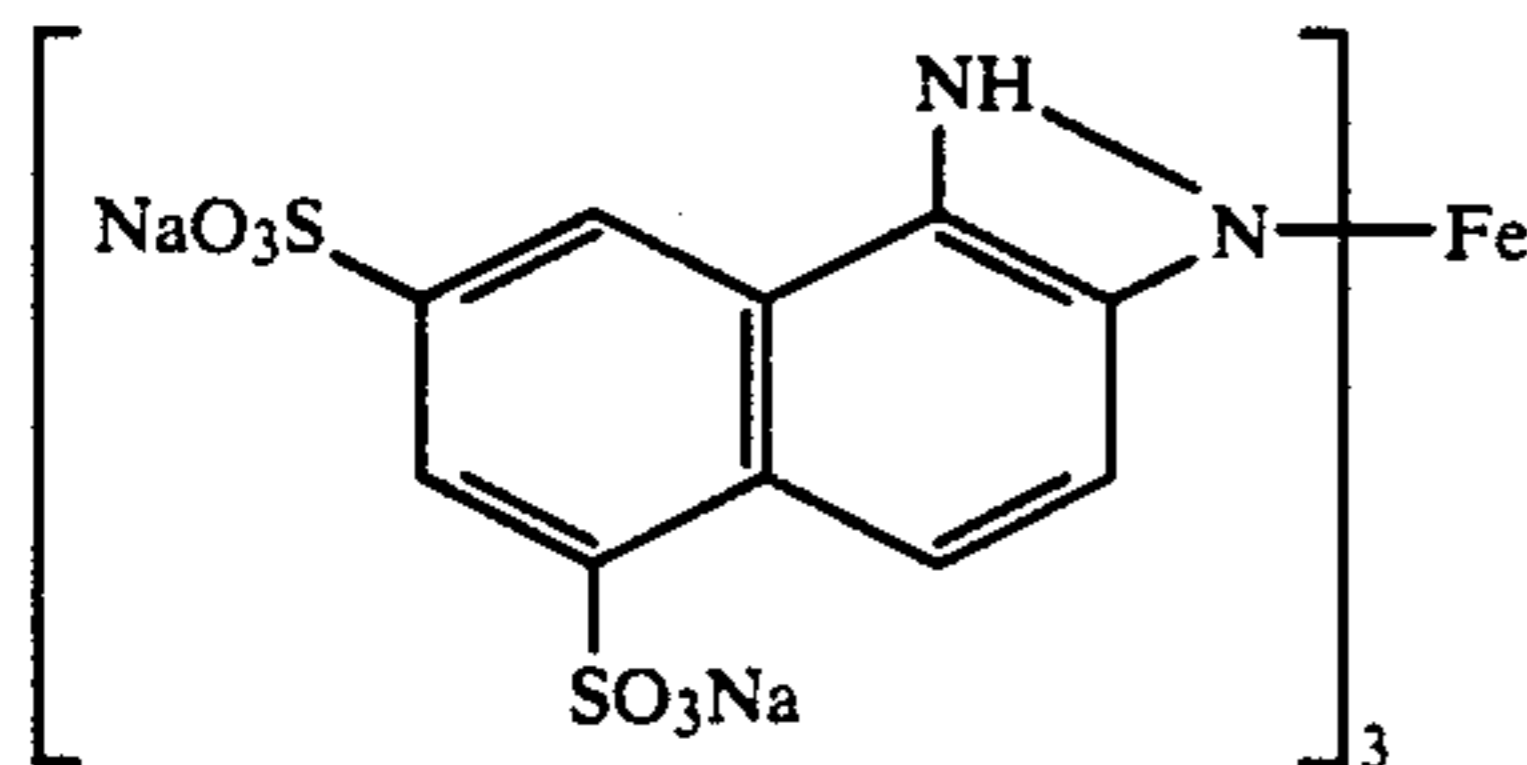
Antihalation dye
