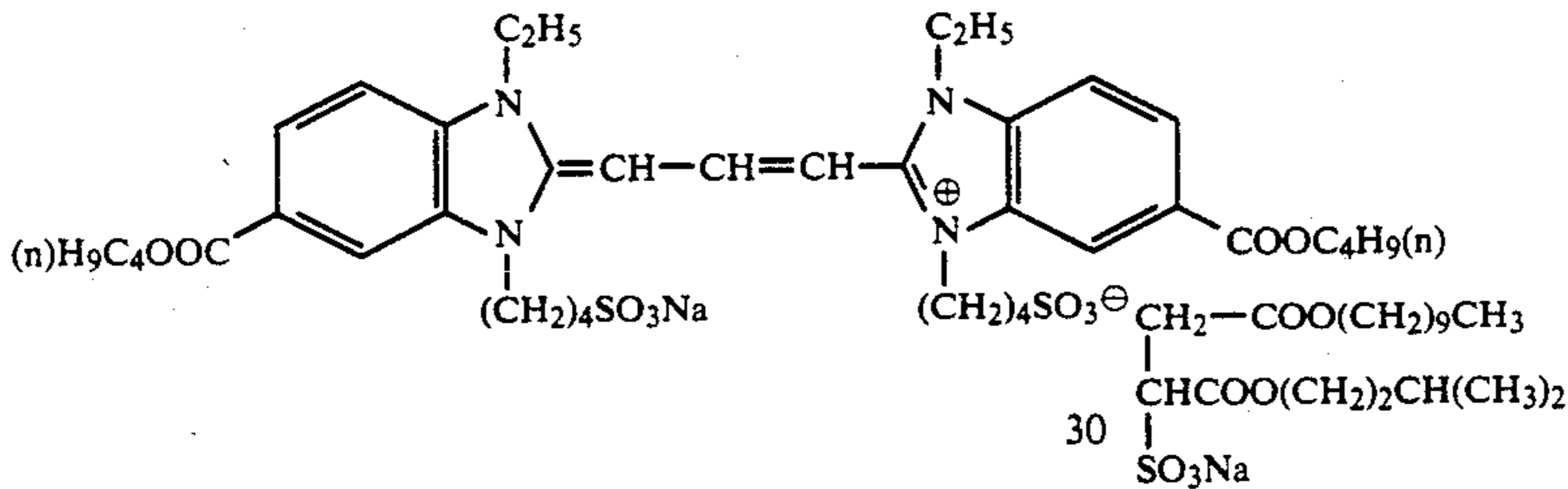
Sensitizing dye (2)
