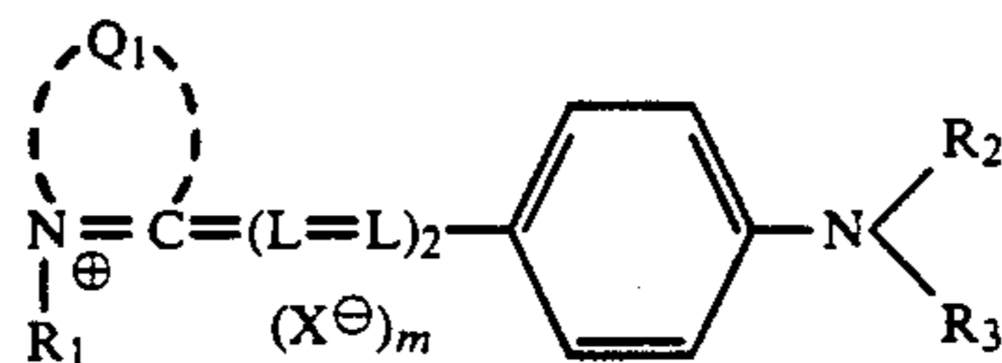
Formula [V]
