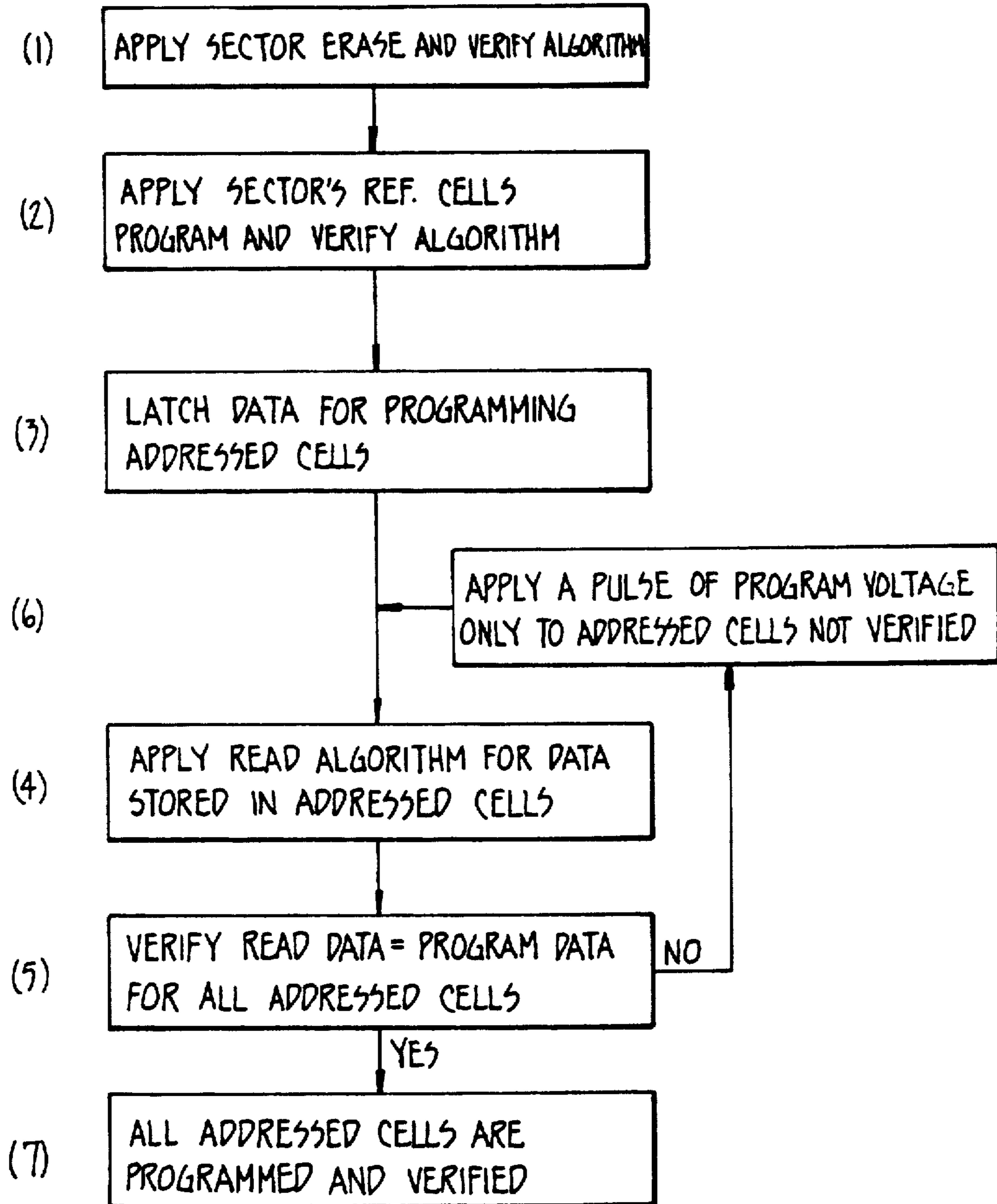
PROGRAM ALGORITHM
