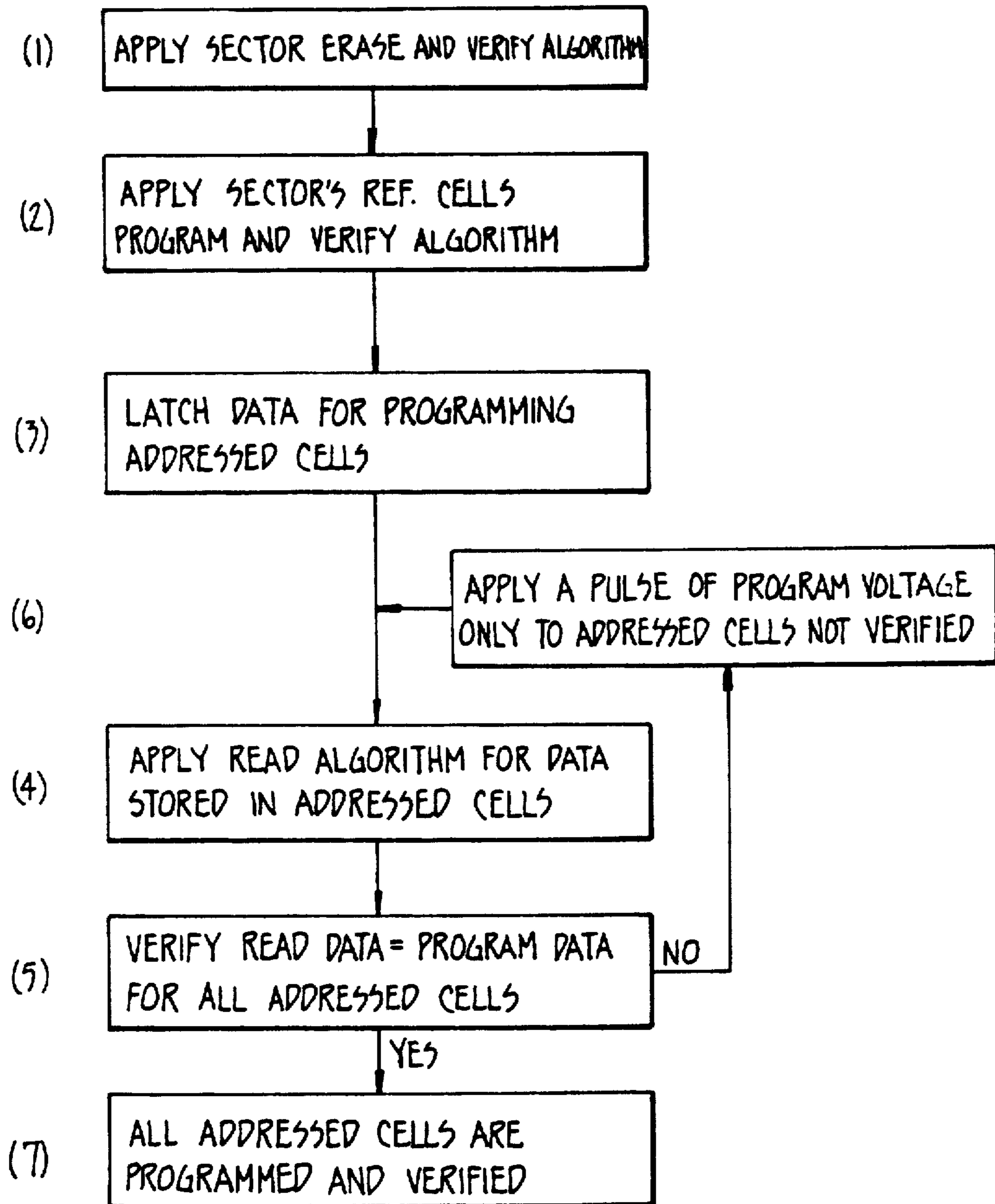
PROGRAM ALGORITHM
