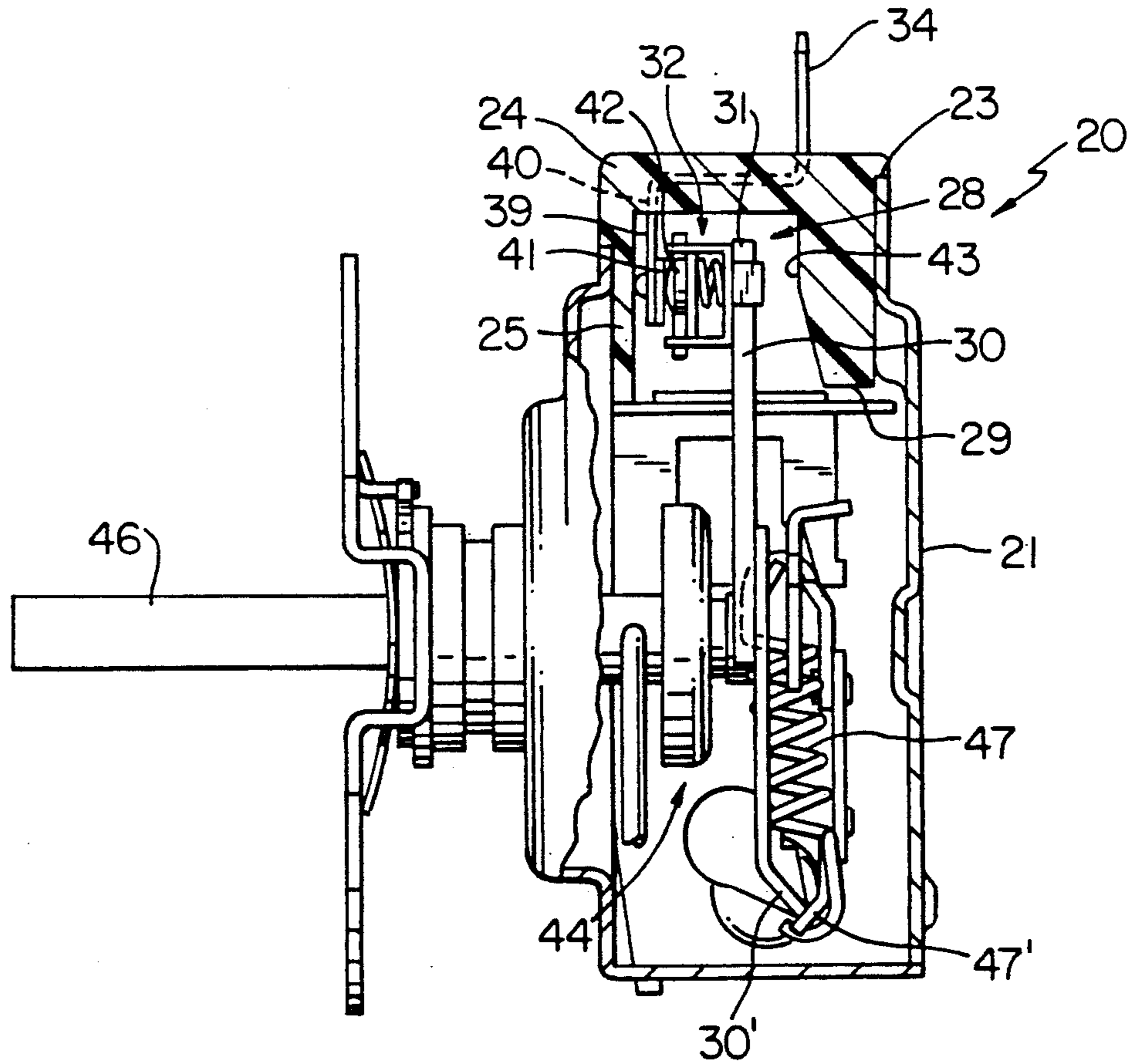
FIG. 2 PRIOR ART
