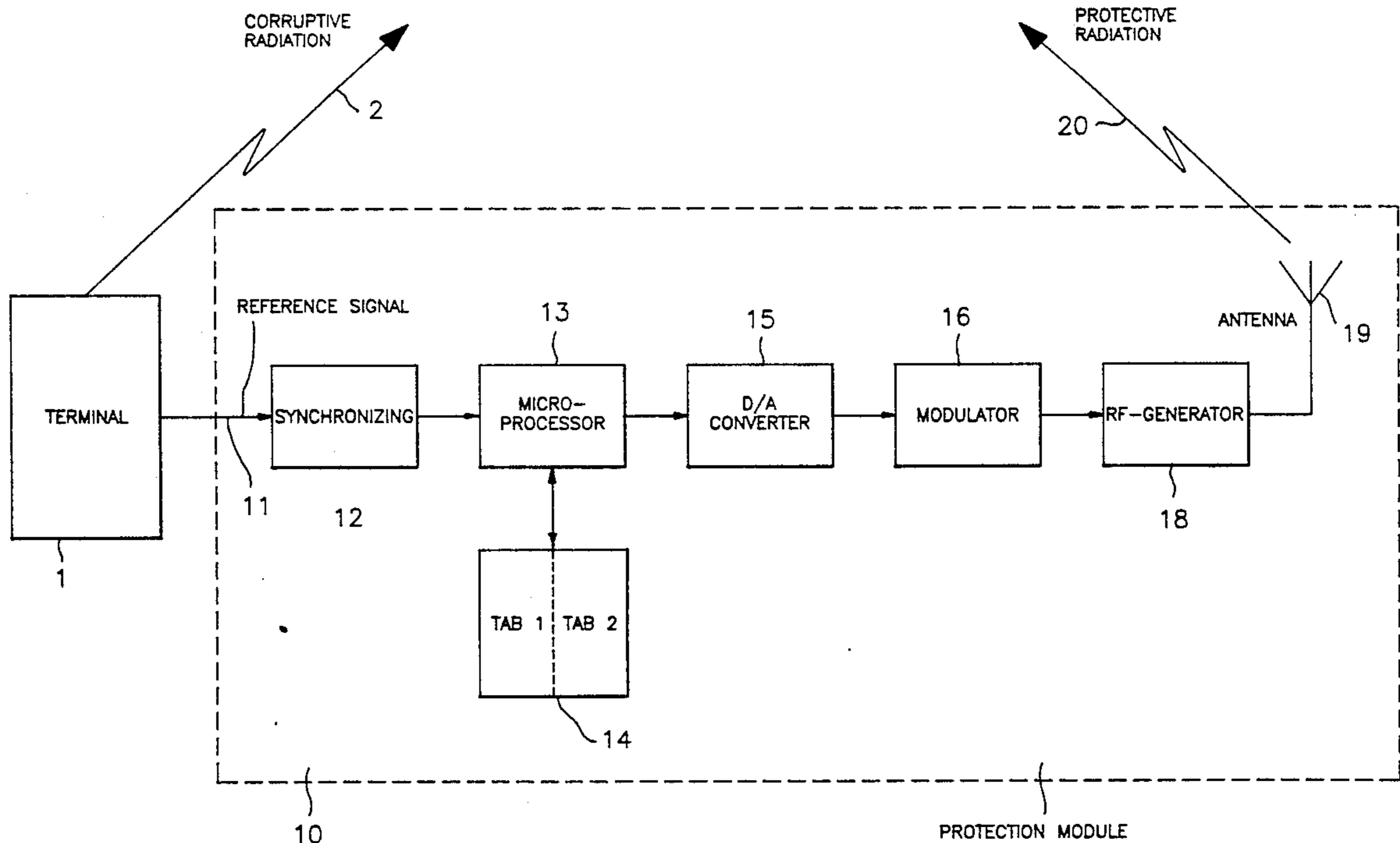
DIAGRAM OF THE PROTECTION MODULE
