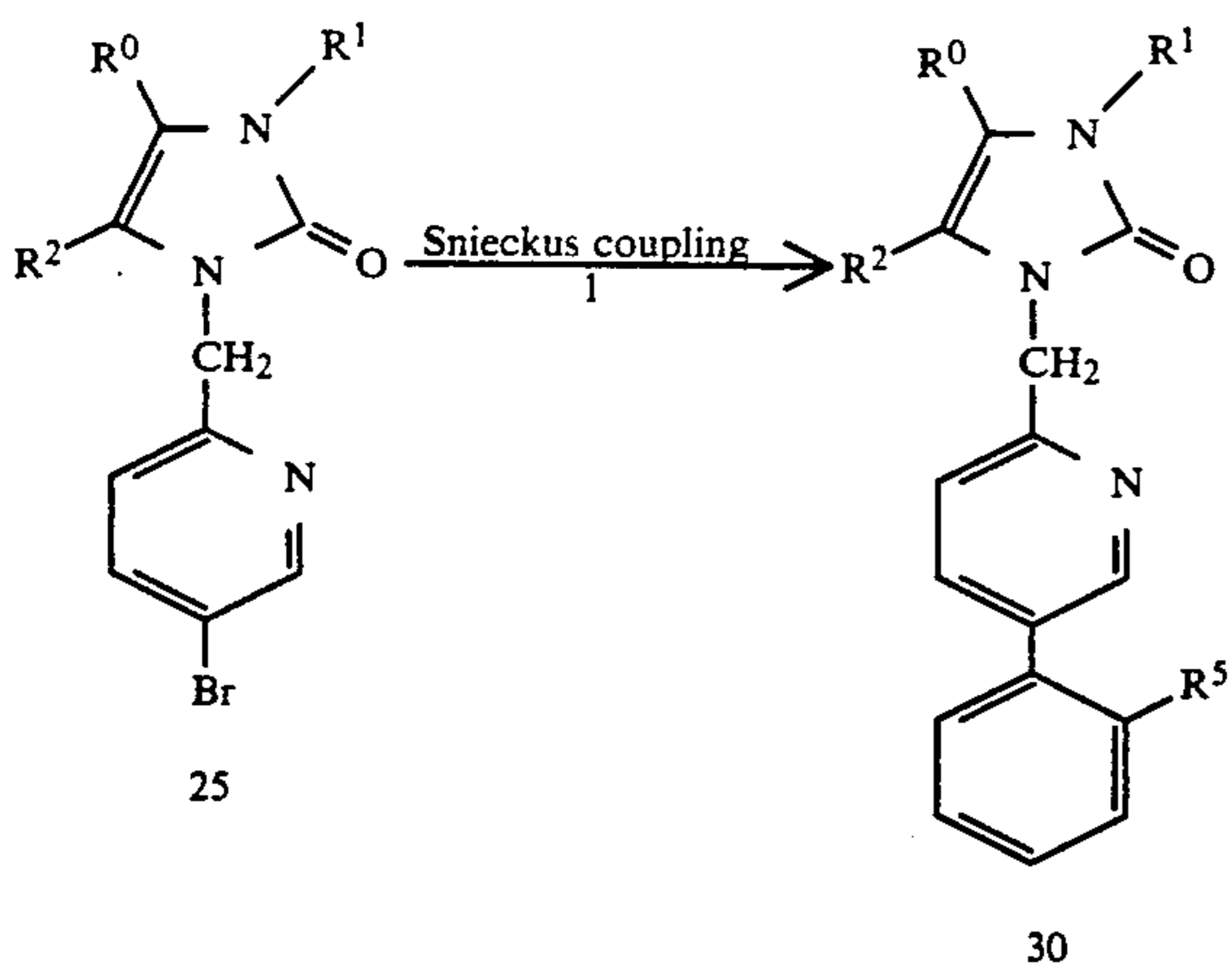
Scheme XIII
