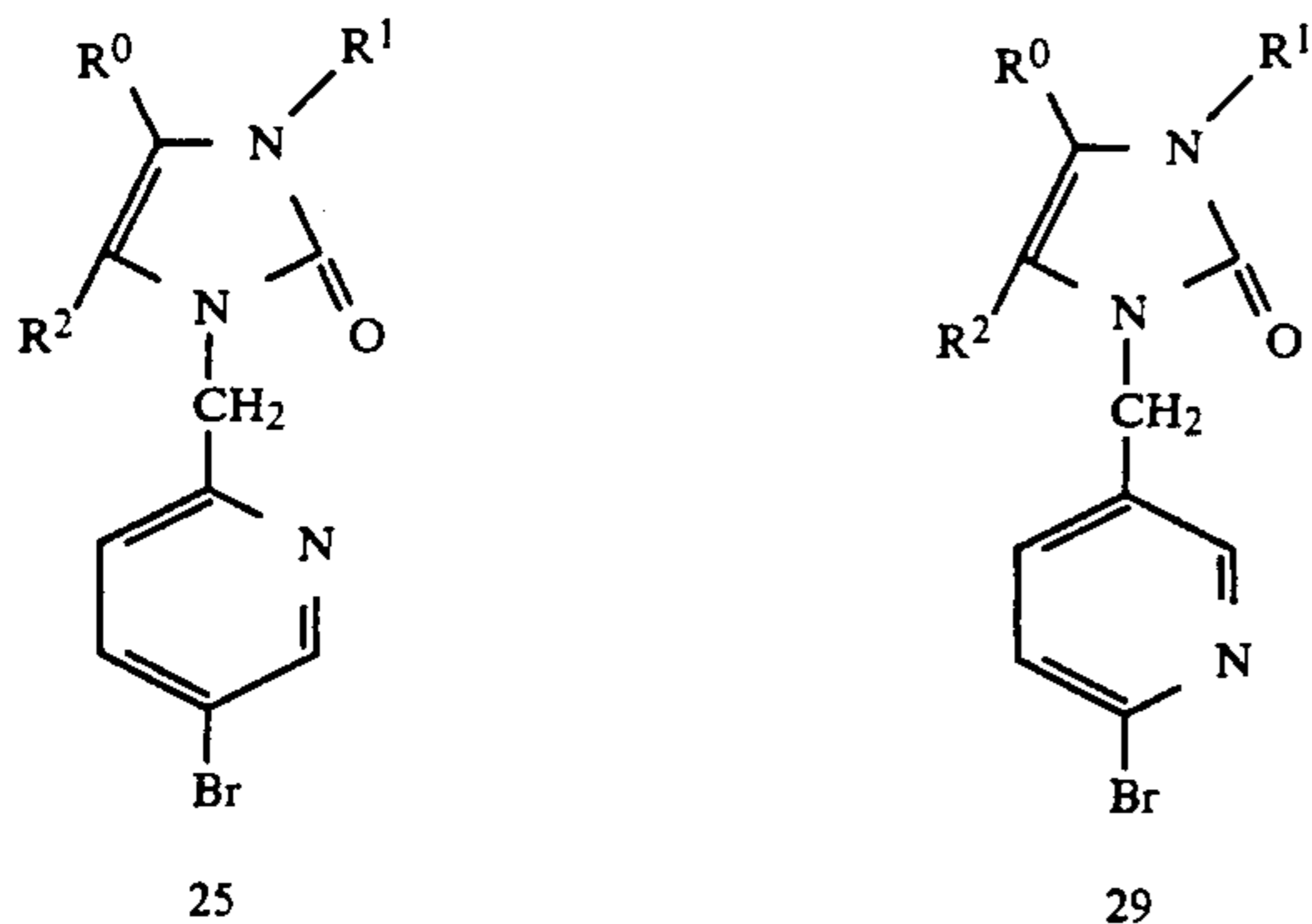
-continued Scheme XII
