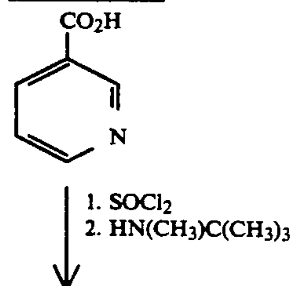
Scheme XVI
