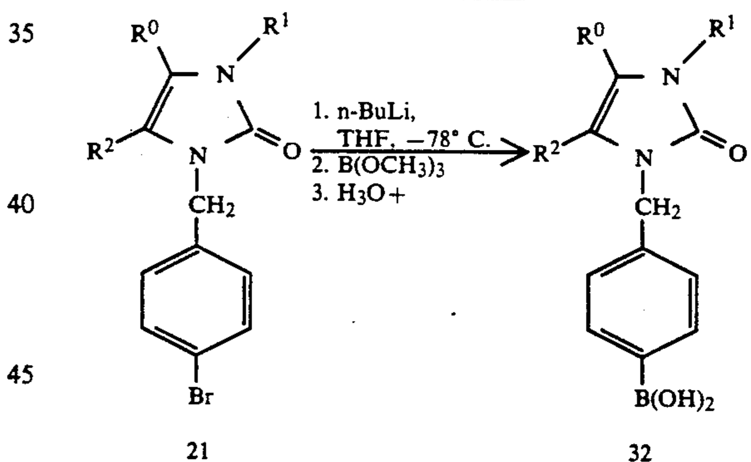
Scheme XV
