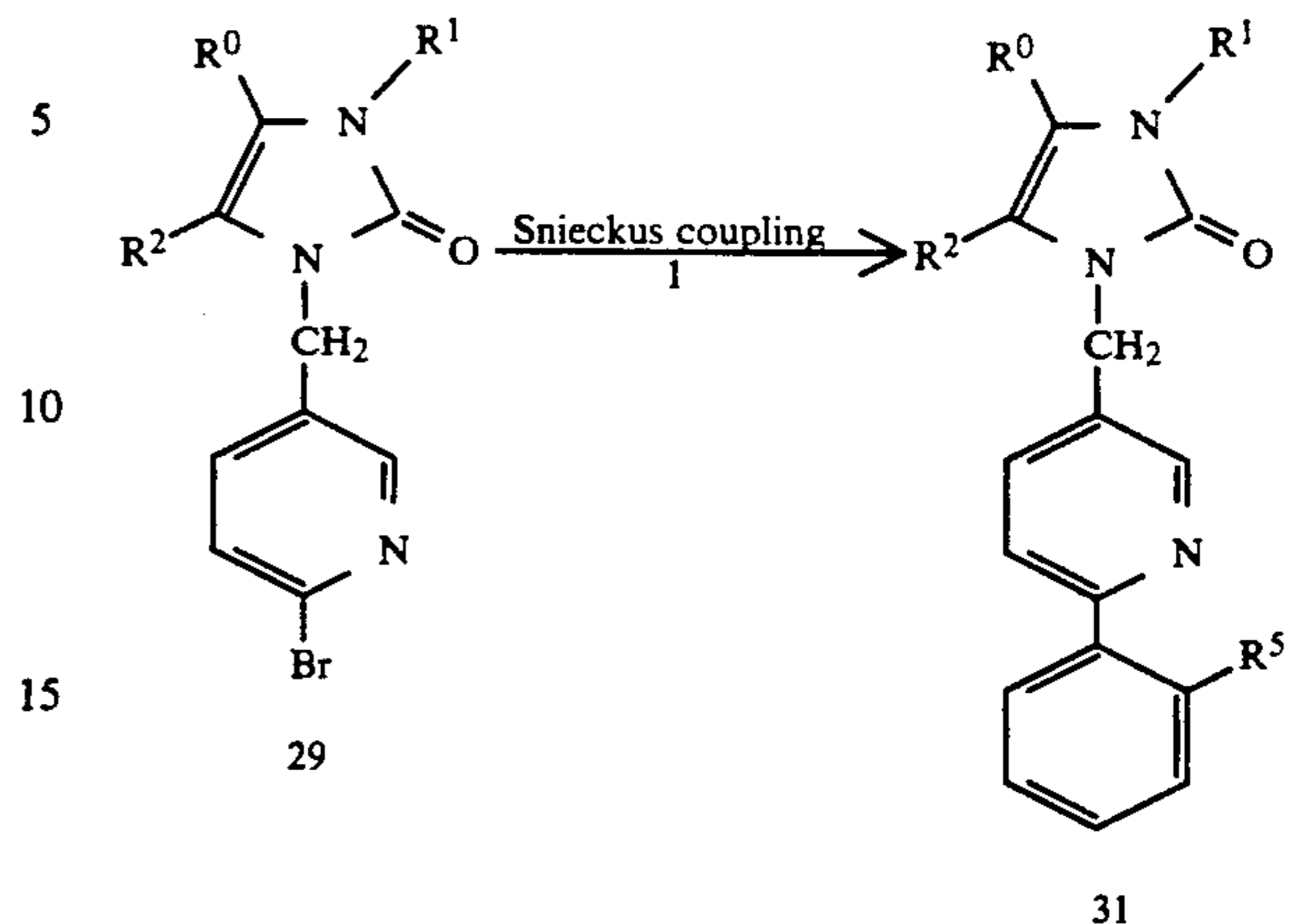
Scheme XIV
