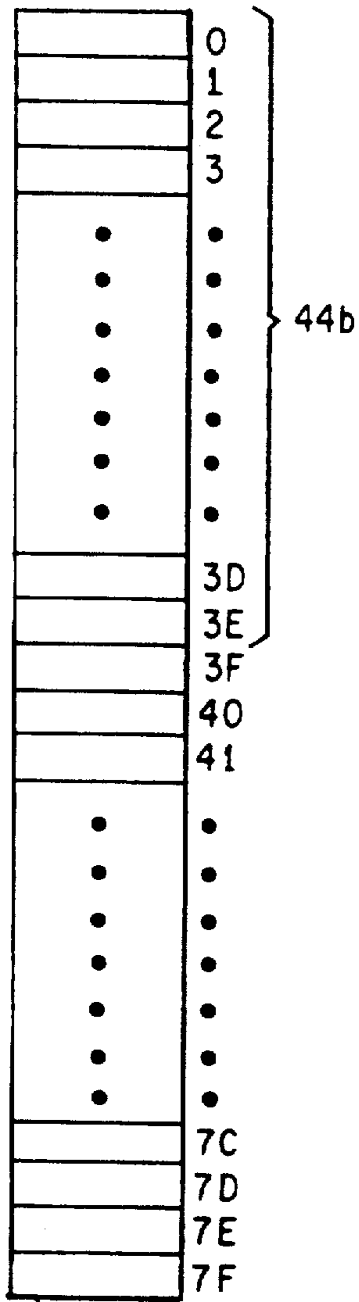
REGISTER FILE 0 OR 1 Fig. 44a
