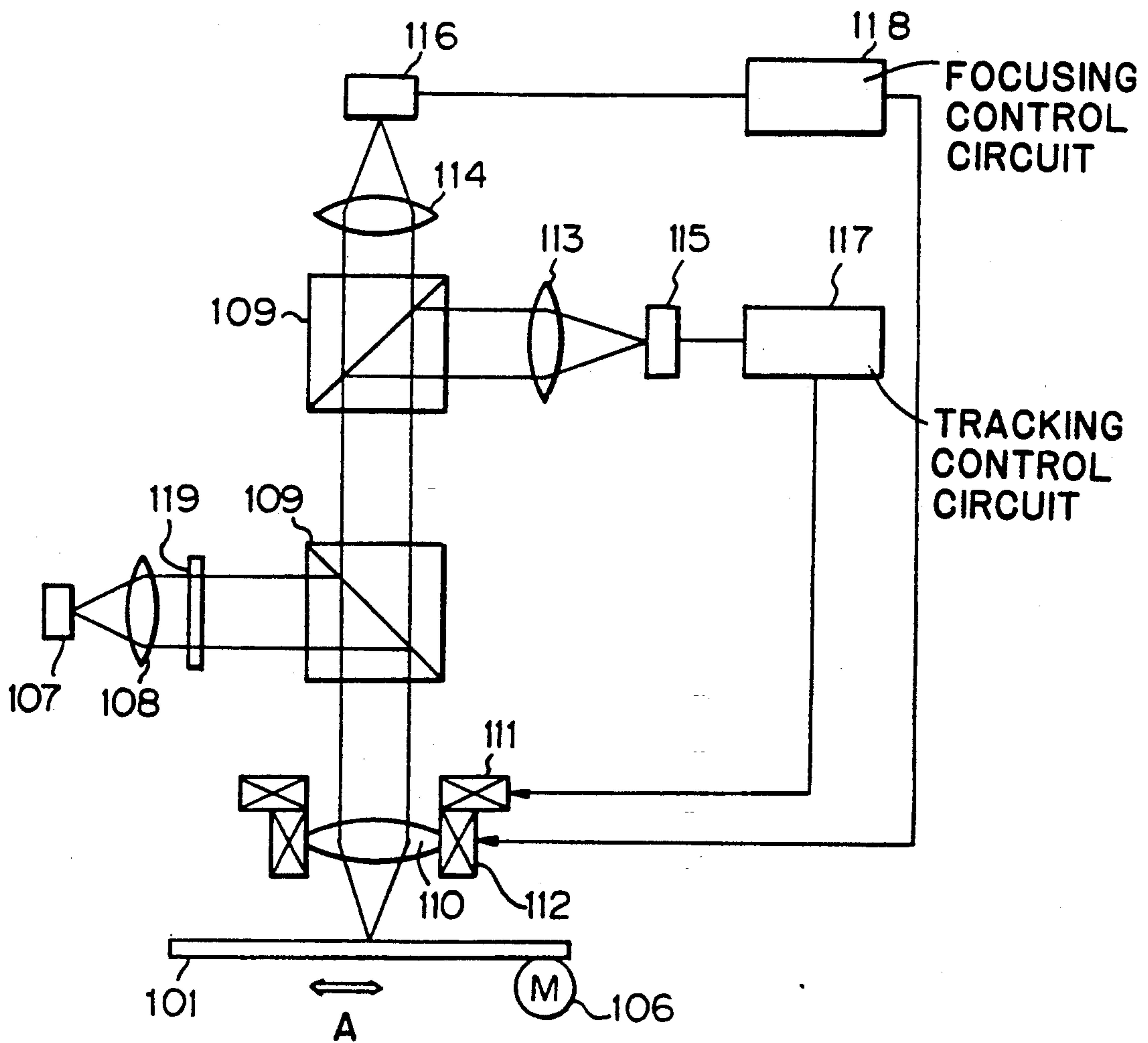
Fig. 2 PRIOR ART
