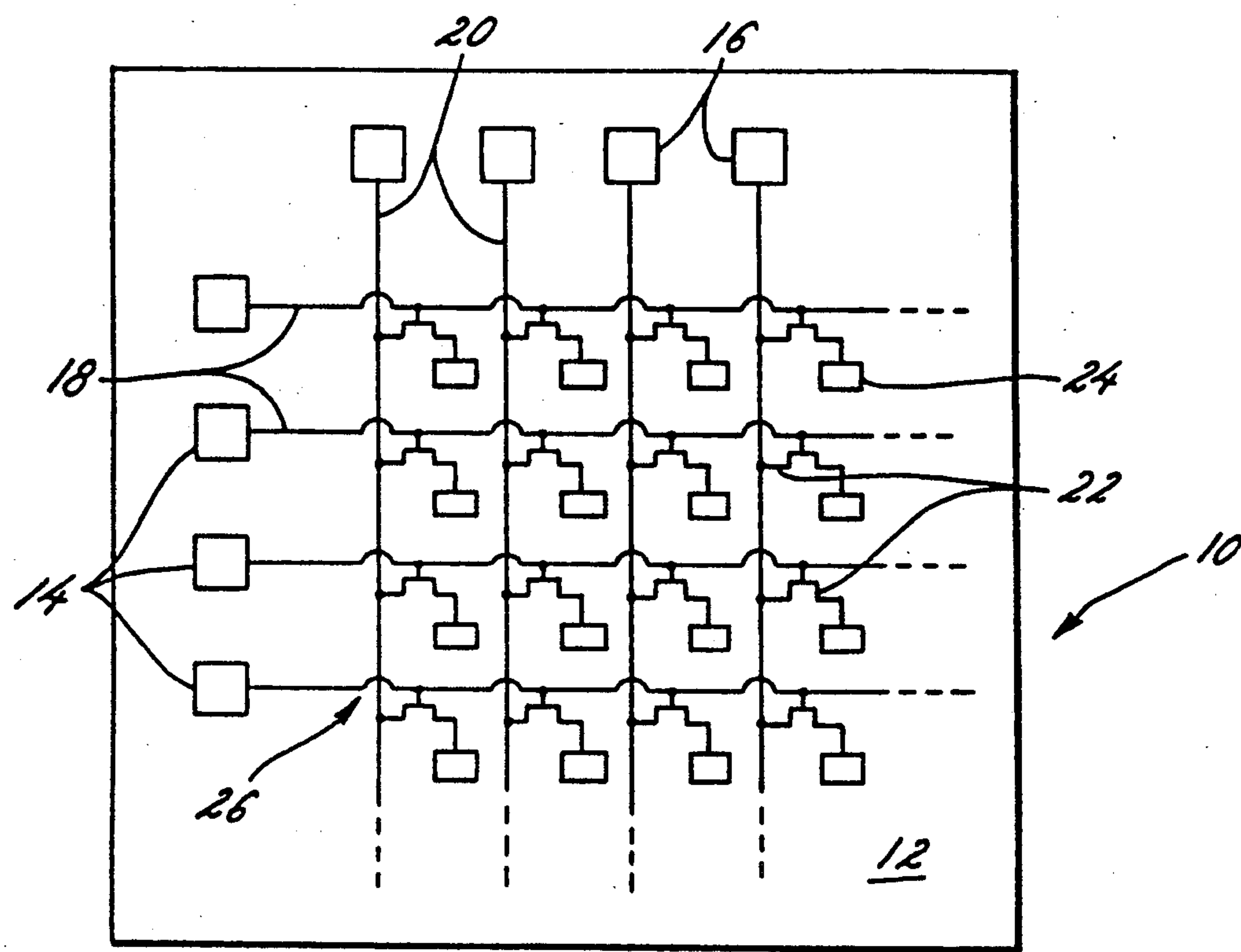
FIG. 1 PRIOR ART
