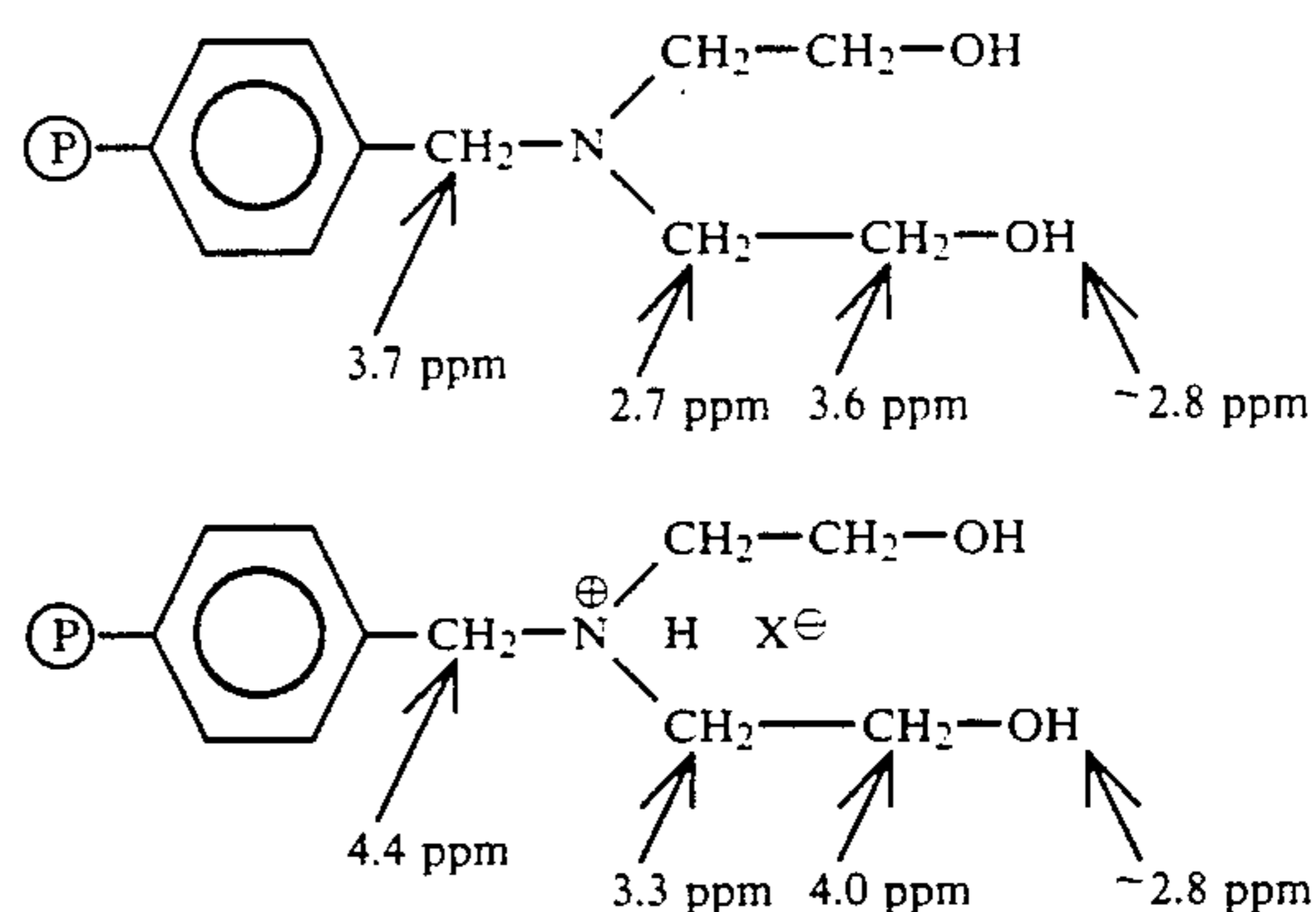
Proton NMR Resonances for Enchained Pendant Functional "mer" Units
