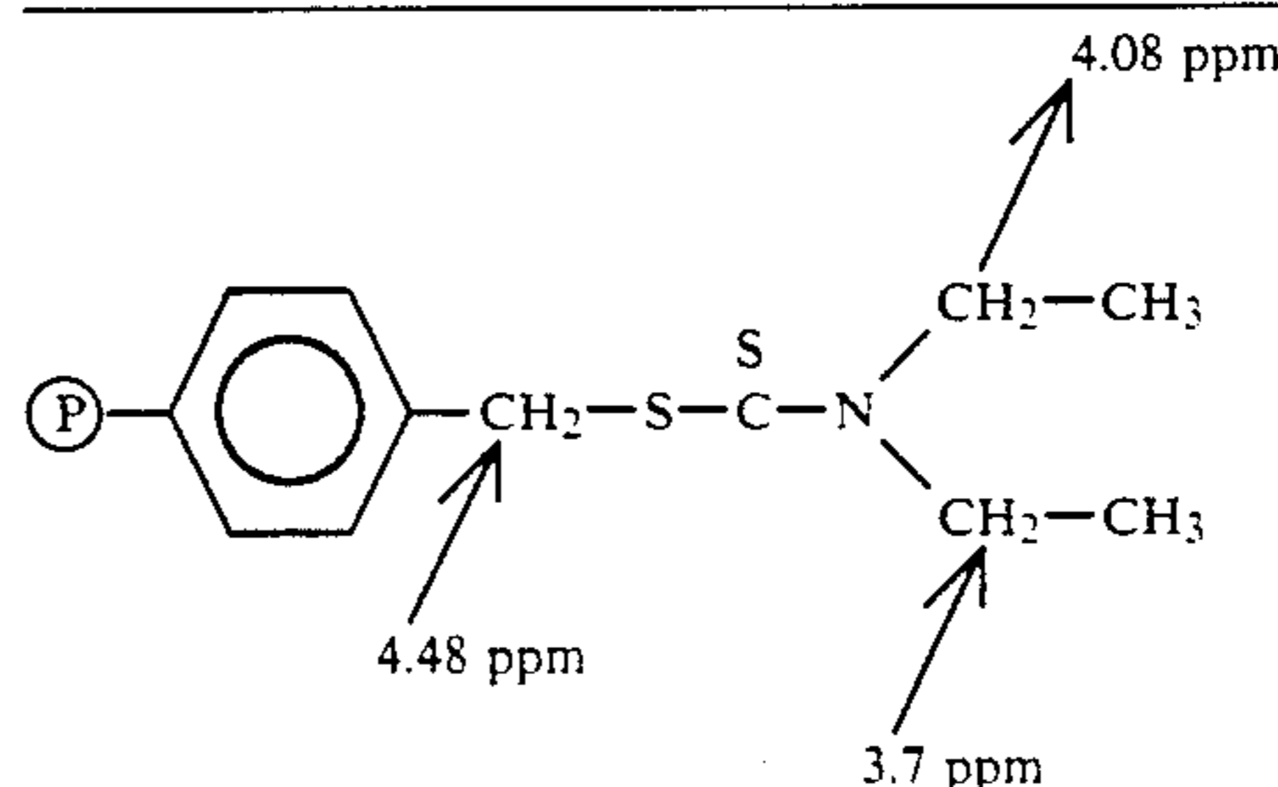
Proton NMR Resonances for Enchained Pendant Functional Dithiocarbamate Ester "Mer" Unit
