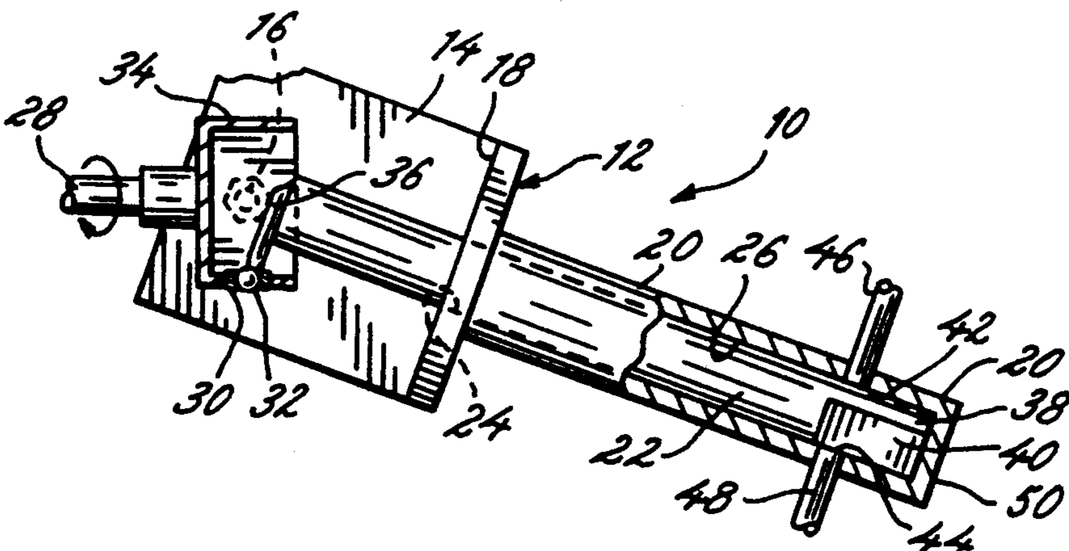
FIG. 1 (PRIOR ART)
