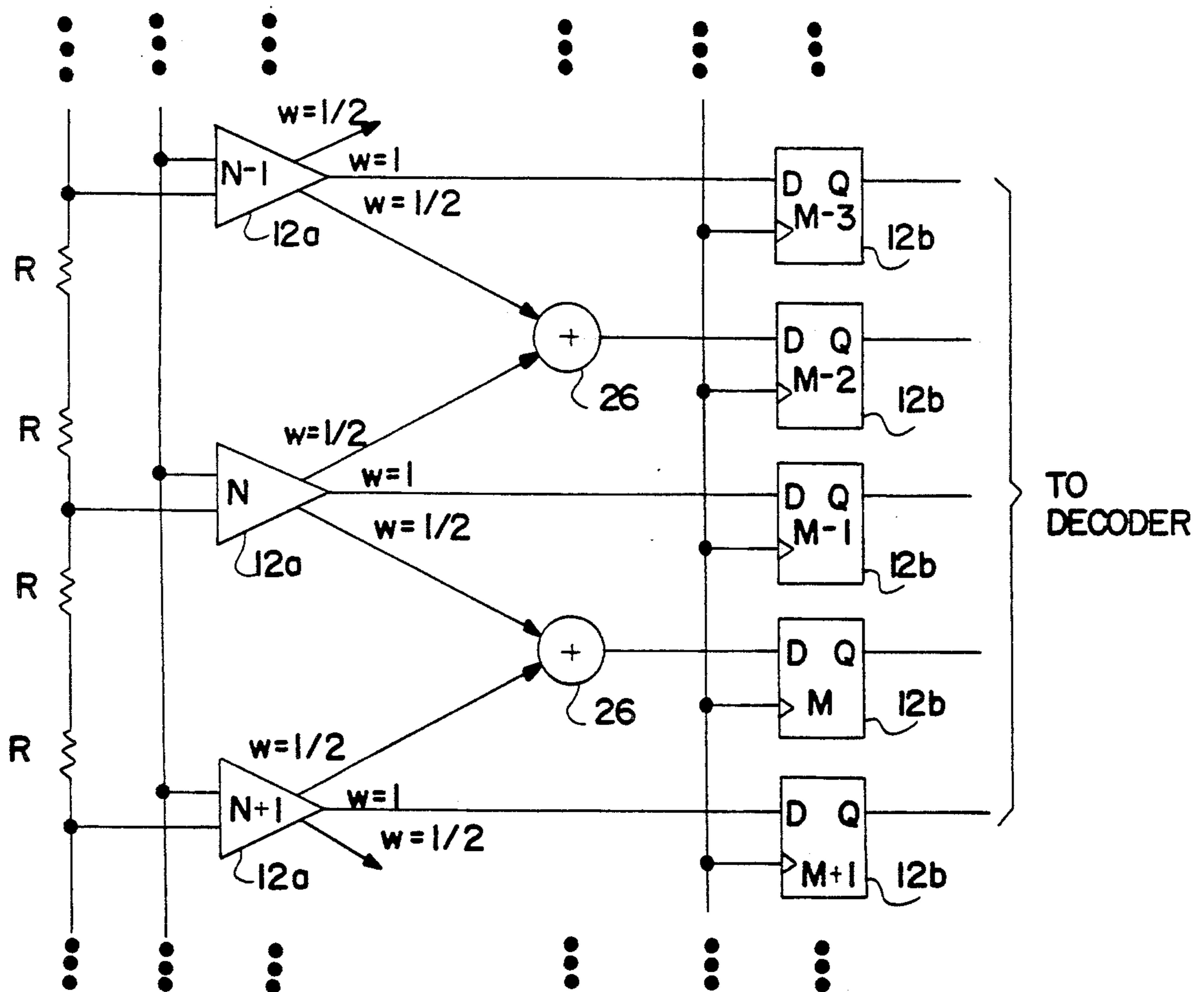
FIG. 3 (PRIOR ART)
