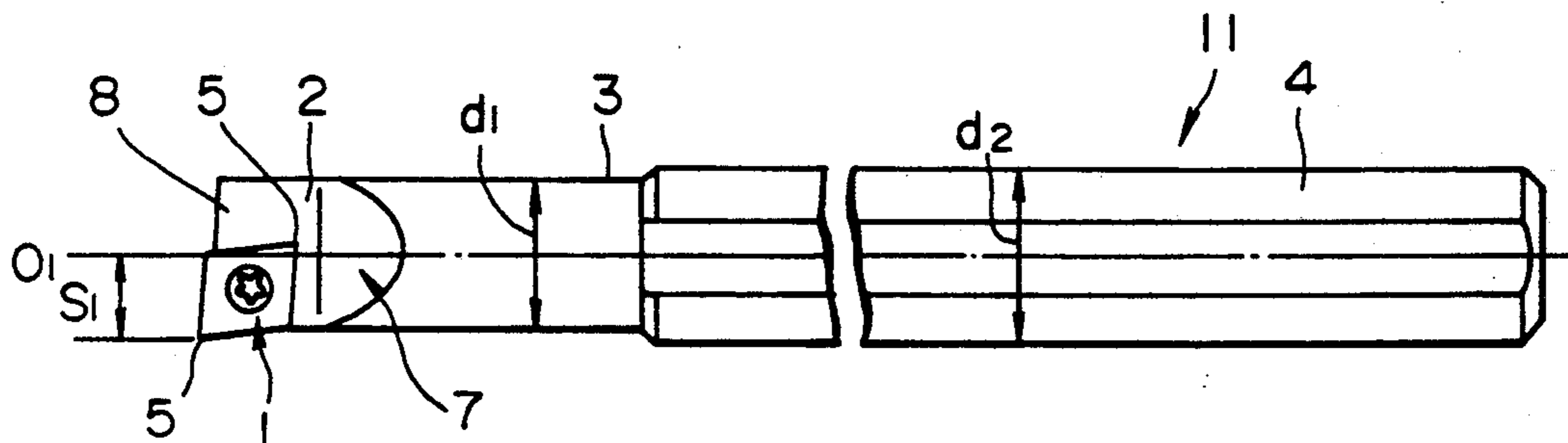
FIG. 48 (PRIOR ART)
