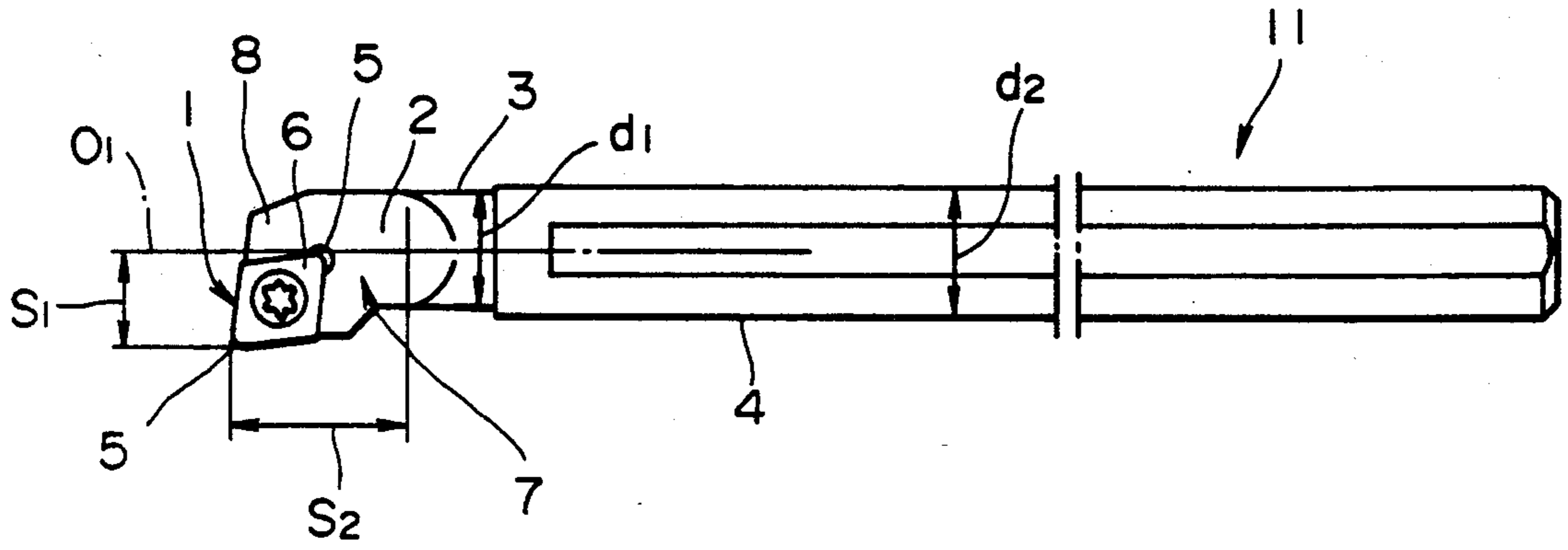
FIG. 52 (PRIOR ART)
