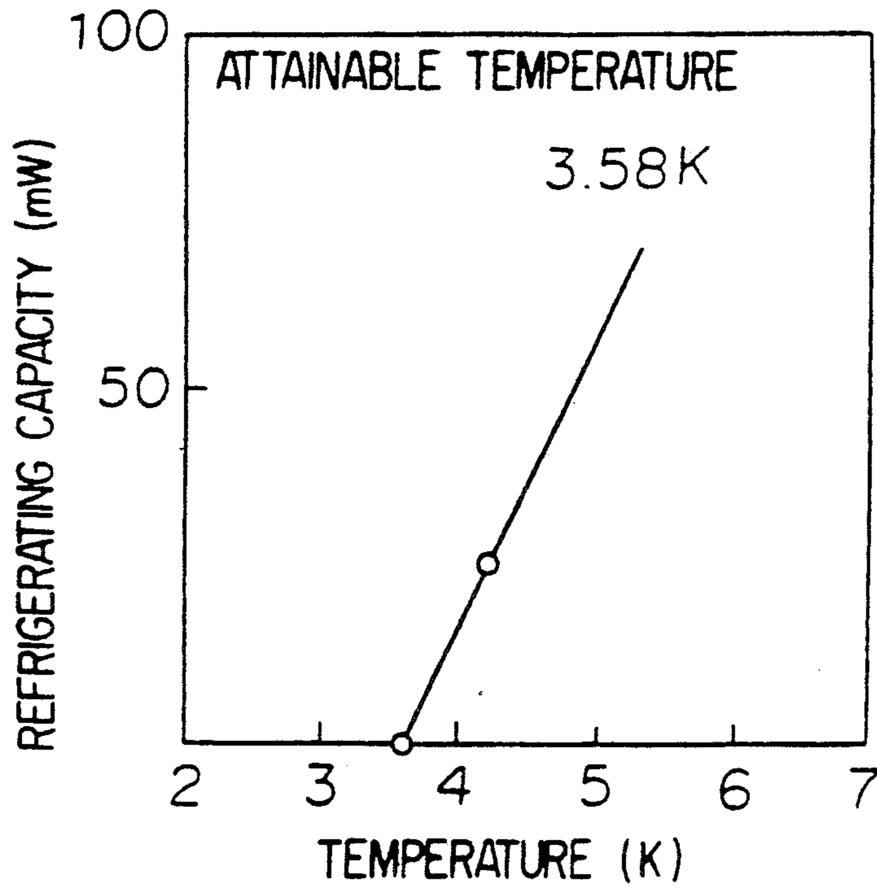
REFRIGERATION CAPACITY OF THREE-STAGE GM REFRIGERATOR
