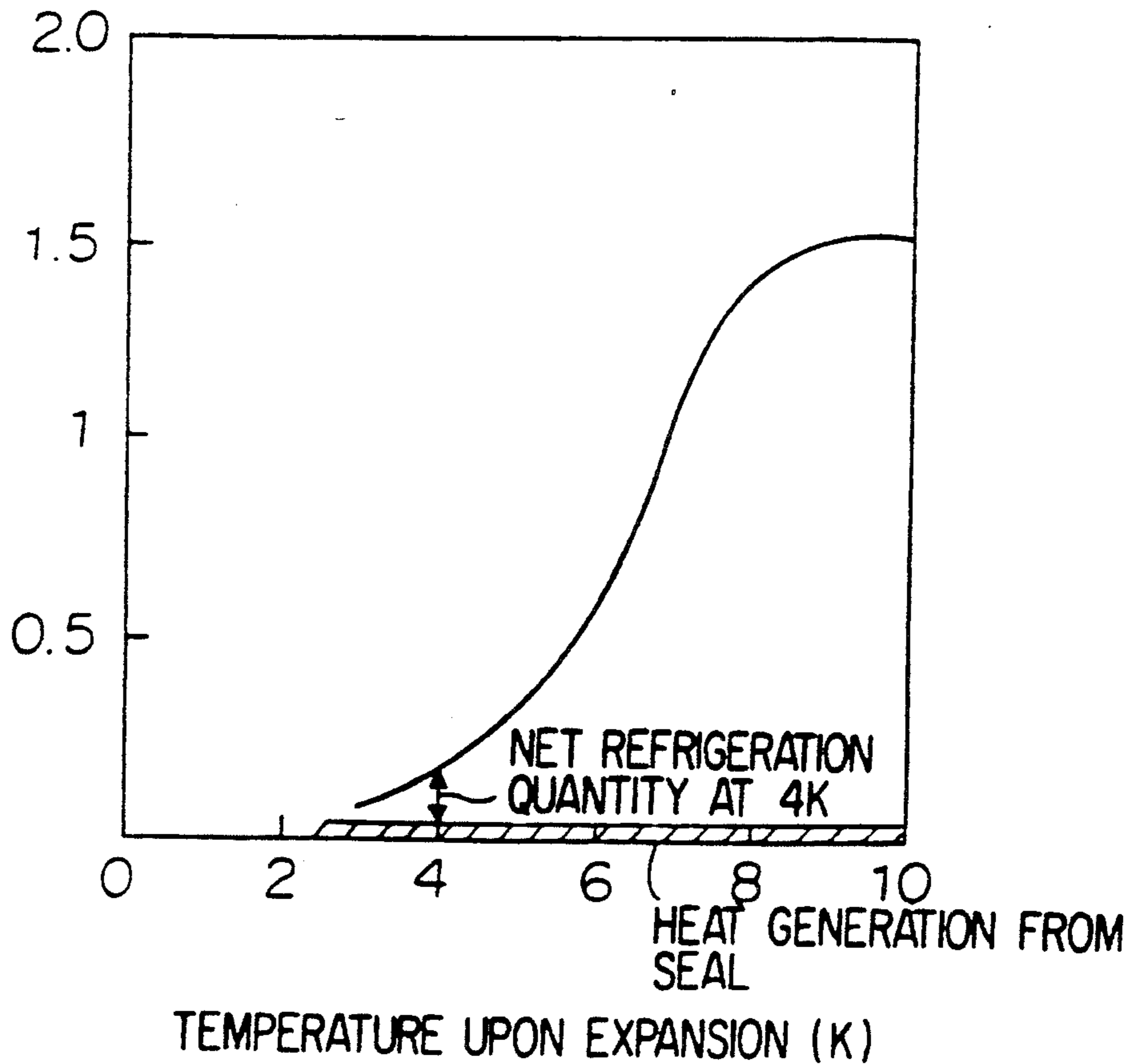
THEORETICAL GENERATED REFRIGERATION QUANTITY / INDICATED REFRIGERATION QUANTITY
