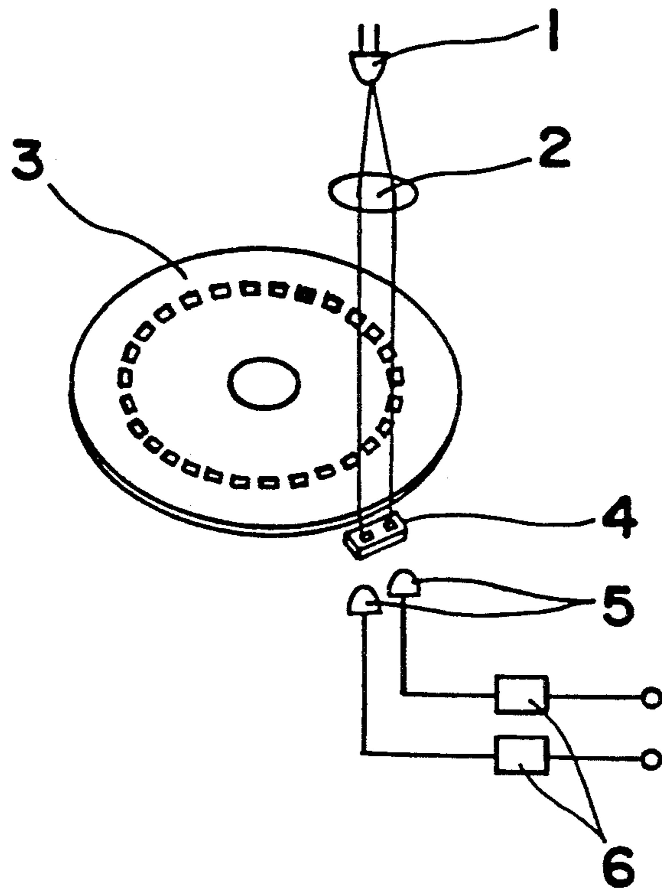
Fig. 1 PRIOR ART
