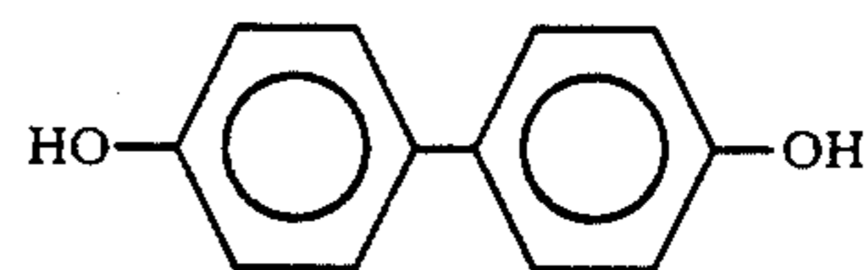
4,4'-Dihydroxybiphenyl (DHBP):
