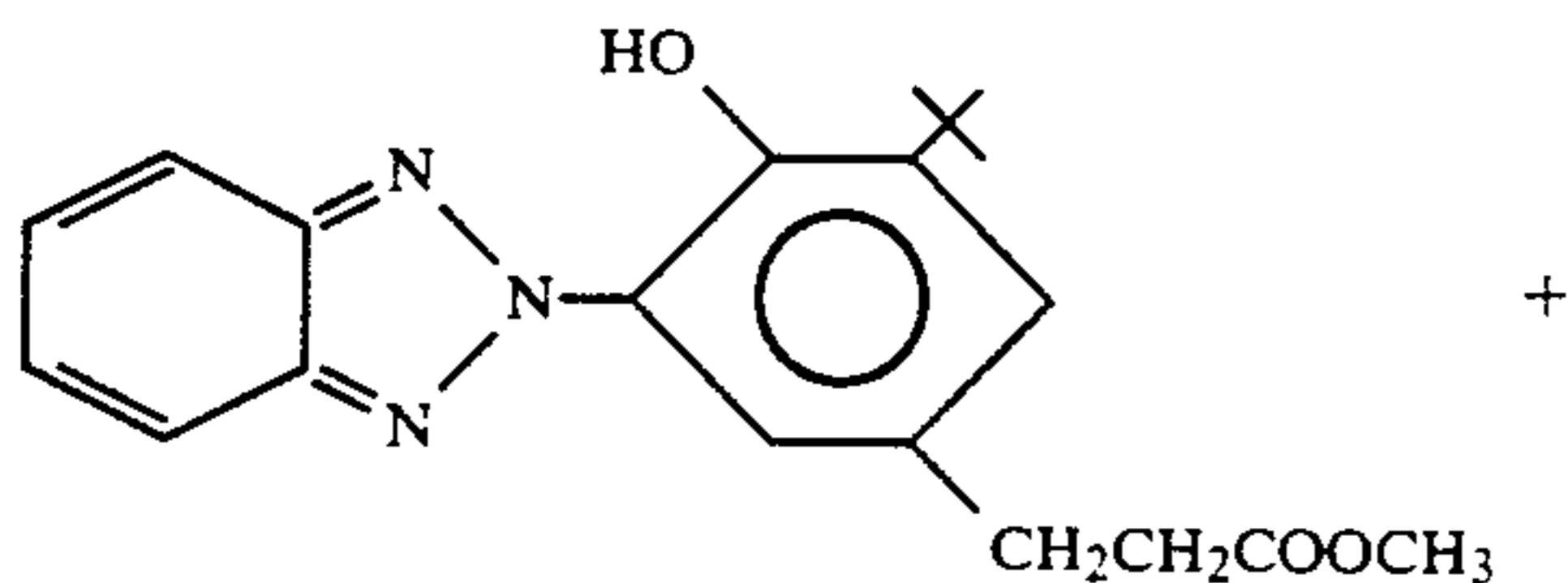
methyl-3-(3-(2H-benzotriazol-2-yl)-5-tert.butyl-4-hydroxyphenyl)propionate
