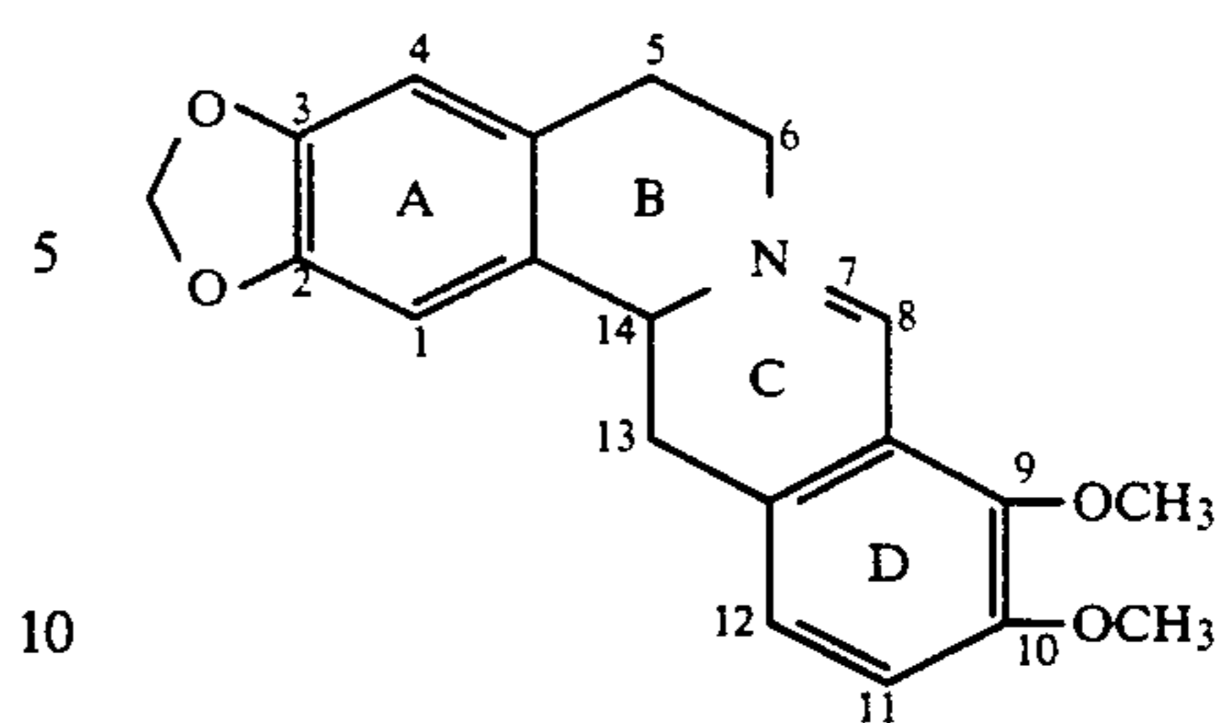
(-)-CANADINE ((-)-TETRAHYDROBERBERINE)
