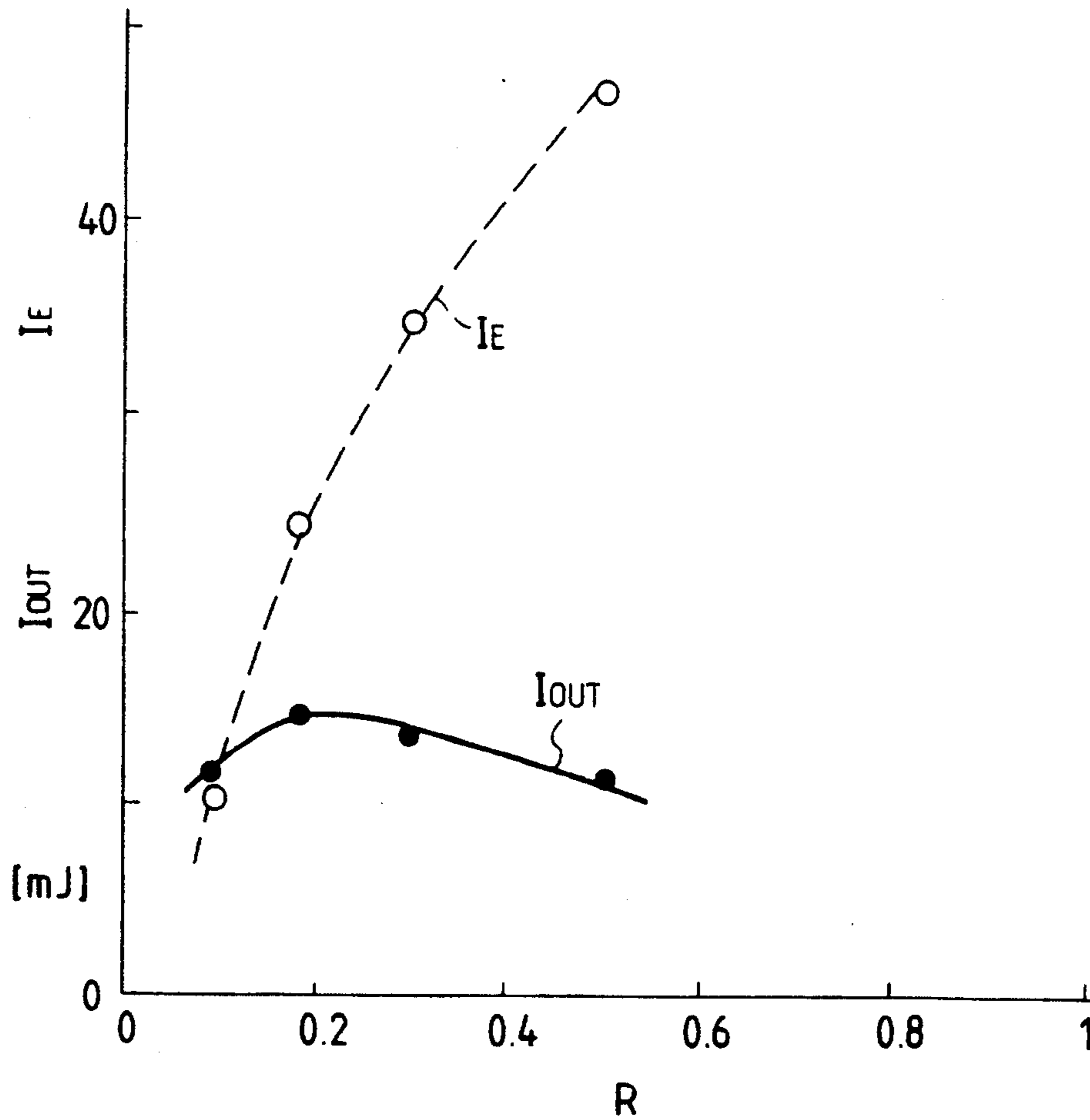
FIG. 8 PRIOR ART
