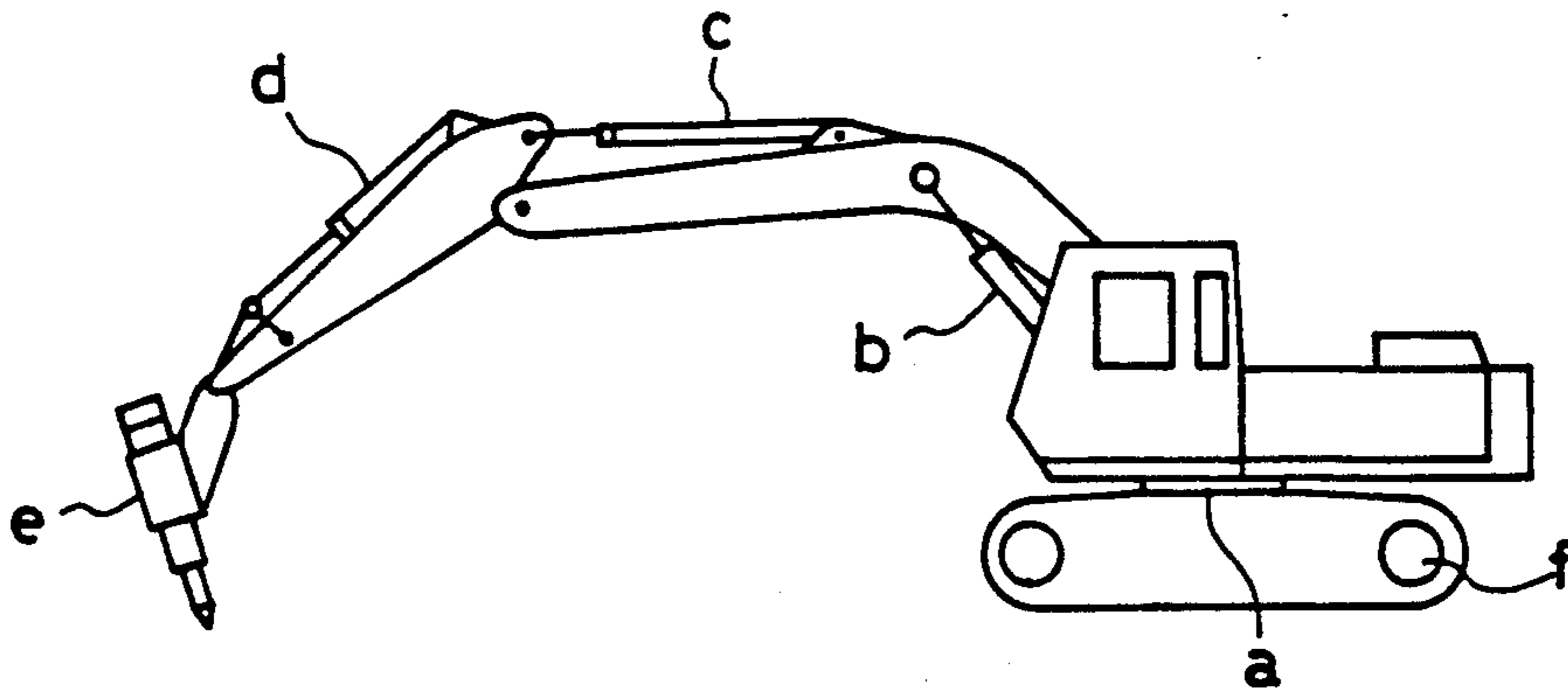
FIG. 3 (PRIOR ART)
