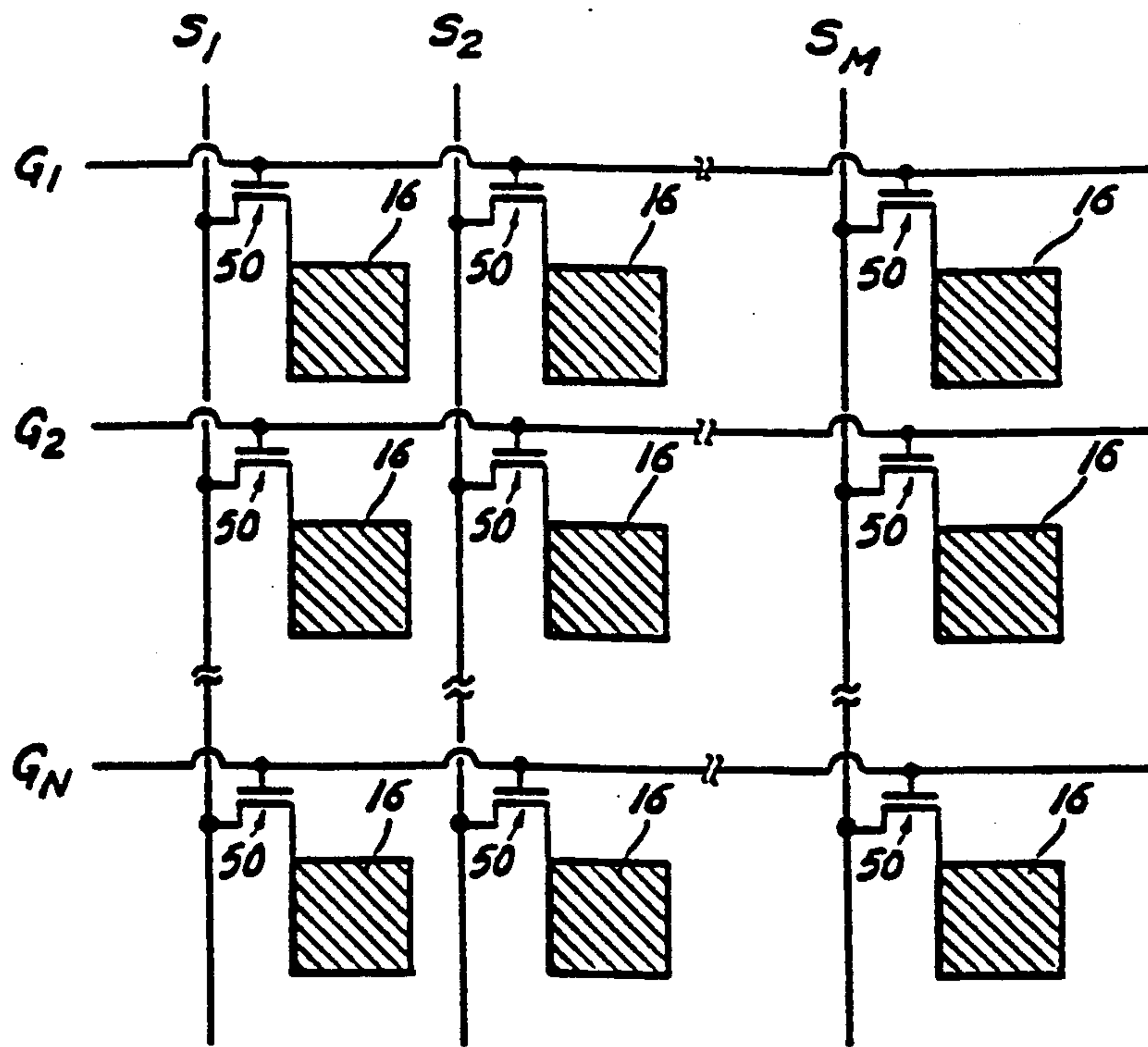
Fig. 1 (Prior Art)
