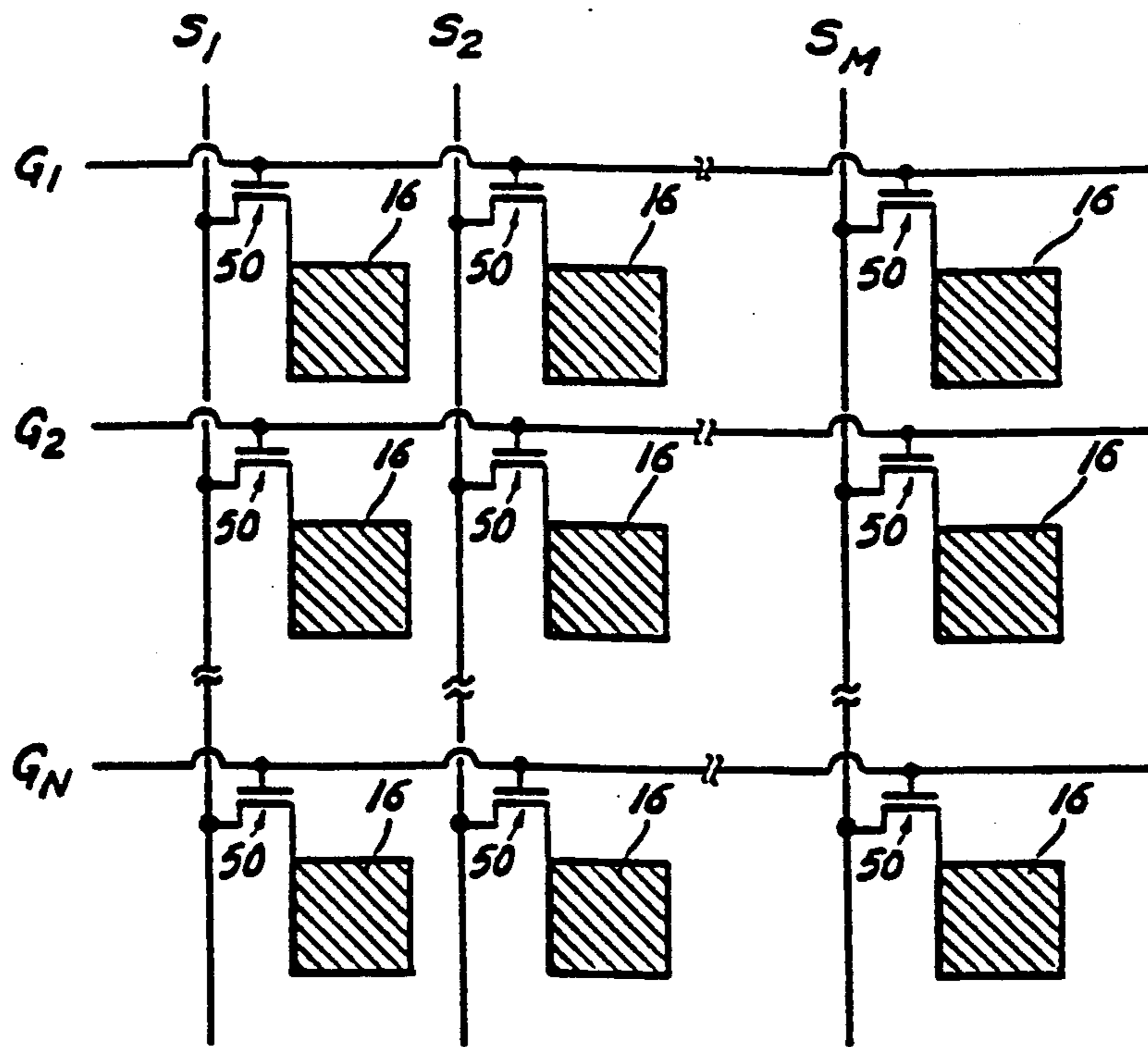
Fig. 1 (Prior Art)
