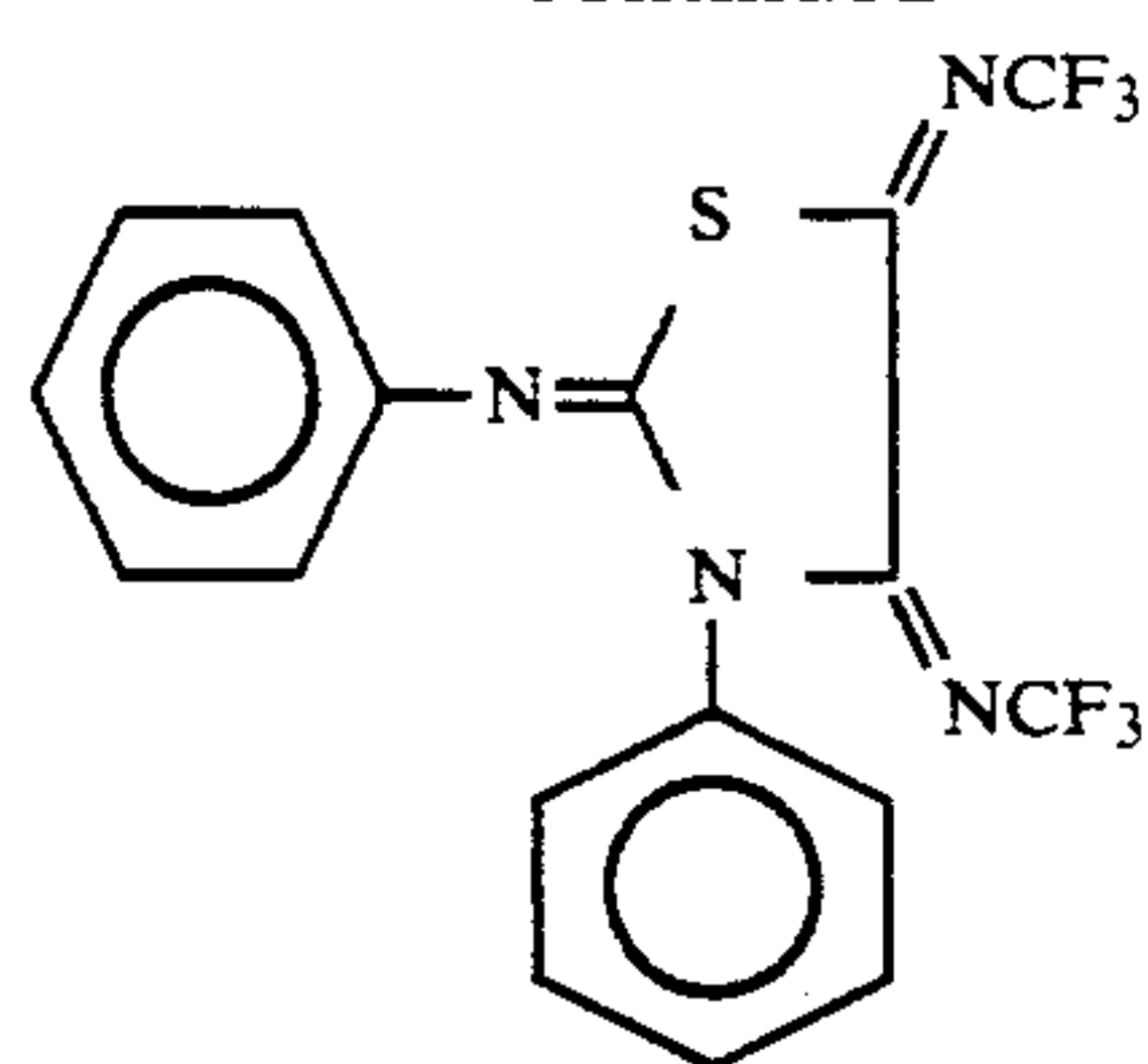
(FLUOBENZIMINE)
