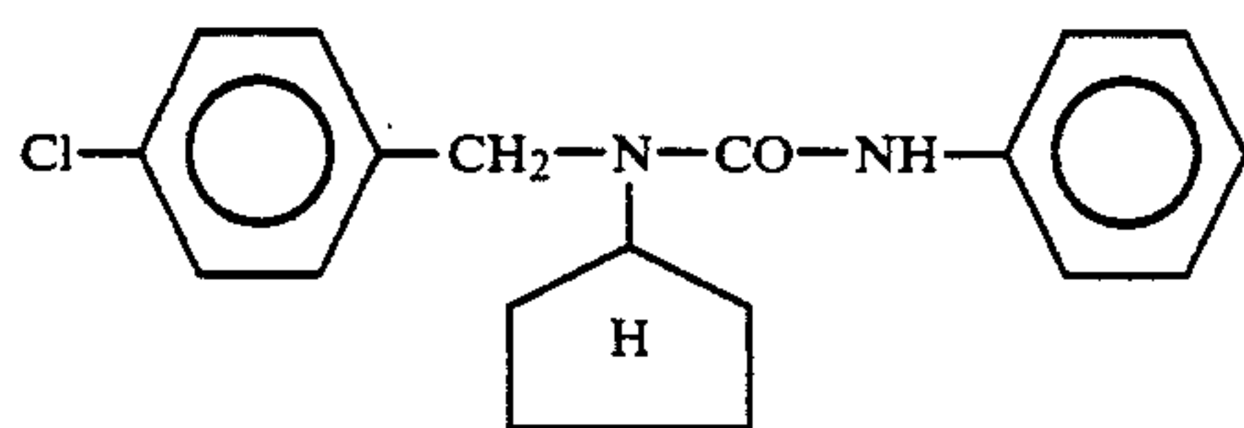
(PENCYCURON)
