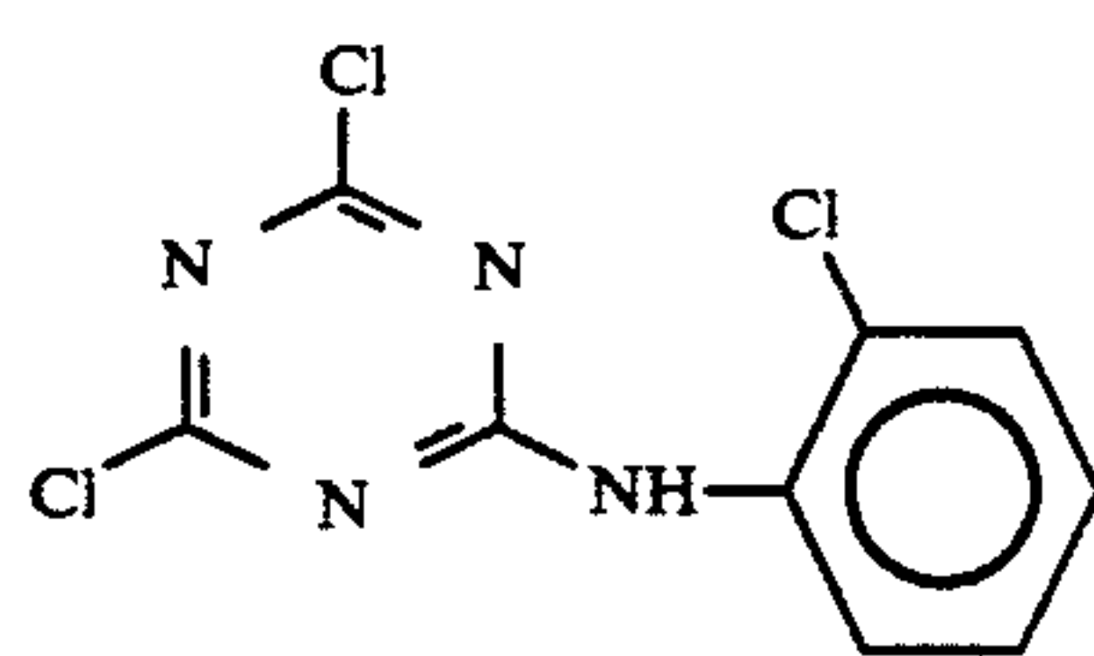
(ANILAZINE)
