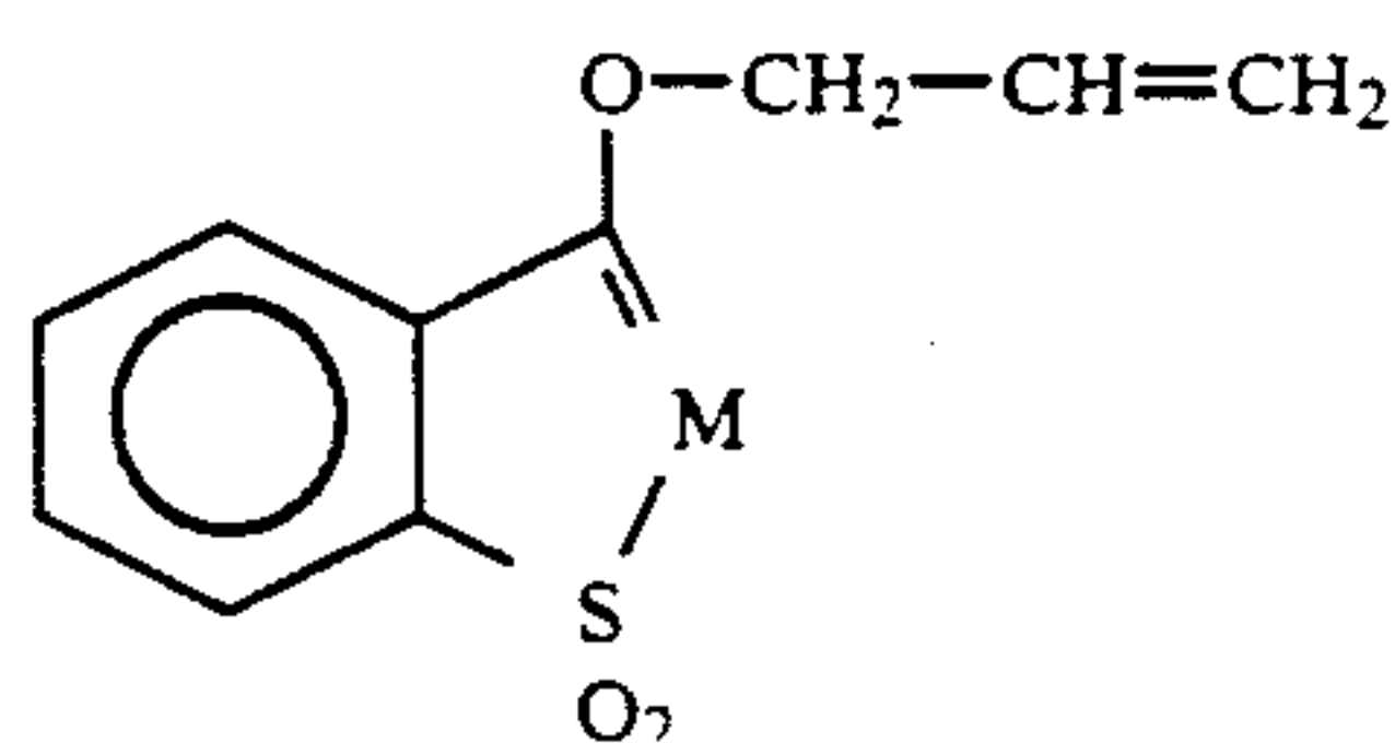
(PROBENAZOLE)
