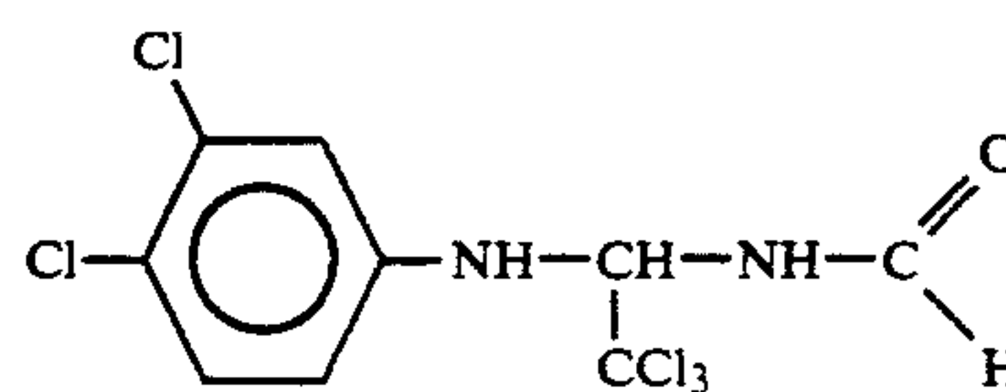
(CHLORANIFORMETHANE)
