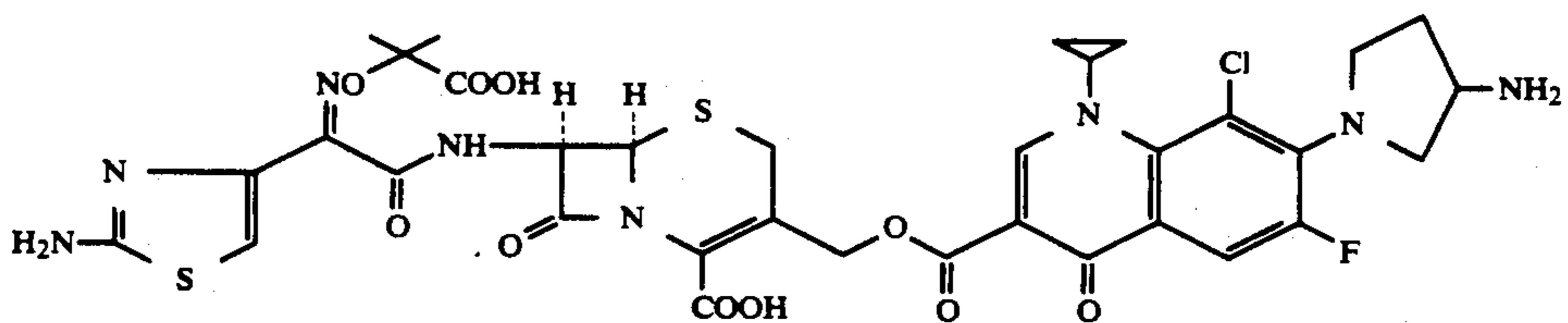
thyl]-8-oxo-5-thia-1-azabicyclo[4.2.0]oct-2-en-7-yl]amino]carbonyl]benzeneacetic acid
