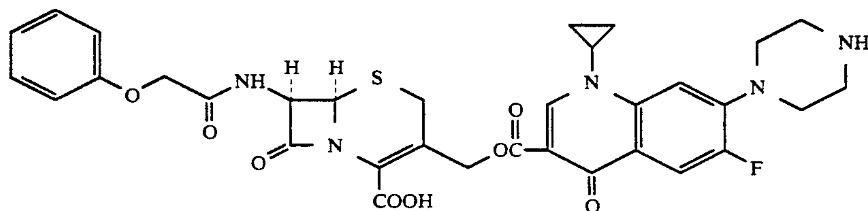
[6R-[6 \alpha ,7 \beta (Z)]]-7-[[[(2-amino-4-thiazolyl)methoxyimino]acetyl]amino]-3-[[[1-cyclopropyl-6-fluoro-1,4-dihydro-4-oxo-7-(1-piperazinyl)-3-quinoliny]carbonyl]oxy]methyl]-8-oxo-5-thia-1-azabicyclo[4.2.0]oct-2-ene-2-carboxylic acid
