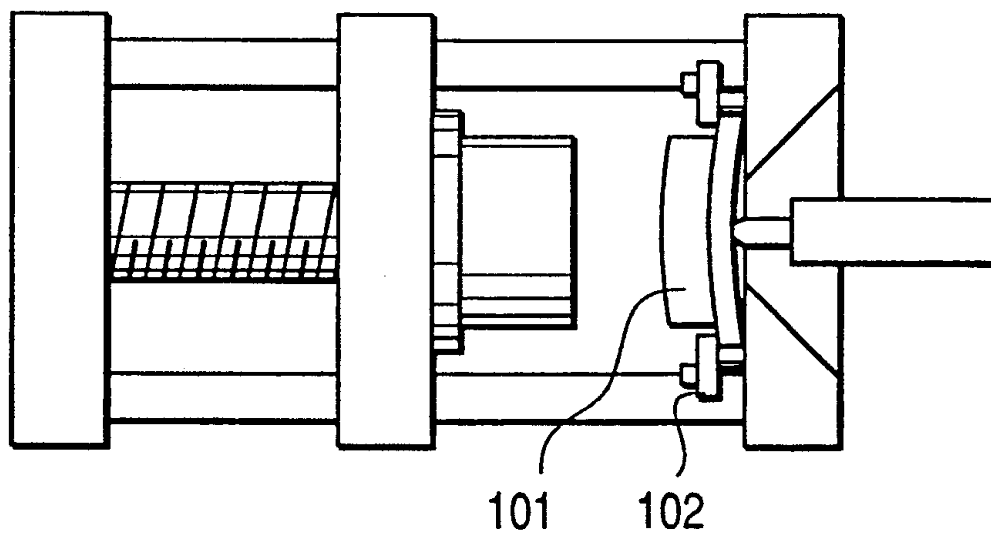
FIG. 3 PRIOR ART
