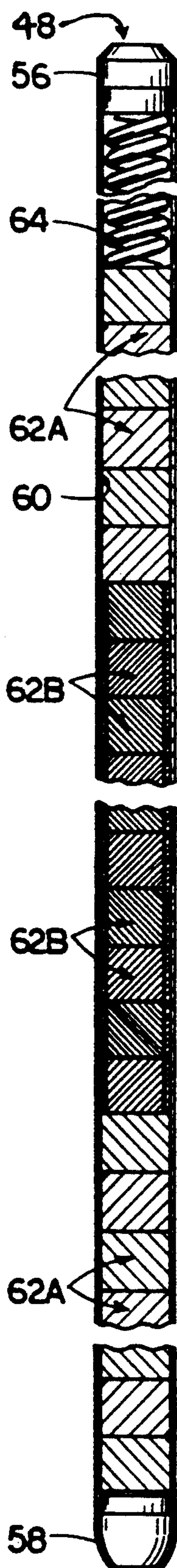
FIG. 4 (PRIOR ART)
