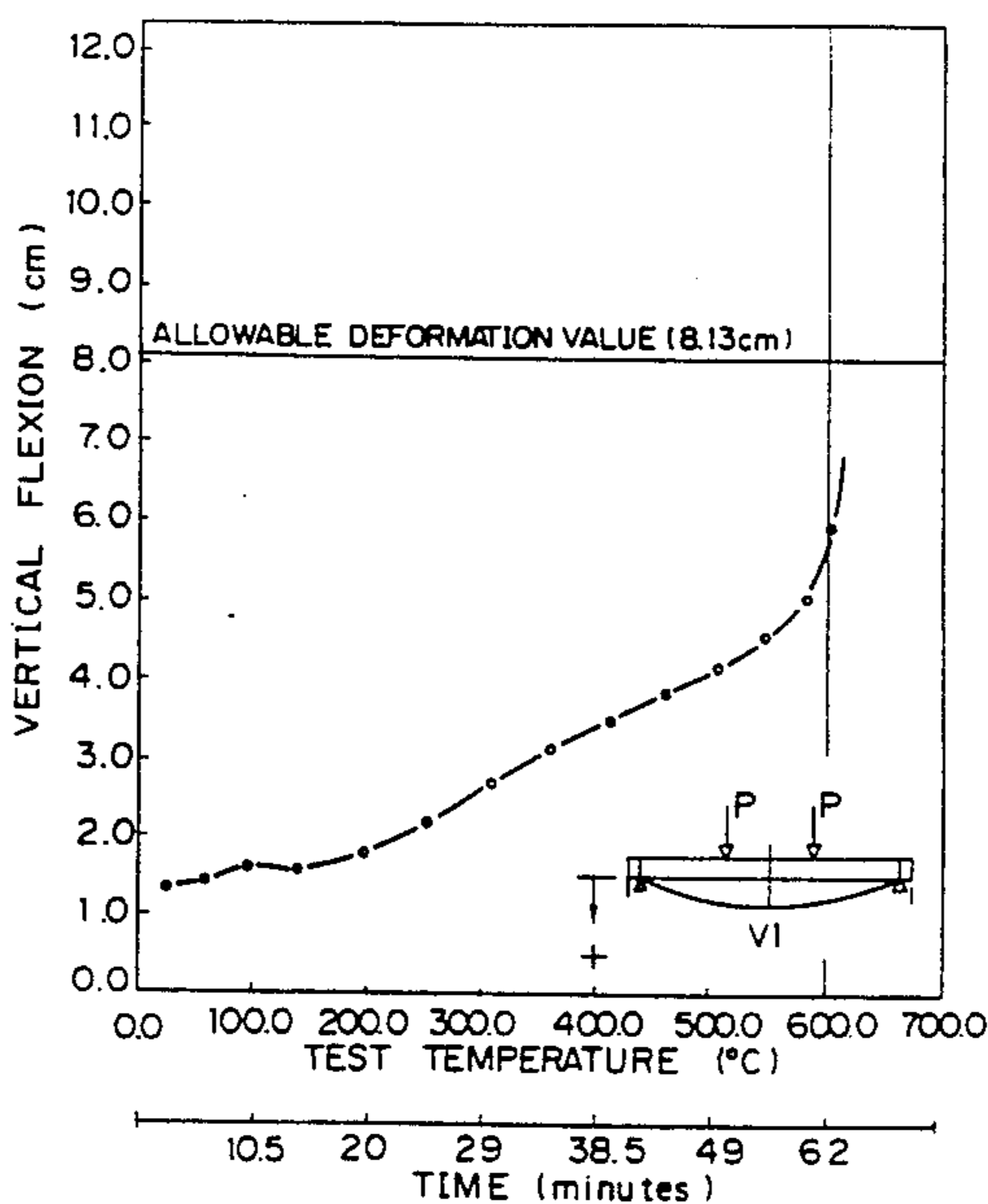
DEFORMATION QUANTITY ( COATING THICKNESS : 10 mm )
