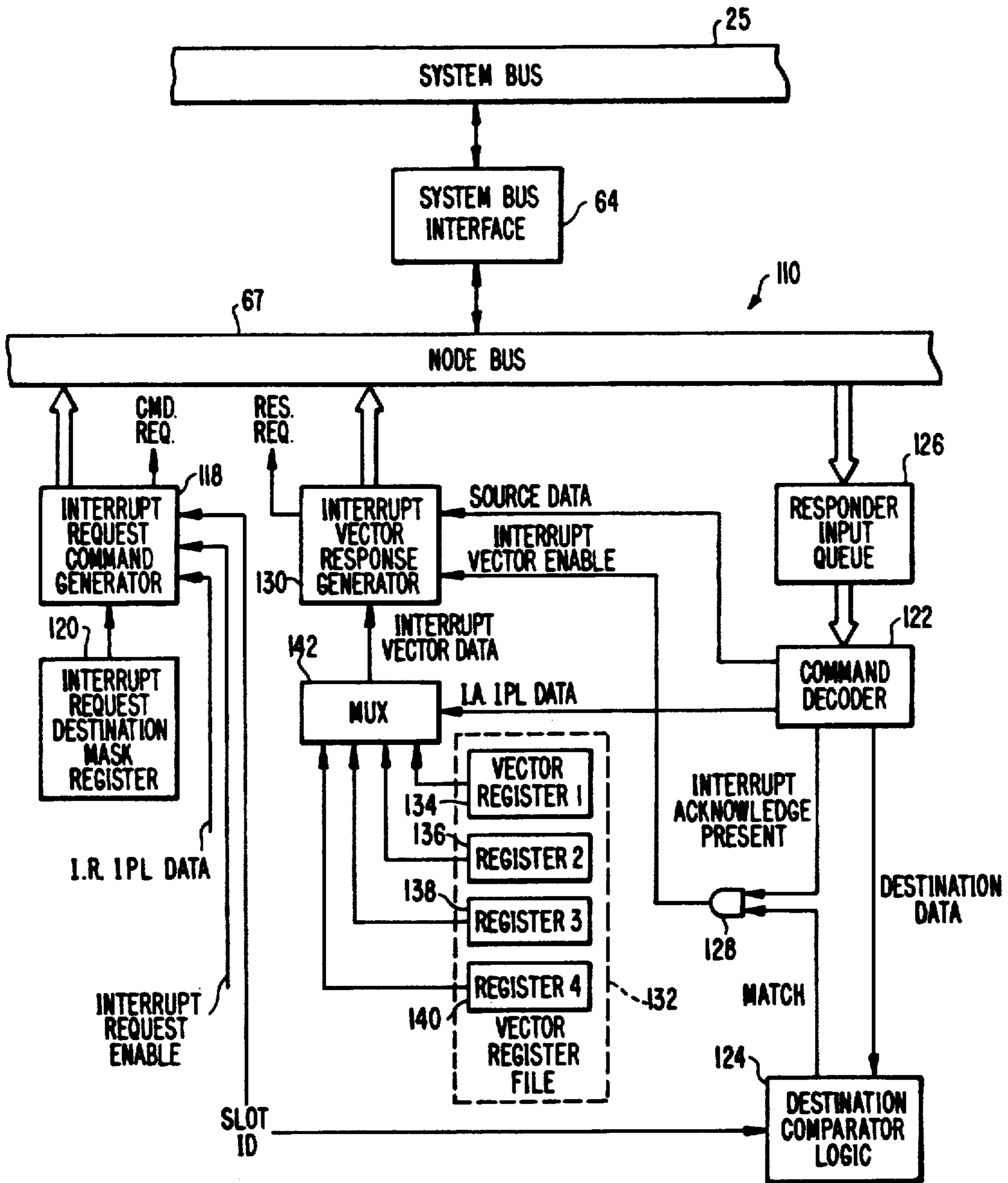
FIG. 6. INTERRUPTING NODE
