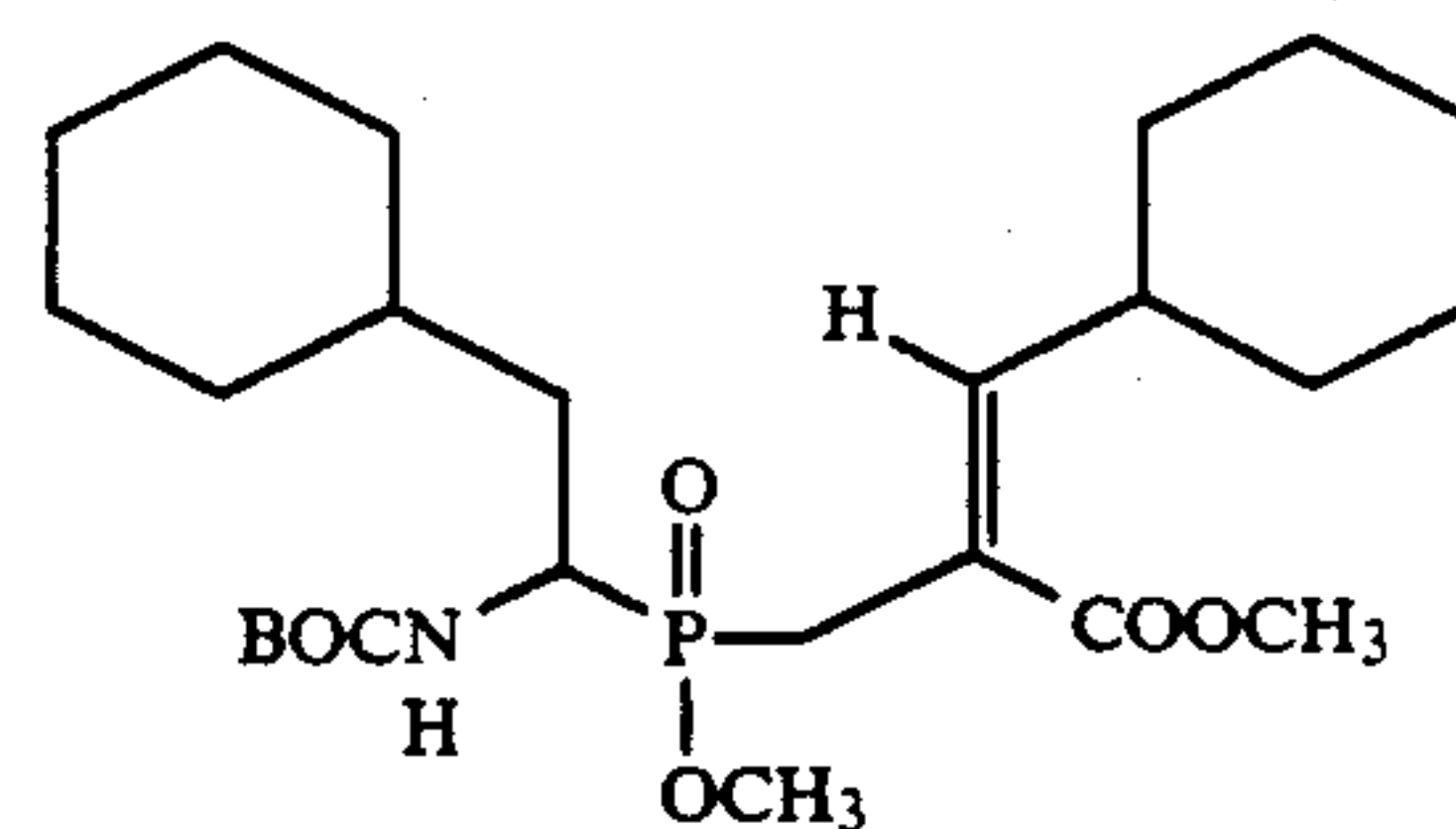
E isomer
