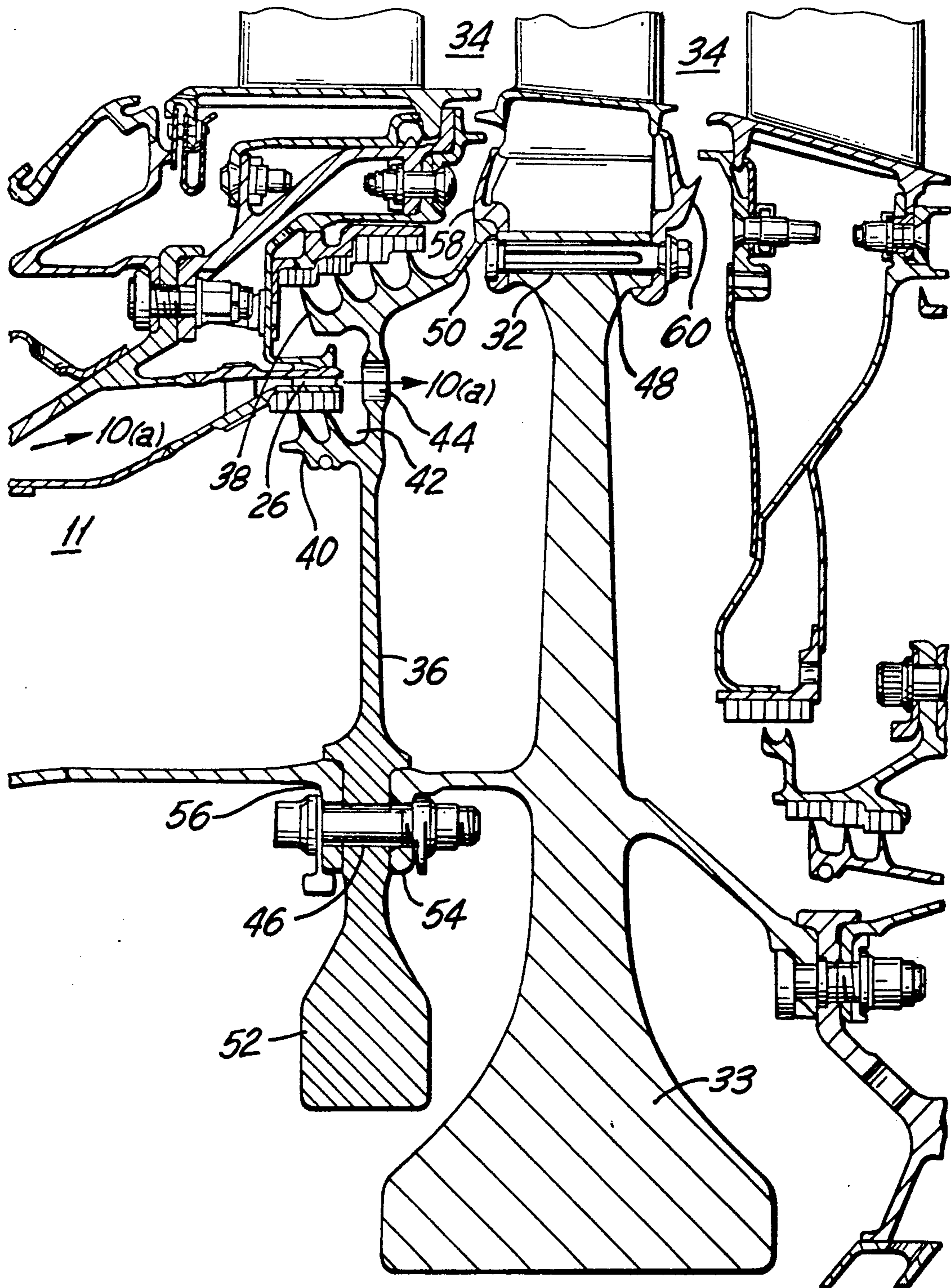
FIG. 2 (PRIOR ART)
