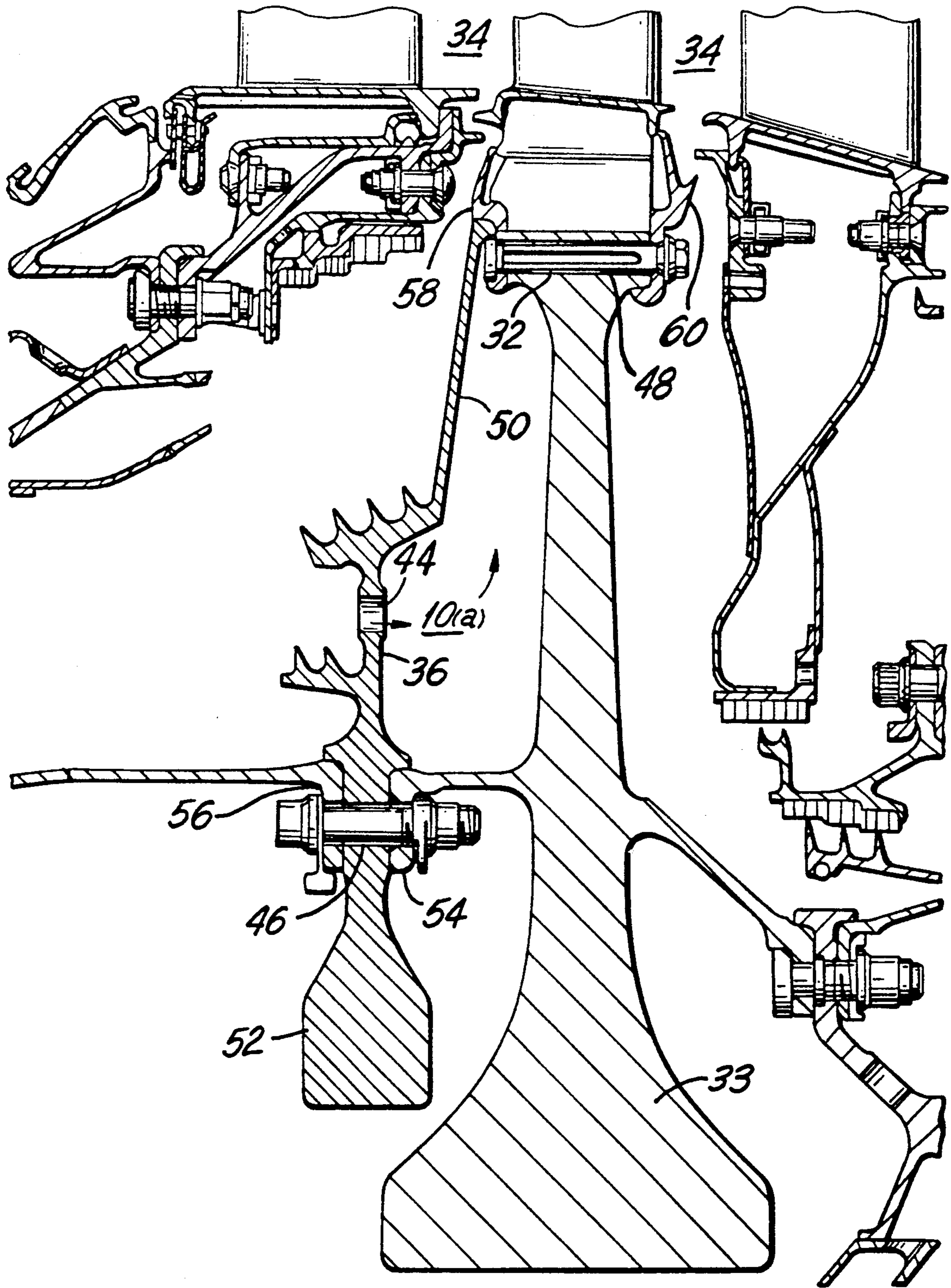
FIG. 3 (PRIOR ART)
