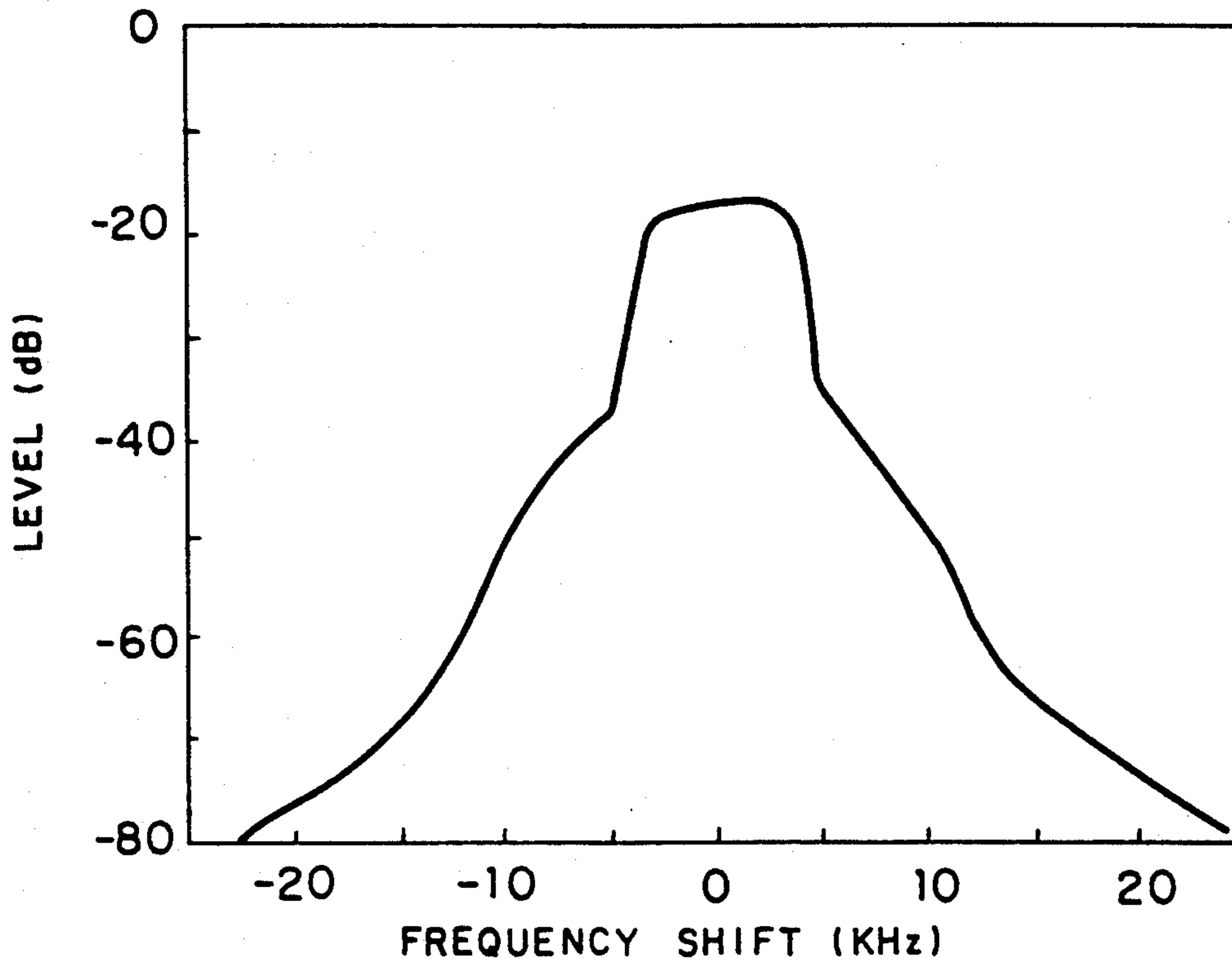
FIG. 4 (PRIOR ART)
