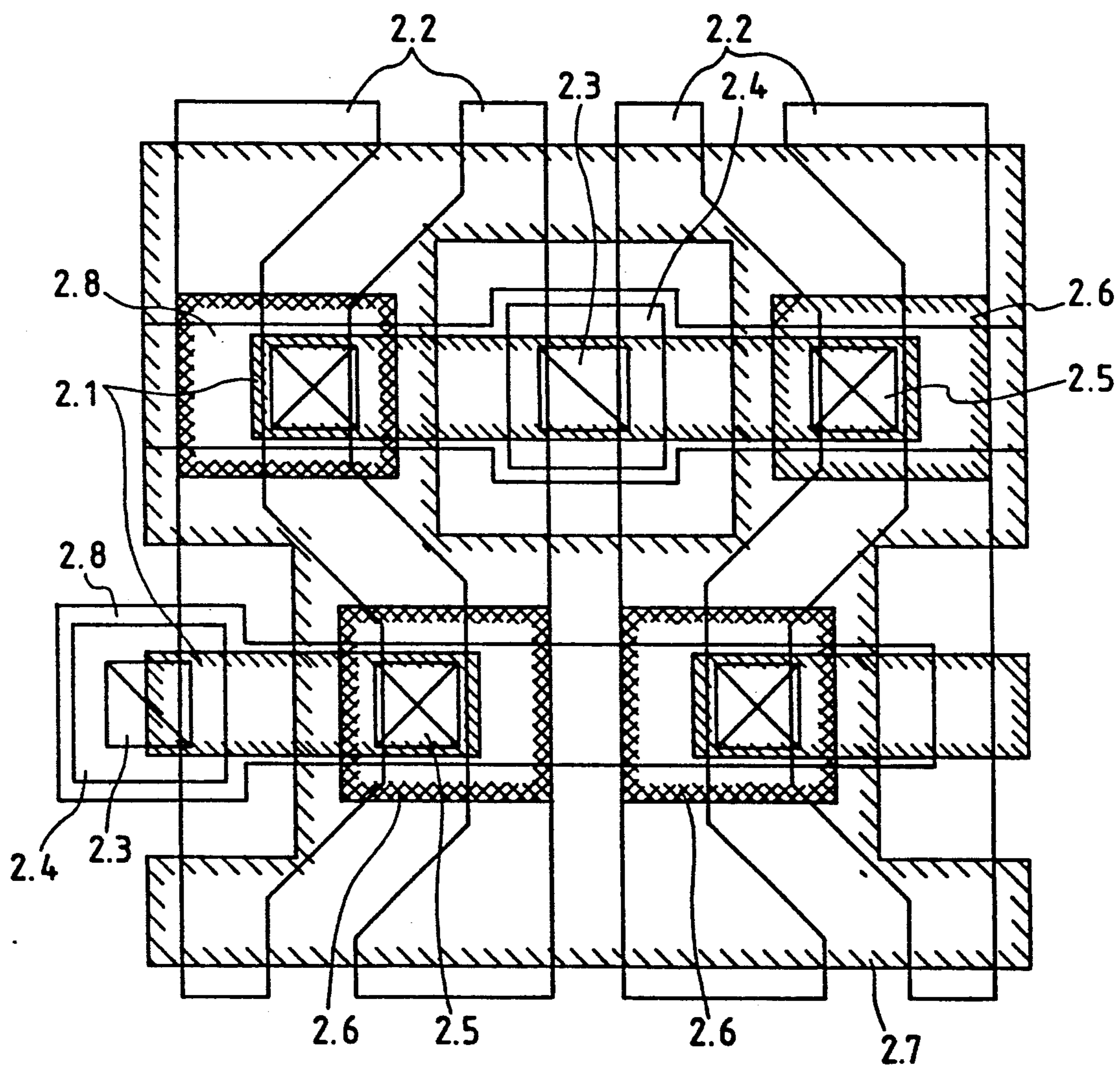
FIG. 2 PRIOR ART
